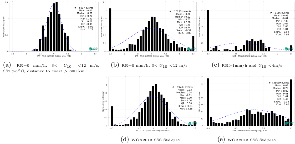
Figure 15: Normalized histogram of \Delta\text{SSS} (SMOS SSS L3 Arctic v2 - 9 Days (CATDS-CEC-LOCEAN) - TSG (GOSUD-Sailing-ship)) for 5 different subdatasets corresponding to: RR=0 mm/h, 3 < U_{10} < 12 m/s, SST >5^{\circ}\text{C} , distance to coast > 800 km (a), RR=0 mm/h, 3 < U_{10} < 12 m/s (b), RR >1 mm/h and U_{10} < 4 m/s (c), WOA2013 SSS Std <0.2 (d), WOA2013 SSS Std >0.2 (e).
