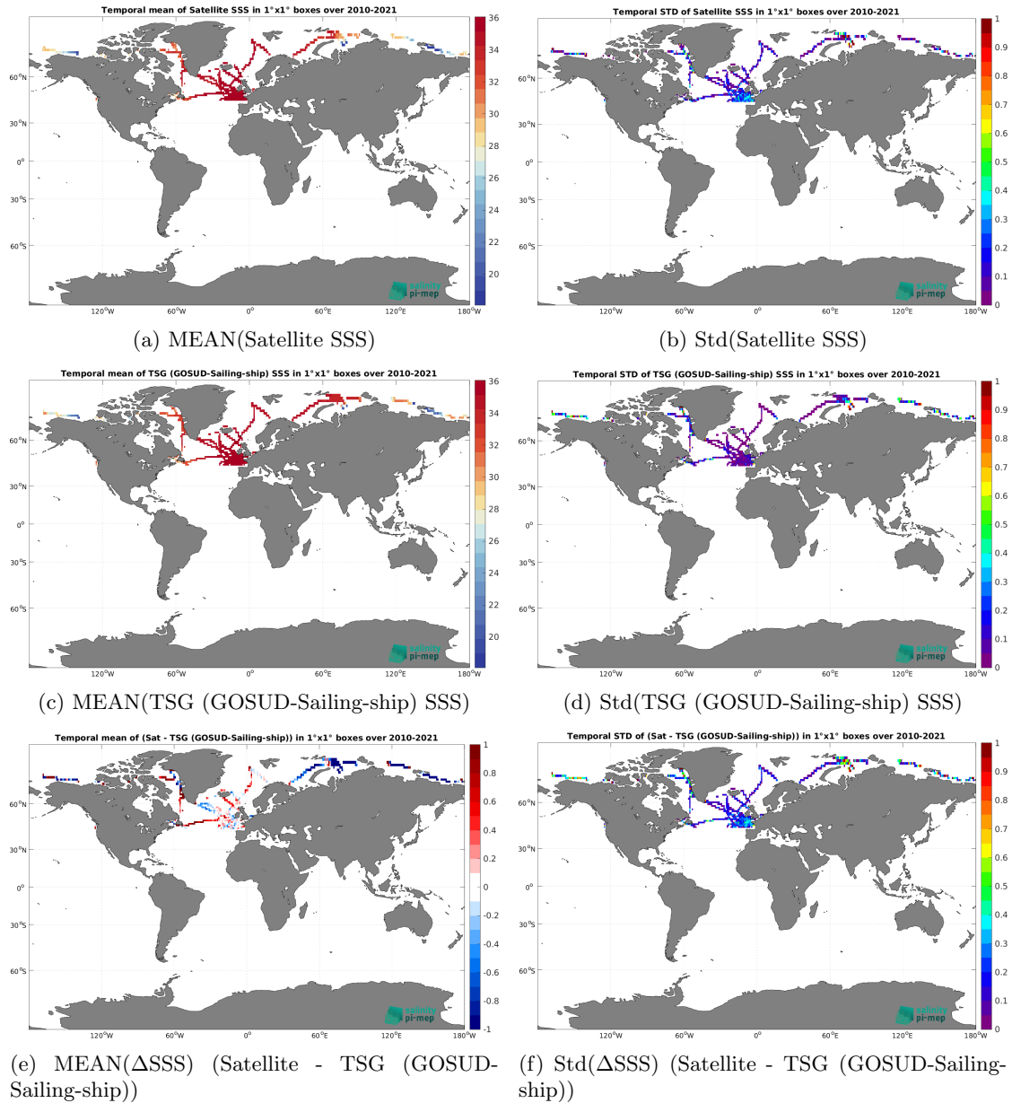
Figure 7: Temporal mean (left) and Std (right) of SSS from SMOS SSS L3 Arctic v2 - 9 Days (CATDS-CEC-LOCEAN) (top), TSG (GOSUD-Sailing-ship) (middle), and of \Delta SSS (Satellite - TSG (GOSUD-Sailing-ship)). Only match-up pairs are used to generate these maps.
