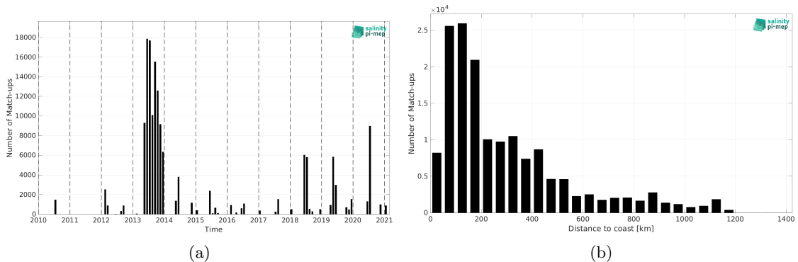
Figure 2: Number of match-ups between TSG (GOSUD-Sailing-ship) and SMOS SSS L3 Arctic v2 - 9 Days (CATDS-CEC-LOCEAN) SSS as a function of time (a) and as function of the distance to coast (b) over the Global Ocean Pi-MEP region and for the full satellite product period.
