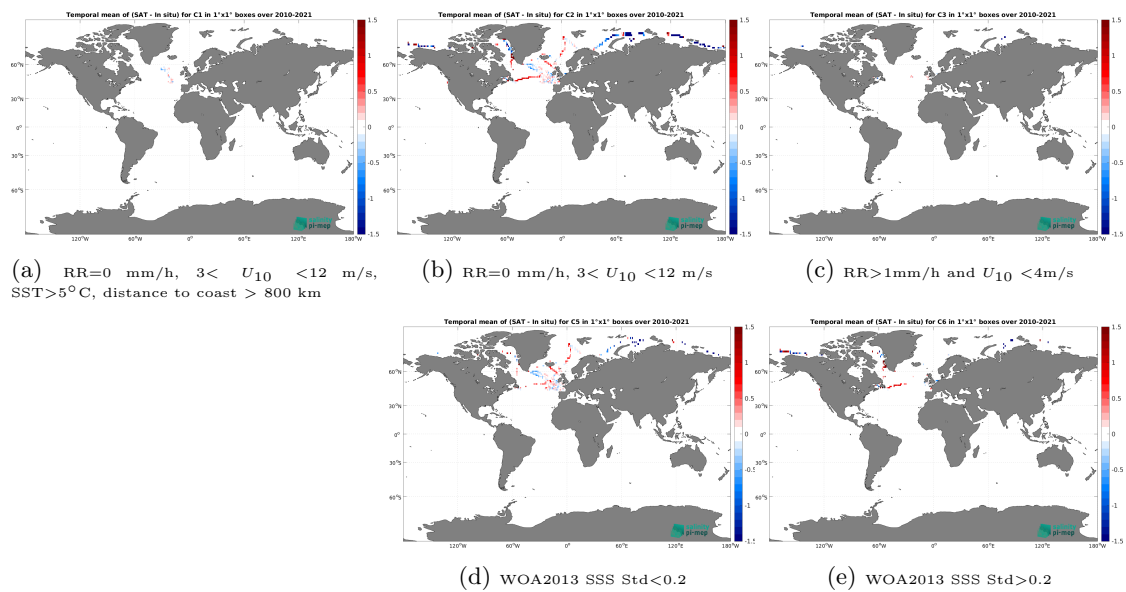
Figure 14: Temporal mean gridded over spatial boxes of size 1^\circ \times 1^\circ of \Delta SSS (SMOS SSS L3 Arctic v2 - 9 Days (CATDS-CEC-LOCEAN) - TSG (GOSUD-Sailing-ship)) for 5 different subdatasets corresponding to:RR=0 mm/h, 3 < U_{10} < 12 m/s, SST > 5^\circ\text{C} , distance to coast > 800 km (a), RR=0 mm/h, 3 < U_{10} < 12 m/s (b), RR > 1 mm/h and U_{10} < 4 m/s (c), WOA2013 SSS Std < 0.2 (d), WOA2013 SSS Std > 0.2 (e).
