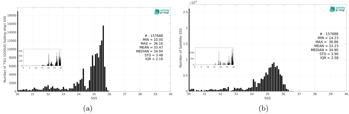
Figure 3: Histograms of SSS from TSG (GOSUD-Sailing-ship) (a) and SMOS SSS L3 Arctic v2 - 9 Days (CATDS-CEC-LOCEAN) (b) considering all match-up pairs per bins of 0.1 over the Global Ocean Pi-MEP region and for the full satellite product period.
