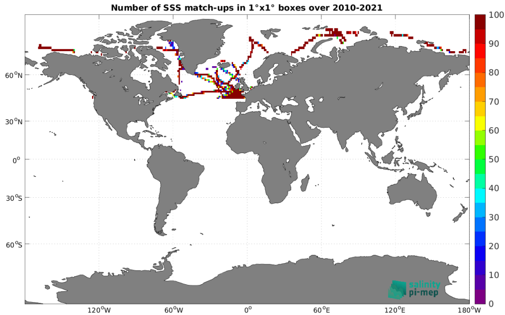
Figure 5: Number of SSS match-ups between TSG (GOSUD-Sailing-ship) SSS and the SMOS SSS L3 Arctic v2 - 9 Days (CATDS-CEC-LOCEAN) SSS product for the Global Ocean Pi-MEP region over 1^\circ \times 1^\circ boxes and for the full satellite product period.
