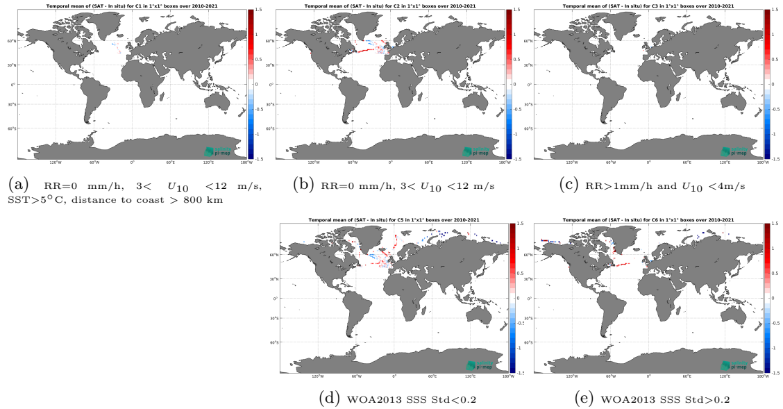
Figure 12: Temporal mean gridded over spatial boxes of size 1^{\circ}\times 1^{\circ} of \Delta SSS (SMOS SSS L3 Arctic v2 - 9 Days (CATDS-CEC-LOCEAN) - TSG (GOSUD-Sailing-ship)) for 5 different subdatasets corresponding to:RR=0 mm/h, 3 < U_{10} < 12 m/s, SST >5^{\circ}\text{C} , distance to coast > 800 km (a), RR=0 mm/h, 3 < U_{10} < 12 m/s (b), RR >1 mm/h and U_{10} < 4 m/s (c), WOA2013 SSS Std <0.2 (d), WOA2013 SSS Std >0.2 (e).
