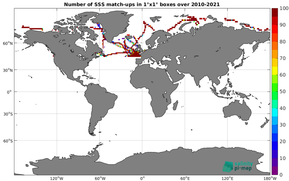
Figure 4: Number of SSS match-ups between TSG (GOSUD-Sailing-ship) SSS and the SMOS SSS L3 Arctic v2 - 9 Days (CATDS-CEC-LOCEAN) SSS product for the Global Ocean Pi-MEP region over 1^\circ \times 1^\circ boxes and for the full satellite product period.
