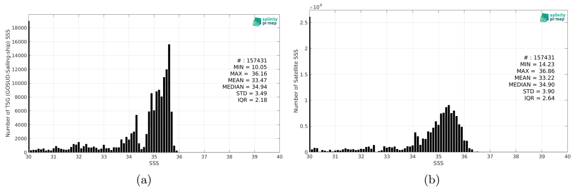
Figure 2: Histograms of SSS from TSG (GOSUD-Sailing-ship) (a) and SMOS SSS L3 Arctic v2 - 9 Days (CATDS-CEC-LOCEAN) (b) considering all match-up pairs per bins of 0.1 over the Global Ocean Pi-MEP region and for the full satellite product period.
