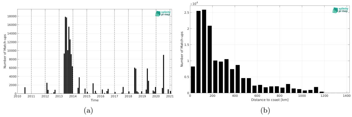
Figure 1: Number of match-ups between TSG (GOSUD-Sailing-ship) and SMOS SSS L3 Arctic v2 - 9 Days (CATDS-CEC-LOCEAN) SSS as a function of time (a) and as function of the distance to coast (b) over the Global Ocean Pi-MEP region and for the full satellite product period.
