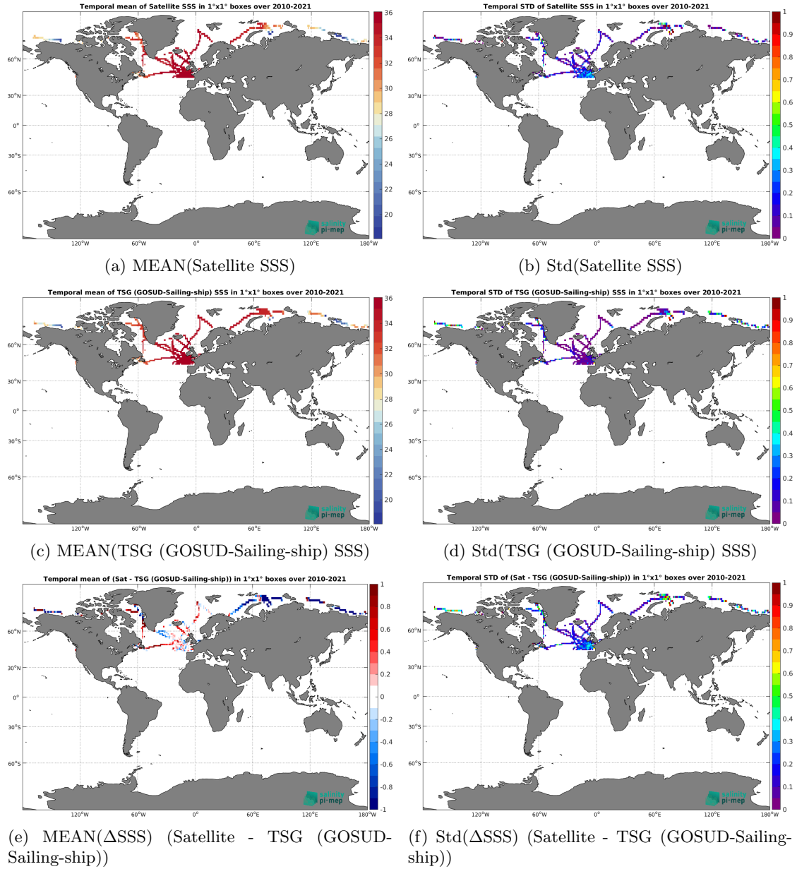
Figure 6: Temporal mean (left) and Std (right) of SSS from SMOS SSS L3 Arctic v2 - 9 Days (CATDS-CEC-LOCEAN) (top), TSG (GOSUD-Sailing-ship) (middle), and of \Delta SSS (Satellite - TSG (GOSUD-Sailing-ship)). Only match-up pairs are used to generate these maps.
