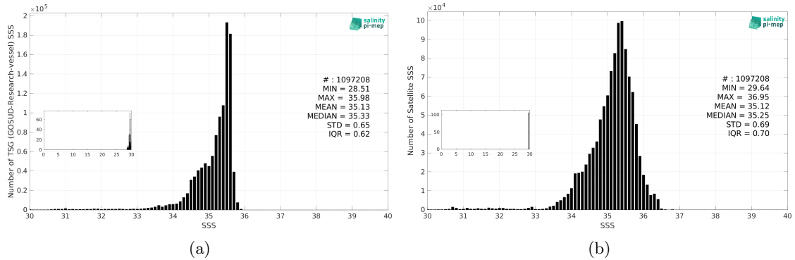
Figure 3: Histograms of SSS from TSG (GOSUD-Research-vessel) (a) and SMOS SSS L3 Arctic v2 - 9 Days (CATDS-CEC-LOCEAN) (b) considering all match-up pairs per bins of 0.1 over the Global Ocean Pi-MEP region and for the full satellite product period.
