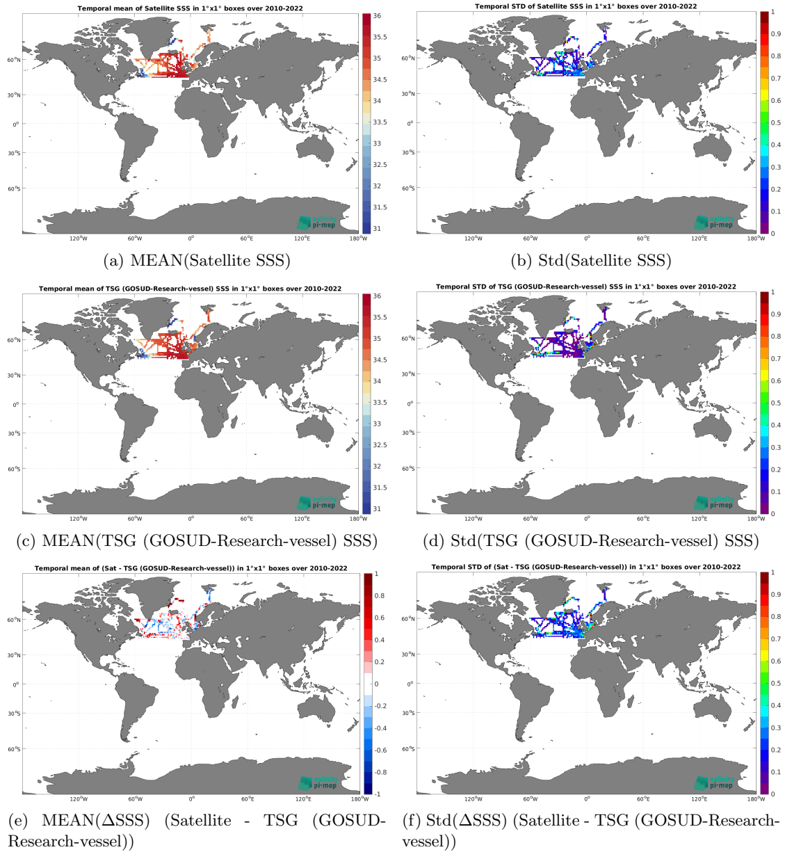
Figure 7: Temporal mean (left) and Std (right) of SSS from SMOS SSS L3 Arctic v2 - 9 Days (CATDS-CEC-LOCEAN) (top), TSG (GOSUD-Research-vessel) (middle), and of \Delta SSS (Satellite - TSG (GOSUD-Research-vessel)). Only match-up pairs are used to generate these maps.
