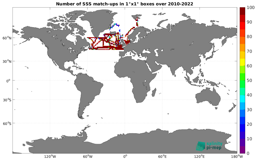
Figure 5: Number of SSS match-ups between TSG (GOSUD-Research-vessel) SSS and the SMOS SSS L3 Arctic v2 - 9 Days (CATDS-CEC-LOCEAN) SSS product for the Global Ocean Pi-MEP region over 1^\circ \times 1^\circ boxes and for the full satellite product period.
