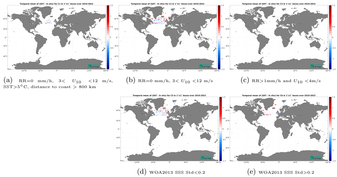
Figure 14: Temporal mean gridded over spatial boxes of size 1^\circ \times 1^\circ of \Delta SSS (SMOS SSS L3 Arctic v2 - 9 Days (CATDS-CEC-LOCEAN) - TSG (GOSUD-Research-vessel)) for 5 different subdatasets corresponding to:RR=0 mm/h, 3 < U_{10} < 12 m/s, SST > 5^\circ\text{C} , distance to coast > 800 km (a), RR=0 mm/h, 3 < U_{10} < 12 m/s (b), RR > 1 mm/h and U_{10} < 4 m/s (c), WOA2013 SSS Std < 0.2 (d), WOA2013 SSS Std > 0.2 (e).
