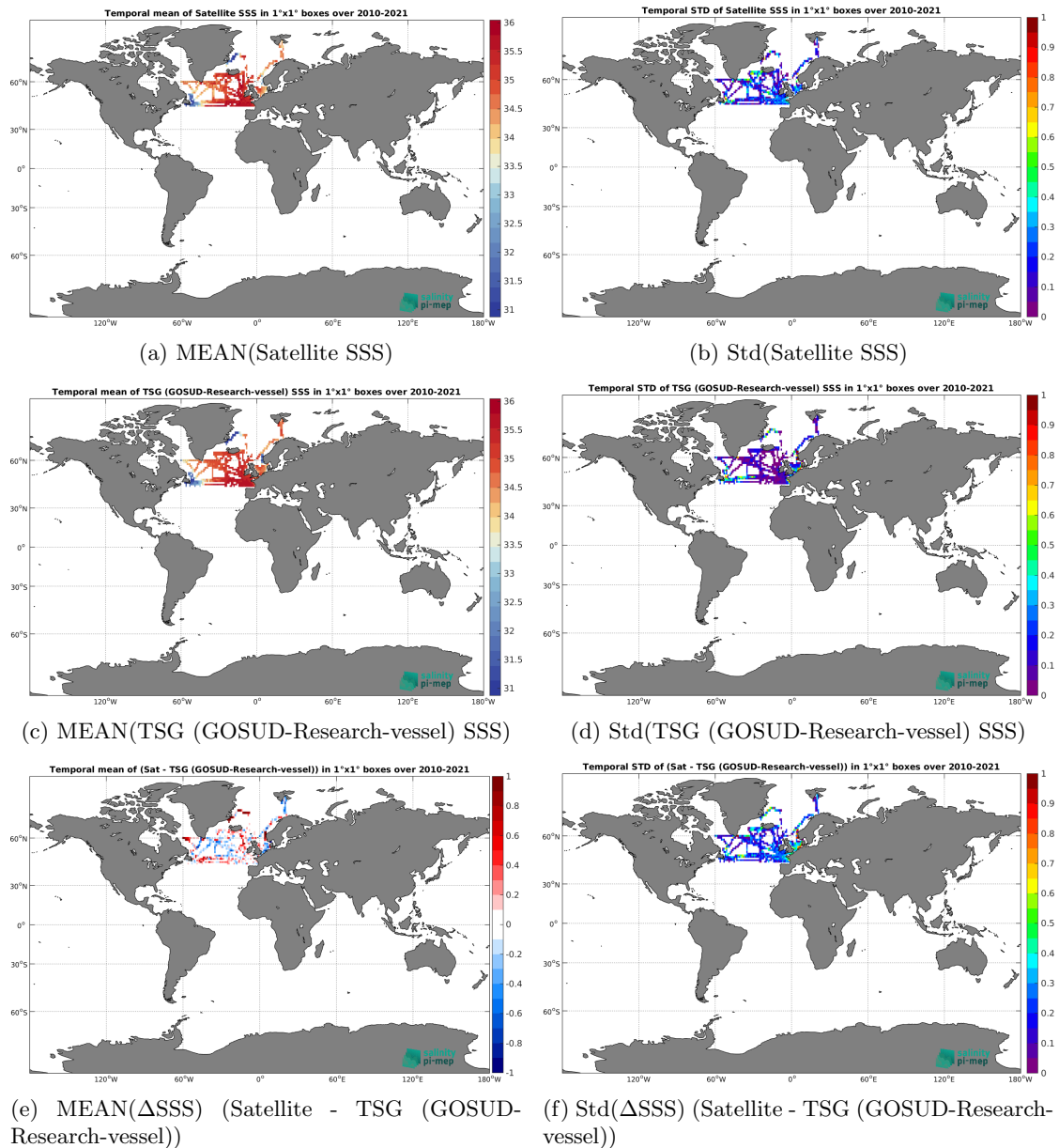
Figure 6: Temporal mean (left) and Std (right) of SSS from SMOS SSS L3 Arctic v2 - 9 Days (CATDS-CEC-LOCEAN) (top), TSG (GOSUD-Research-vessel) (middle), and of \Delta SSS (Satellite - TSG (GOSUD-Research-vessel)). Only match-up pairs are used to generate these maps.
