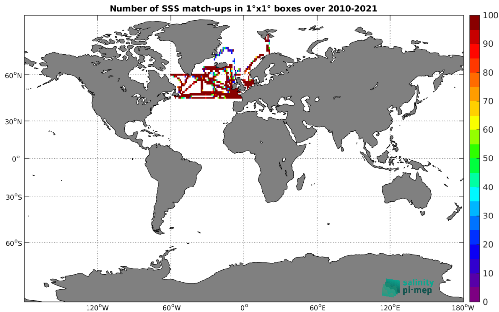
Figure 4: Number of SSS match-ups between TSG (GOSUD-Research-vessel) SSS and the SMOS SSS L3 Arctic v2 - 9 Days (CATDS-CEC-LOCEAN) SSS product for the Global Ocean Pi-MEP region over 1^\circ \times 1^\circ boxes and for the full satellite product period.
