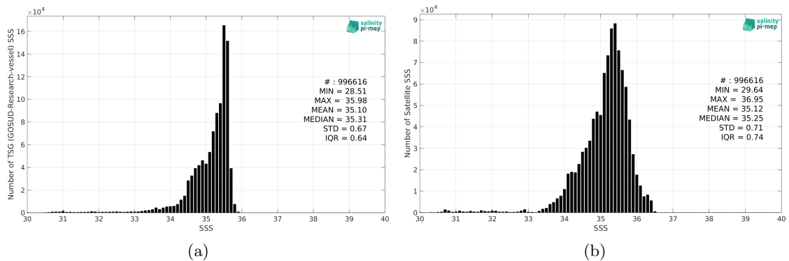
Figure 2: Histograms of SSS from TSG (GOSUD-Research-vessel) (a) and SMOS SSS L3 Arctic v2 - 9 Days (CATDS-CEC-LOCEAN) (b) considering all match-up pairs per bins of 0.1 over the Global Ocean Pi-MEP region and for the full satellite product period.
