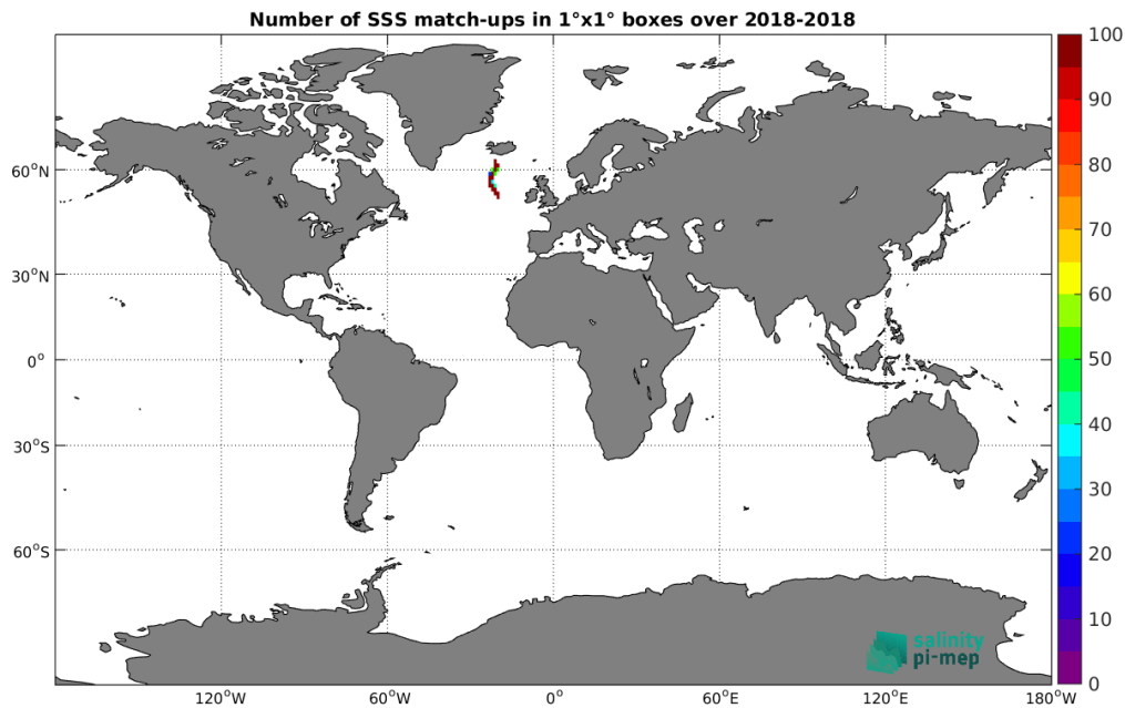
Figure 4: Number of SSS match-ups between TSG (CSIC-UTM) SSS and the SMOS SSS L3 Arctic v2 - 9 Days (CATDS-CEC-LOCEAN) SSS product for the Global Ocean Pi-MEP region over 1^\circ \times 1^\circ boxes and for the full satellite product period.
