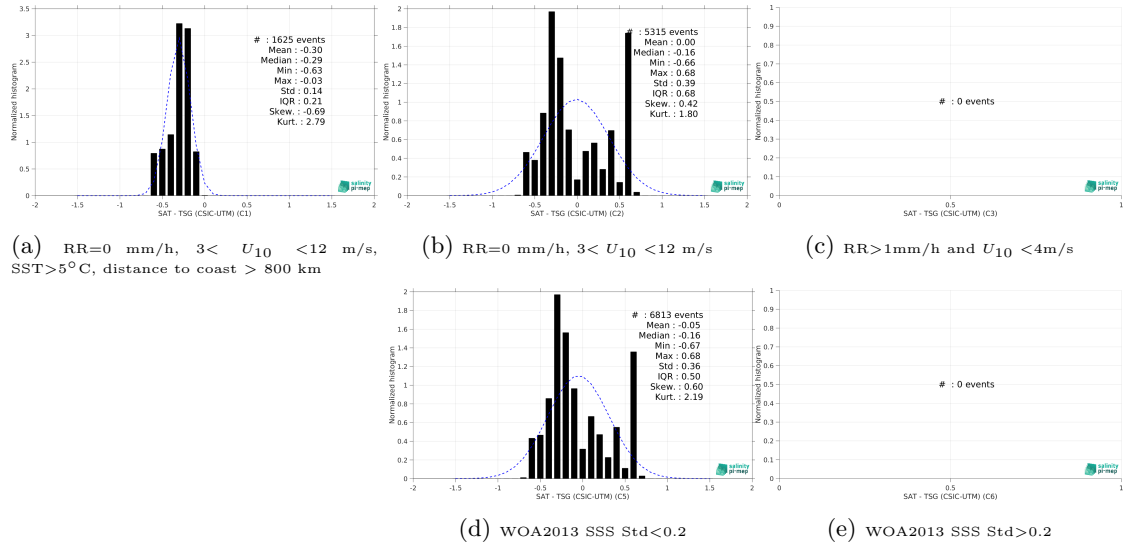
Figure 13: Normalized histogram of \Delta SSS (SMOS SSS L3 Arctic v2 - 9 Days (CATDS-CEC-LOCEAN) - TSG (CSIC-UTM)) for 5 different subdatasets corresponding to: RR=0 mm/h, 3 < U_{10} < 12 m/s, SST > 5°C, distance to coast > 800 km (a), RR=0 mm/h, 3 < U_{10} < 12 m/s (b), RR > 1mm/h and U_{10} < 4 m/s (c), WOA2013 SSS Std < 0.2 (d), WOA2013 SSS Std > 0.2 (e).
