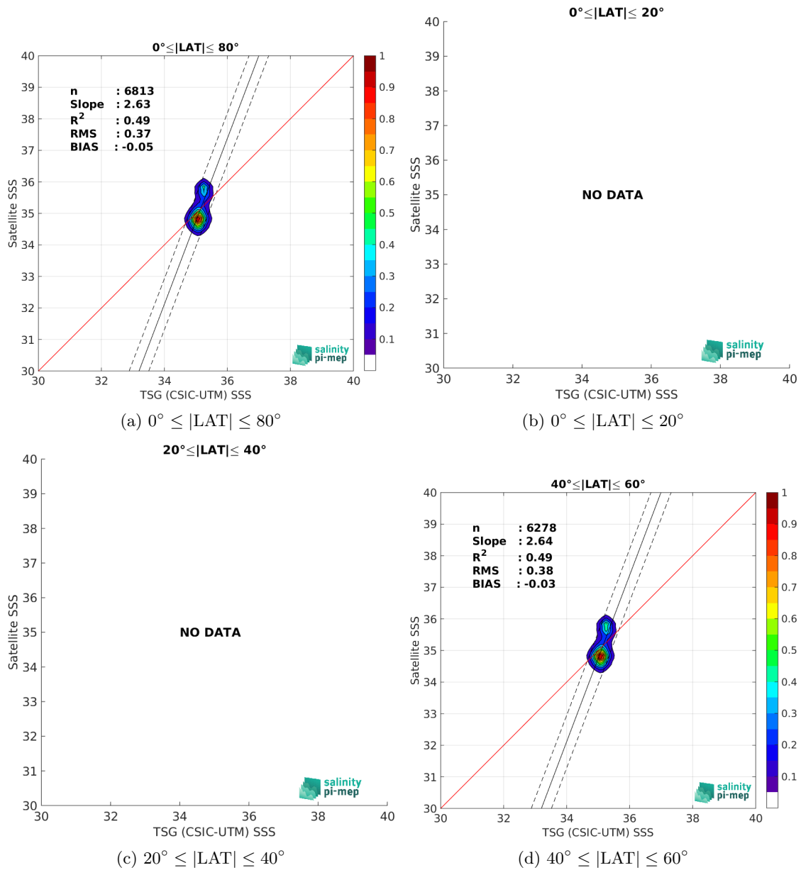
Figure 9: Contour maps of the concentration of SMOS SSS L3 Arctic v2 - 9 Days (CATDS-CEC-LOCEAN) SSS (y-axis) versus TSG (CSIC-UTM) SSS (x-axis) at match-up pairs for different latitude bands. For each plot, the red line shows x=y . The black thin and dashed lines indicate a linear fit through the data cloud and the \pm 95\% confidence levels, respectively. The number match-up pairs n , the slope and R^2 coefficient of the linear fit, the root mean square (RMS) and the mean bias between satellite and in situ data are indicated for each latitude band in each plots.
