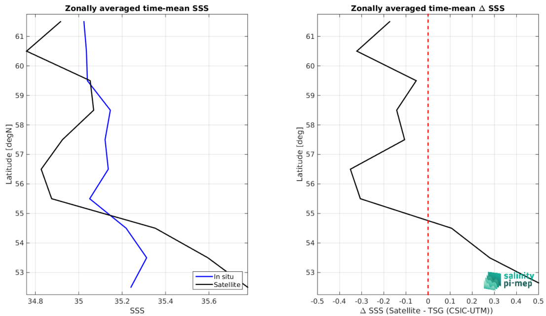
Figure 8: Left panel: Zonal mean SSS from SMOS SSS L3 Arctic v2 - 9 Days (CATDS-CEC-LOCEAN) satellite product (black) and from TSG (CSIC-UTM) (blue). Right panel: Zonal mean of \Delta SSS (Satellite - TSG (CSIC-UTM)) for all the collected Pi-MEP match-up pairs estimated over the full satellite product period.
