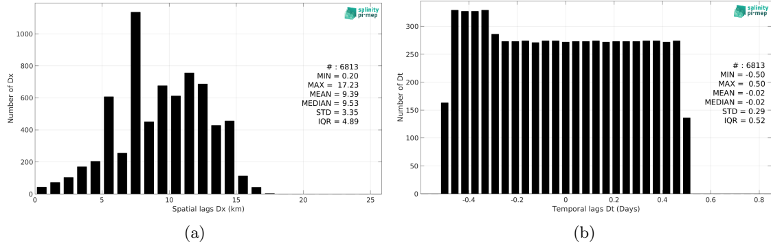
Figure 5: Histograms of the spatial (a) and temporal (b) lags between the location/time of the TSG (CSIC-UTM) measurement and the date of the corresponding SMOS SSS L3 Arctic v2 - 9 Days (CATDS-CEC-LOCEAN) SSS pixel.
