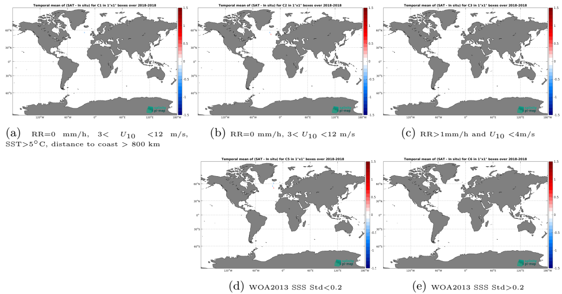
Figure 12: Temporal mean gridded over spatial boxes of size 1^{\circ}\times 1^{\circ} of \Delta\text{SSS} (SMOS SSS L3 Arctic v2 - 9 Days (CATDS-CEC-LOCEAN) - TSG (CSIC-UTM)) for 5 different subdatasets corresponding to:RR=0 mm/h, 3 < U_{10} < 12 m/s, SST >5^{\circ}\text{C} , distance to coast > 800 km (a), RR=0 mm/h, 3 < U_{10} < 12 m/s (b), RR >1 mm/h and U_{10} < 4 m/s (c), WOA2013 SSS Std <0.2 (d), WOA2013 SSS Std >0.2 (e).
