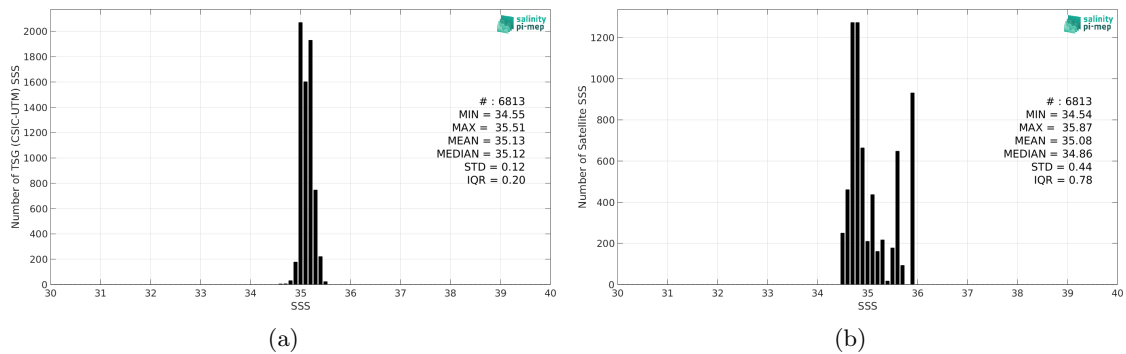
Figure 2: Histograms of SSS from TSG (CSIC-UTM) (a) and SMOS SSS L3 Arctic v2 - 9 Days (CATDS-CEC-LOCEAN) (b) considering all match-up pairs per bins of 0.1 over the Global Ocean Pi-MEP region and for the full satellite product period.
