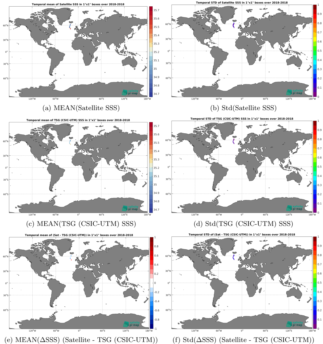
Figure 6: Temporal mean (left) and Std (right) of SSS from SMOS SSS L3 Arctic v2 - 9 Days (CATDS-CEC-LOCEAN) (top), TSG (CSIC-UTM) (middle), and of \Delta SSS (Satellite - TSG (CSIC-UTM)). Only match-up pairs are used to generate these maps.
