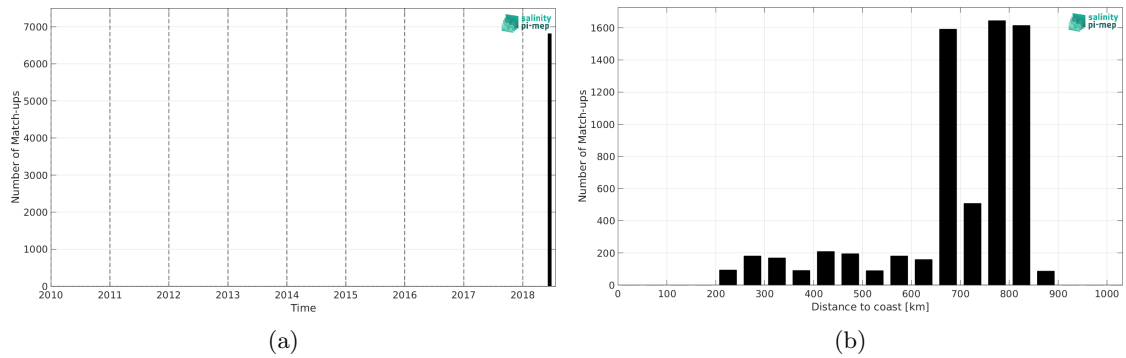
Figure 1: Number of match-ups between TSG (CSIC-UTM) and SMOS SSS L3 Arctic v2 - 9 Days (CATDS-CEC-LOCEAN) SSS as a function of time (a) and as function of the distance to coast (b) over the Global Ocean Pi-MEP region and for the full satellite product period.
