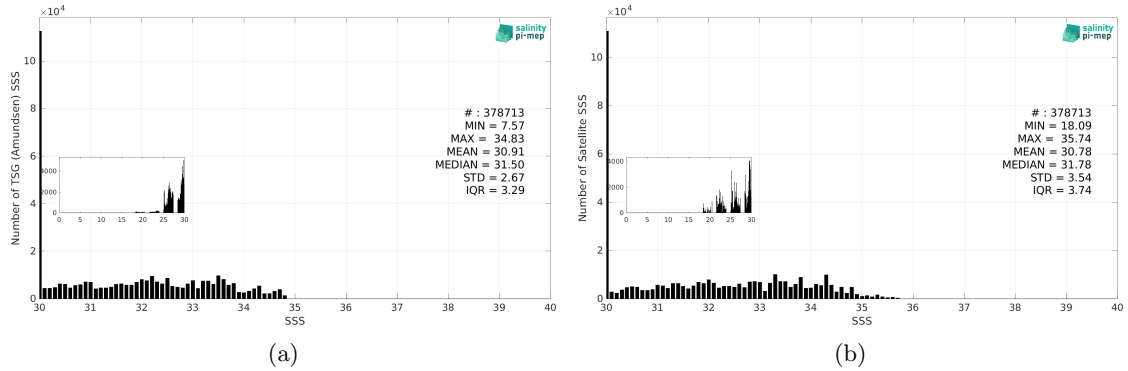
Figure 3: Histograms of SSS from TSG (Amundsen) (a) and SMOS SSS L3 Arctic v2 - 9 Days (CATDS-CEC-LOCEAN) (b) considering all match-up pairs per bins of 0.1 over the Global Ocean Pi-MEP region and for the full satellite product period.
