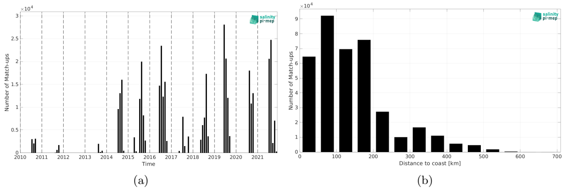
Figure 2: Number of match-ups between TSG (Amundsen) and SMOS SSS L3 Arctic v2 - 9 Days (CATDS-CEC-LOCEAN) SSS as a function of time (a) and as function of the distance to coast (b) over the Global Ocean Pi-MEP region and for the full satellite product period.
