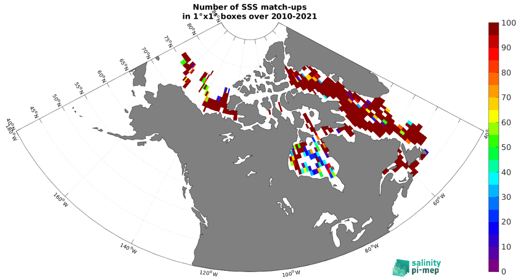
Figure 5: Number of SSS match-ups between TSG (Amundsen) SSS and the SMOS SSS L3 Arctic v2 - 9 Days (CATDS-CEC-LOCEAN) SSS product for the Global Ocean Pi-MEP region over 1°×1° boxes and for the full satellite product period.
