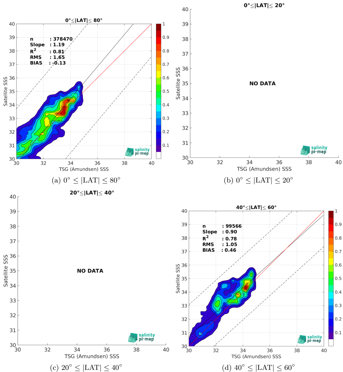
Figure 9: Contour maps of the concentration of SMOS SSS L3 Arctic v2 - 9 Days (CATDS-CEC-LOCEAN) SSS (y-axis) versus TSG (Amundsen) SSS (x-axis) at match-up pairs for different latitude bands. For each plot, the red line shows x=y . The black thin and dashed lines indicate a linear fit through the data cloud and the \pm 95\% confidence levels, respectively. The number match-up pairs n , the slope and R^2 coefficient of the linear fit, the root mean square (RMS) and the mean bias between satellite and in situ data are indicated for each latitude band in each plots.
