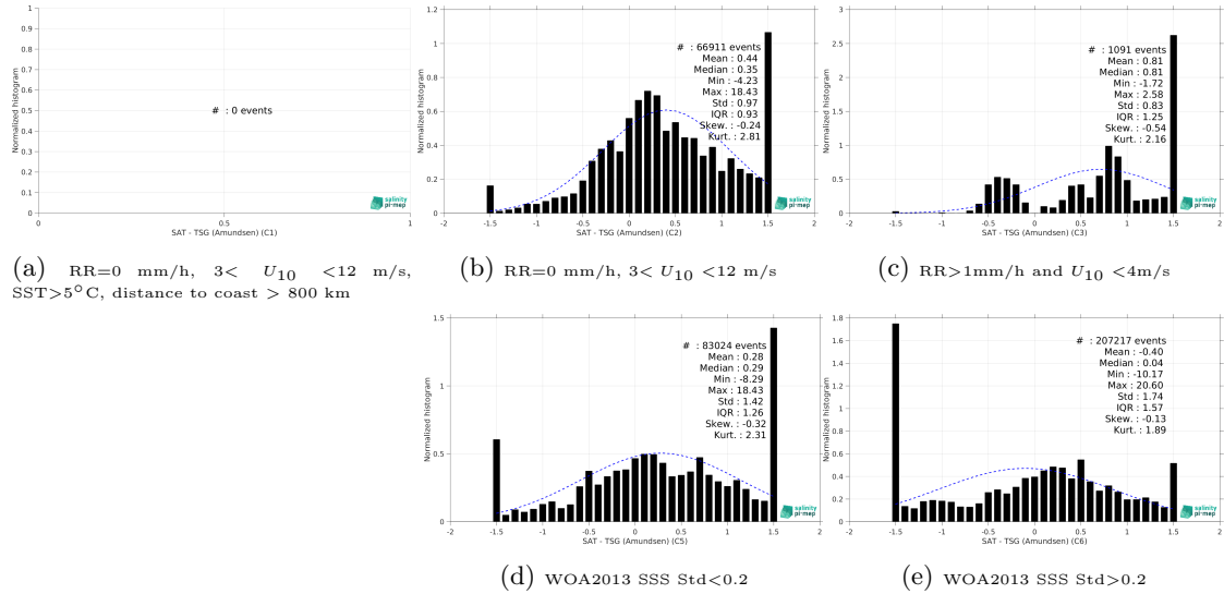
Figure 13: Normalized histogram of \Delta SSS (SMOS SSS L3 Arctic v2 - 9 Days (CATDS-CEC-LOCEAN) - TSG (Amundsen)) for 5 different subdatasets corresponding to: RR=0 mm/h, 3 < U_{10} < 12 m/s, SST>5°C, distance to coast > 800 km (a), RR=0 mm/h, 3 < U_{10} < 12 m/s (b), RR>1mm/h and U_{10} < 4 m/s (c), WOA2013 SSS Std<0.2 (d), WOA2013 SSS Std>0.2 (e).
