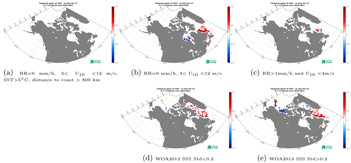
Figure 12: Temporal mean gridded over spatial boxes of size 1^{\circ}\times 1^{\circ} of \Delta\text{SSS} (SMOS SSS L3 Arctic v2 - 9 Days (CATDS-CEC-LOCEAN) - TSG (Amundsen)) for 5 different subdatasets corresponding to:RR=0 mm/h, 3 < U_{10} < 12 m/s, SST >5^{\circ}\text{C} , distance to coast > 800 km (a), RR=0 mm/h, 3 < U_{10} < 12 m/s (b), RR >1 mm/h and U_{10} < 4 m/s (c), WOA2013 SSS Std <0.2 (d), WOA2013 SSS Std >0.2 (e).
