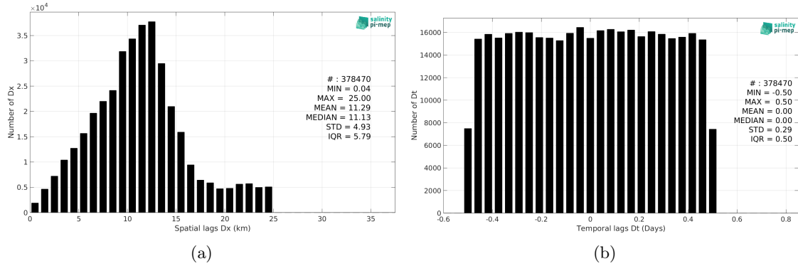
Figure 5: Histograms of the spatial (a) and temporal (b) lags between the location/time of the TSG (Amundsen) measurement and the date of the corresponding SMOS SSS L3 Arctic v2 - 9 Days (CATDS-CEC-LOCEAN) SSS pixel.
