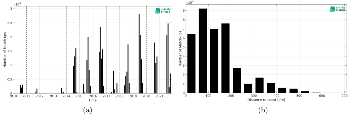
Figure 1: Number of match-ups between TSG (Amundsen) and SMOS SSS L3 Arctic v2 - 9 Days (CATDS-CEC-LOCEAN) SSS as a function of time (a) and as function of the distance to coast (b) over the Global Ocean Pi-MEP region and for the full satellite product period.
