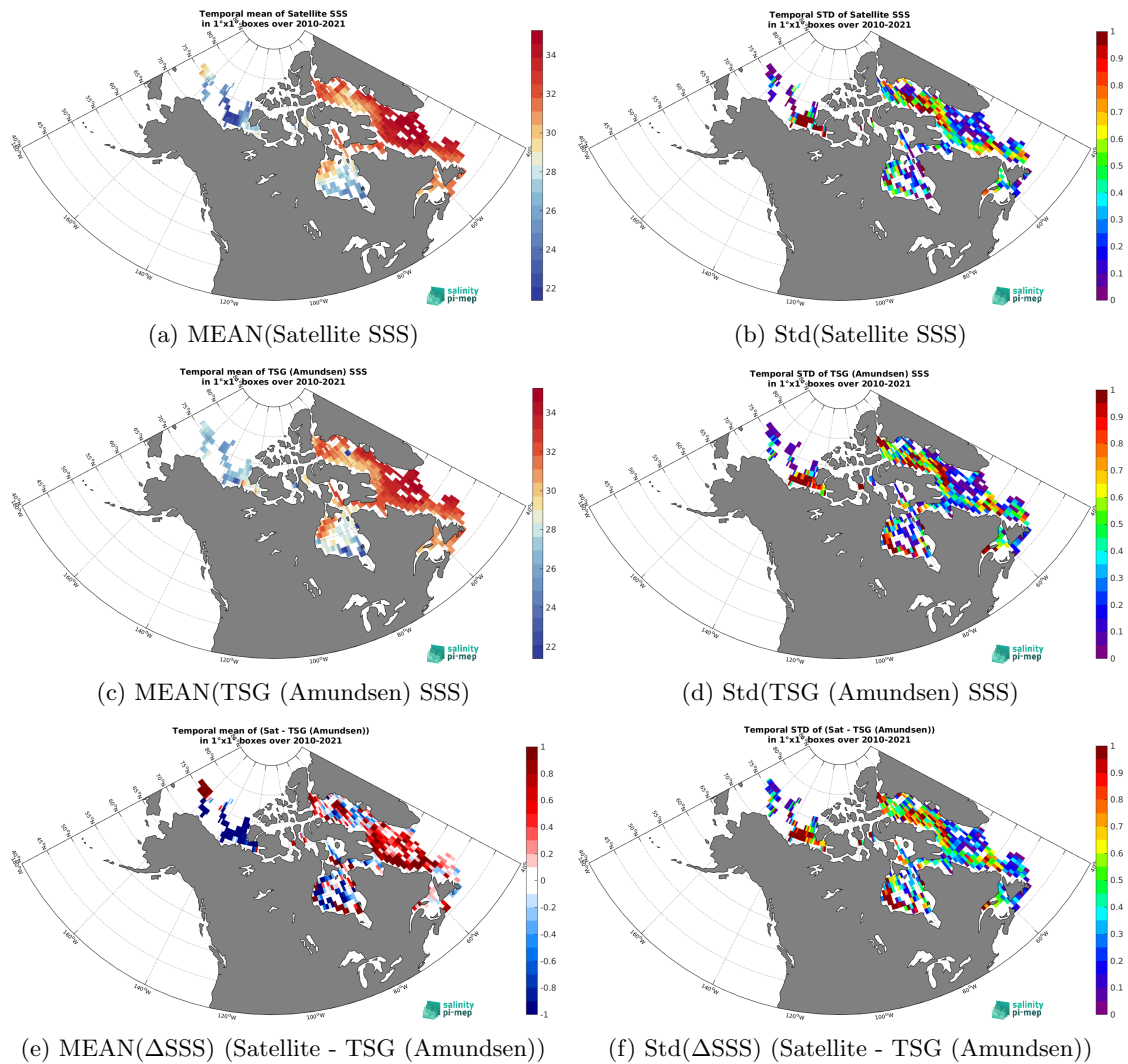
Figure 6: Temporal mean (left) and Std (right) of SSS from SMOS SSS L3 Arctic v2 - 9 Days (CATDS-CEC-LOCEAN) (top), TSG (Amundsen) (middle), and of \Delta SSS (Satellite - TSG (Amundsen)). Only match-up pairs are used to generate these maps.
