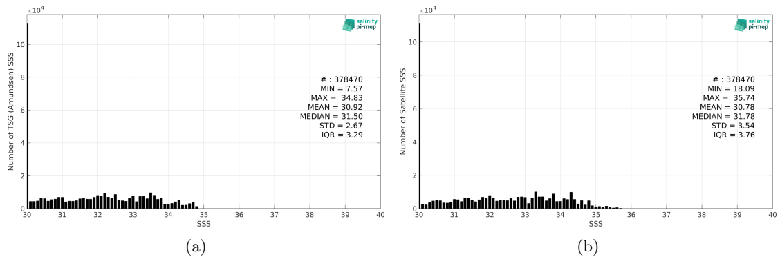
Figure 2: Histograms of SSS from TSG (Amundsen) (a) and SMOS SSS L3 Arctic v2 - 9 Days (CATDS-CEC-LOCEAN) (b) considering all match-up pairs per bins of 0.1 over the Global Ocean Pi-MEP region and for the full satellite product period.
