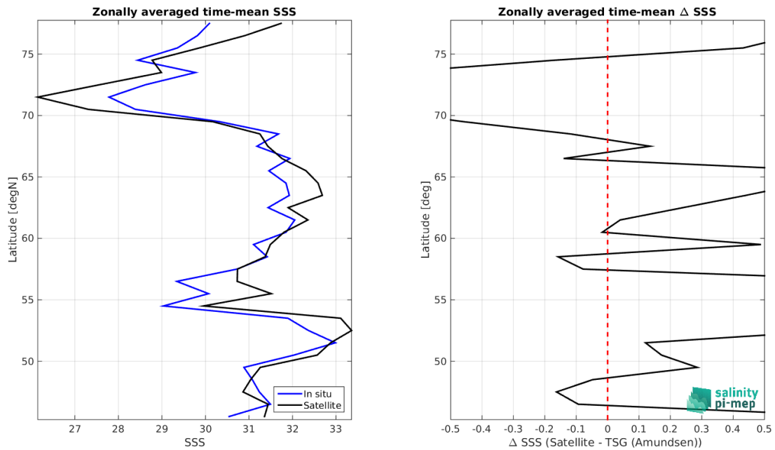
Figure 8: Left panel: Zonal mean SSS from SMOS SSS L3 Arctic v2 - 9 Days (CATDS-CEC-LOCEAN) satellite product (black) and from TSG (Amundsen) (blue). Right panel: Zonal mean of \Delta SSS (Satellite - TSG (Amundsen)) for all the collected Pi-MEP match-up pairs estimated over the full satellite product period.
