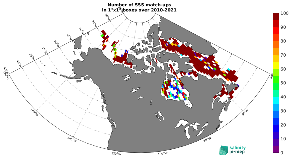
Figure 4: Number of SSS match-ups between TSG (Amundsen) SSS and the SMOS SSS L3 Arctic v2 - 9 Days (CATDS-CEC-LOCEAN) SSS product for the Global Ocean Pi-MEP region over 1^\circ \times 1^\circ boxes and for the full satellite product period.
