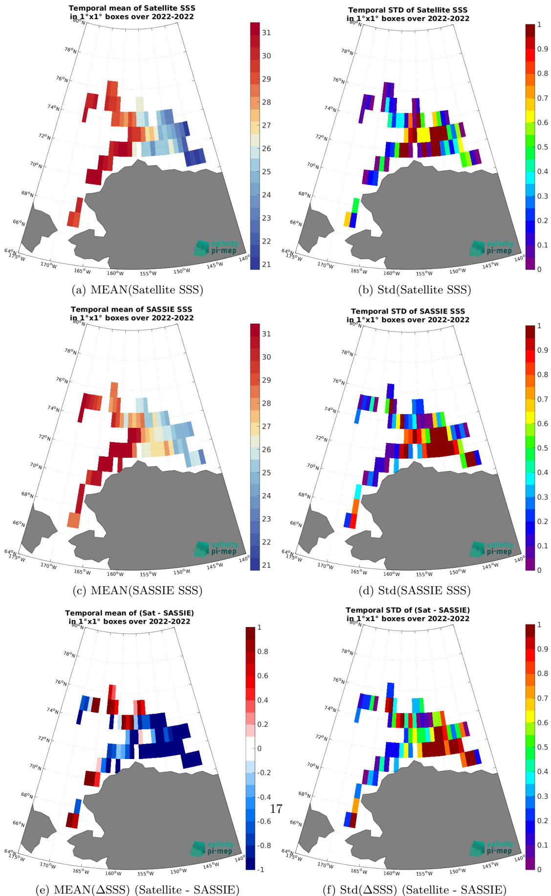
Figure 7: Temporal mean (left) and Std (right) of SSS from SMOS SSS L3 Arctic v2 - 9 Days (CATDS-CEC-LOCEAN) (top), SASSIE (middle), and of \Delta SSS (Satellite - SASSIE). Only match-up pairs are used to generate these maps.
