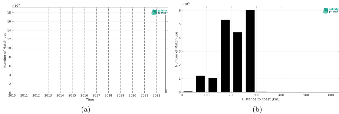
Figure 2: Number of match-ups between SASSIE and SMOS SSS L3 Arctic v2 - 9 Days (CATDS-CEC-LOCEAN) SSS as a function of time (a) and as function of the distance to coast (b) over the Global Ocean Pi-MEP region and for the full satellite product period.
