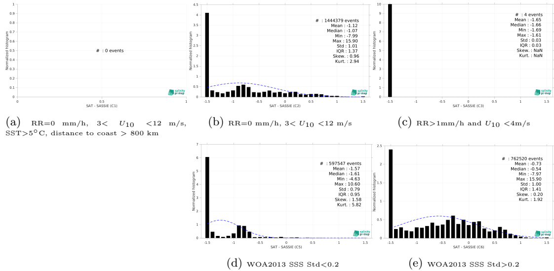
Figure 15: Normalized histogram of \Delta SSS (SMOS SSS L3 Arctic v2 - 9 Days (CATDS-CEC-LOCEAN) - SASSIE) for 5 different subdatasets corresponding to: RR=0 mm/h, 3 < U_{10} < 12 m/s, SST>5°C, distance to coast > 800 km (a), RR=0 mm/h, 3 < U_{10} < 12 m/s (b), RR>1mm/h and U_{10} < 4 m/s (c), WOA2013 SSS Std<0.2 (d), WOA2013 SSS Std>0.2 (e).
