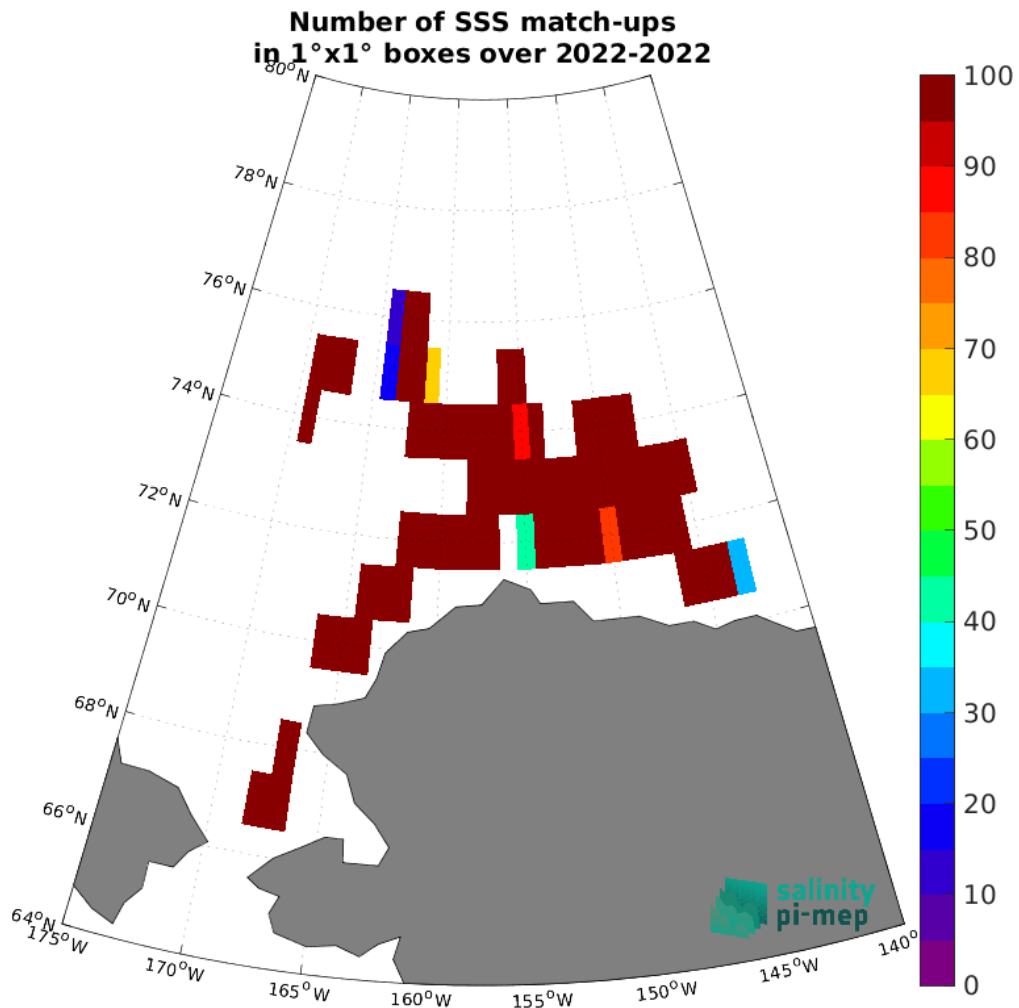
Figure 5: Number of SSS match-ups between SASSIE SSS and the SMOS SSS L3 Arctic v2 - 9 Days (CATDS-CEC-LOCEAN) SSS product for the Global Ocean Pi-MEP region over 1^\circ \times 1^\circ boxes and for the full satellite product period.
