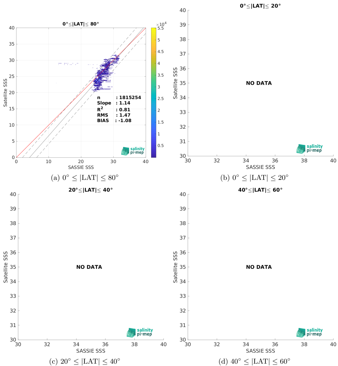
Figure 10: Contour maps of the concentration of SMOS SSS L3 Arctic v2 - 9 Days (CATDS-CEC-LOCEAN) SSS (y-axis) versus SASSIE SSS (x-axis) at match-up pairs for different latitude bands. For each plot, the red line shows x=y . The black thin and dashed lines indicate a linear fit through the data cloud and the \pm 95\% confidence levels, respectively. The number match-up pairs n , the slope and R^2 coefficient of the linear fit, the root mean square (RMS) and the mean bias between satellite and in situ data are indicated for each latitude band in each plots.
