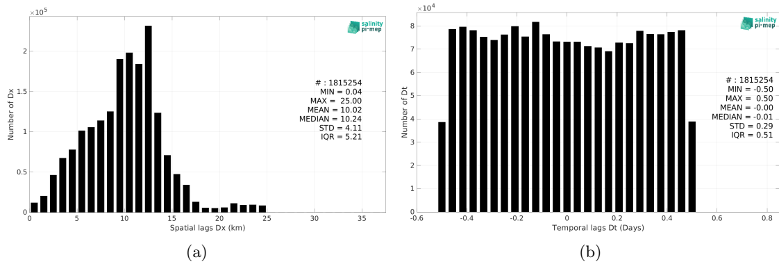
Figure 6: Histograms of the spatial (a) and temporal (b) lags between the location/time of the SASSIE measurement and the date of the corresponding SMOS SSS L3 Arctic v2 - 9 Days (CATDS-CEC-LOCEAN) SSS pixel.
