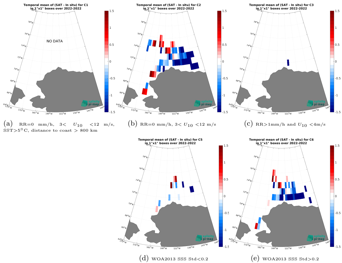
Figure 14: Temporal mean gridded over spatial boxes of size 1^\circ \times 1^\circ of \Delta\text{SSS} (SMOS SSS L3 Arctic v2 - 9 Days (CATDS-CEC-LOCEAN) - SASSIE) for 5 different subdatasets corresponding to:RR=0 mm/h, 3 < U_{10} < 12 m/s, SST>5°C, distance to coast > 800 km (a), RR=0 mm/h, 3 < U_{10} < 12 m/s (b), RR>1mm/h and U_{10} < 4 m/s (c), WOA2013 SSS Std<0.2 (d), WOA2013 SSS Std>0.2 (e).
