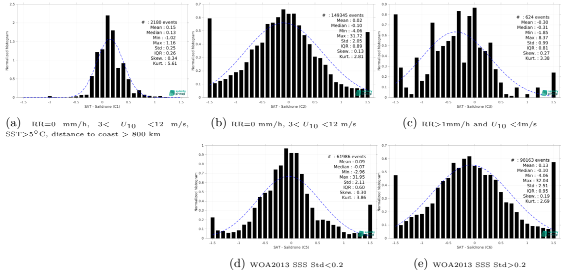
Figure 15: Normalized histogram of \Delta SSS (SMOS SSS L3 Arctic v2 - 9 Days (CATDS-CEC-LOCEAN) - Saildrone) for 5 different subdatasets corresponding to: RR=0 mm/h, 3 < U_{10} < 12 m/s, SST > 5°C, distance to coast > 800 km (a), RR=0 mm/h, 3 < U_{10} < 12 m/s (b), RR > 1mm/h and U_{10} < 4 m/s (c), WOA2013 SSS Std < 0.2 (d), WOA2013 SSS Std > 0.2 (e).
