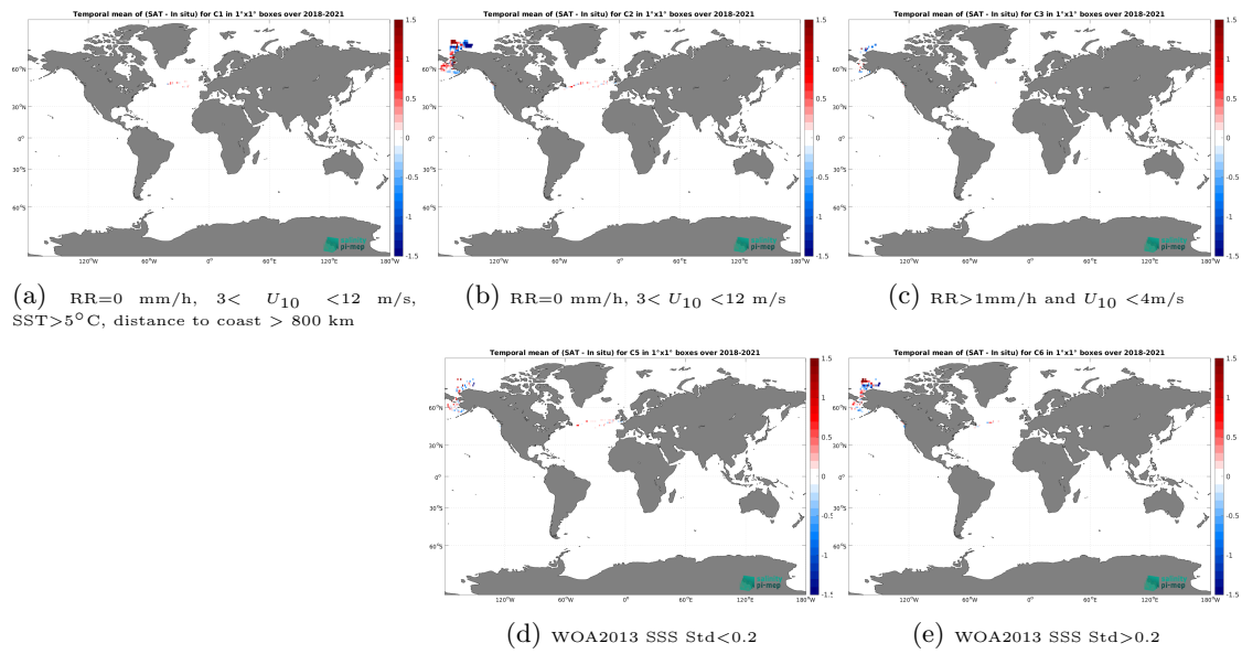
Figure 14: Temporal mean gridded over spatial boxes of size 1^\circ \times 1^\circ of \Delta SSS (SMOS SSS L3 Arctic v2 - 9 Days (CATDS-CEC-LOCEAN) - Sairdrone) for 5 different subdatasets corresponding to:RR=0 mm/h, 3 < U_{10} < 12 m/s, SST > 5^\circ\text{C} , distance to coast > 800 km (a), RR=0 mm/h, 3 < U_{10} < 12 m/s (b), RR > 1 mm/h and U_{10} < 4 m/s (c), WOA2013 SSS Std < 0.2 (d), WOA2013 SSS Std > 0.2 (e).
