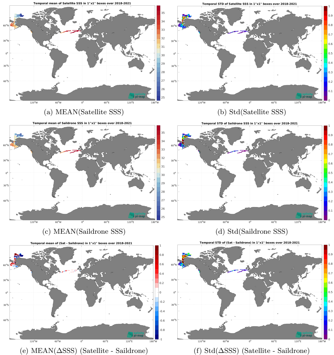
Figure 7: Temporal mean (left) and Std (right) of SSS from SMOS SSS L3 Arctic v2 - 9 Days (CATDS-CEC-LOCEAN) (top), Saildrone (middle), and of \Delta SSS (Satellite - Saildrone). Only match-up pairs are used to generate these maps.
