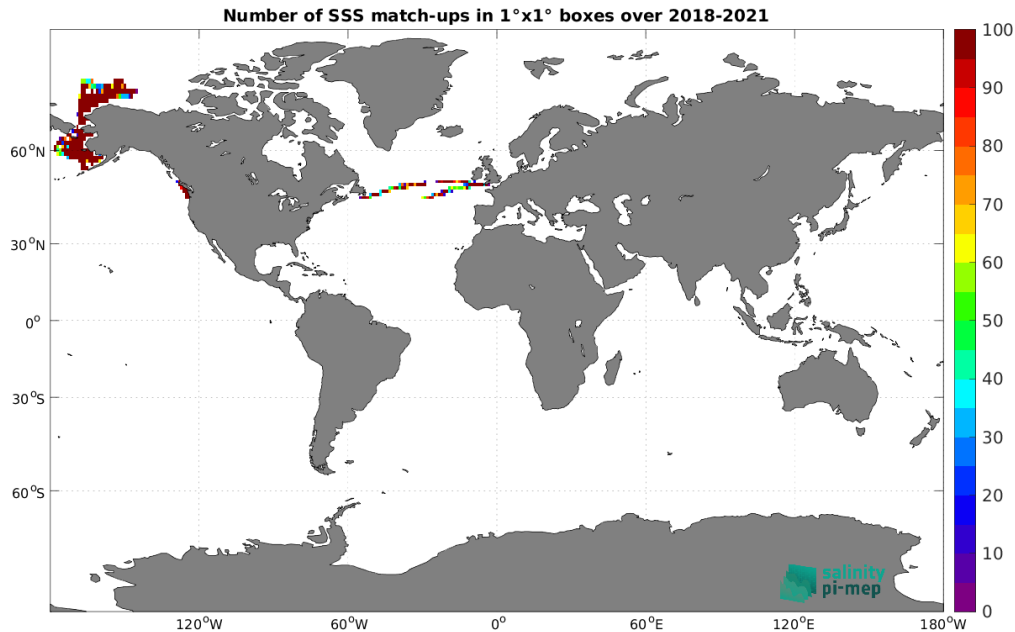
Figure 5: Number of SSS match-ups between Saildrone SSS and the SMOS SSS L3 Arctic v2 - 9 Days (CATDS-CEC-LOCEAN) SSS product for the Global Ocean Pi-MEP region over 1^\circ \times 1^\circ boxes and for the full satellite product period.
