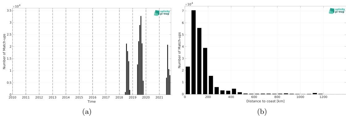
Figure 2: Number of match-ups between Saildrone and SMOS SSS L3 Arctic v2 - 9 Days (CATDS-CEC-LOCEAN) SSS as a function of time (a) and as function of the distance to coast (b) over the Global Ocean Pi-MEP region and for the full satellite product period.
