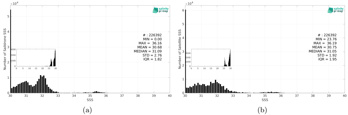
Figure 3: Histograms of SSS from Saildrone (a) and SMOS SSS L3 Arctic v2 - 9 Days (CATDS-CEC-LOCEAN) (b) considering all match-up pairs per bins of 0.1 over the Global Ocean Pi-MEP region and for the full satellite product period.
