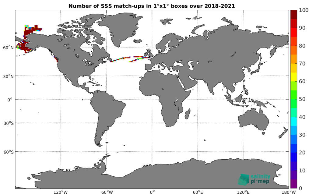
Figure 4: Number of SSS match-ups between Saildrone SSS and the SMOS SSS L3 Arctic v2 - 9 Days (CATDS-CEC-LOCEAN) SSS product for the Global Ocean Pi-MEP region over 1^\circ \times 1^\circ boxes and for the full satellite product period.
