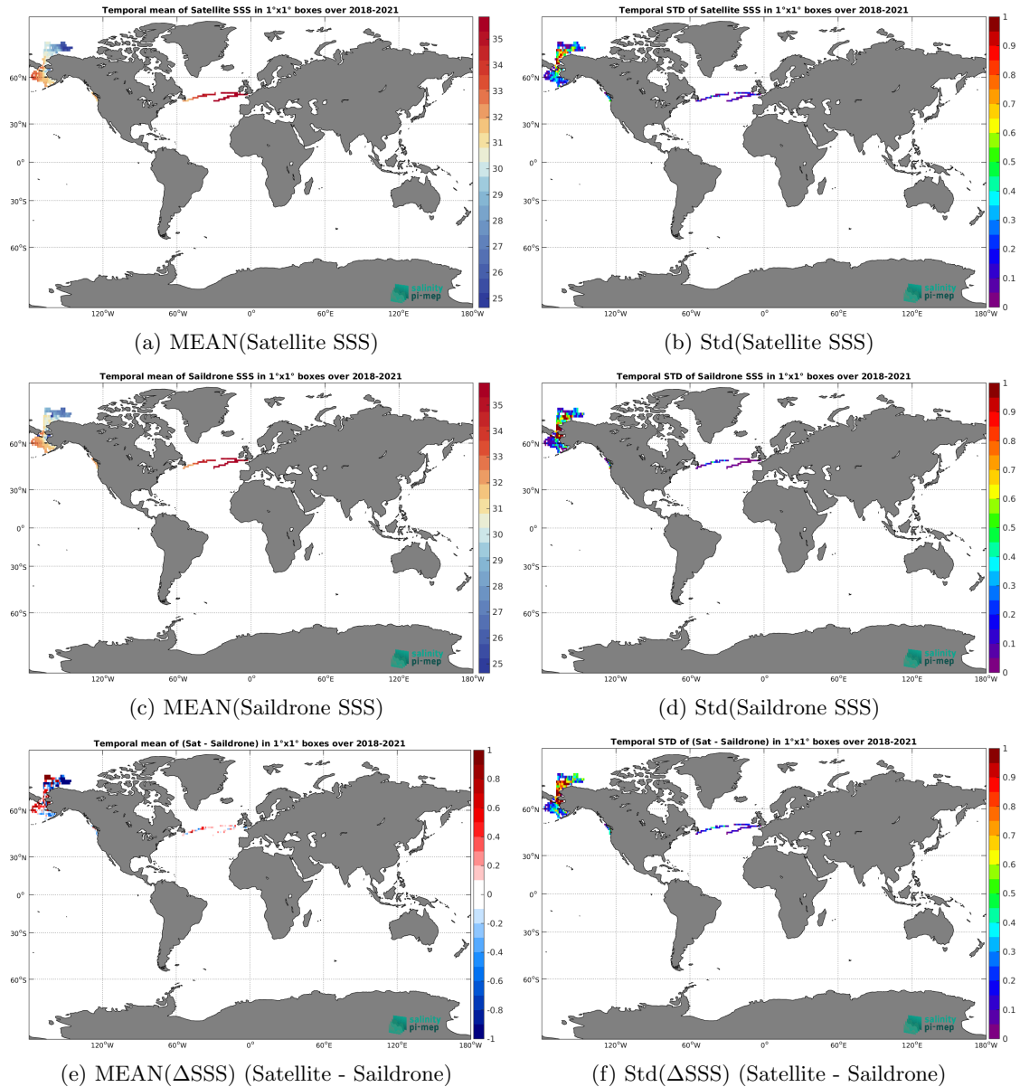
Figure 6: Temporal mean (left) and Std (right) of SSS from SMOS SSS L3 Arctic v2 - 9 Days (CATDS-CEC-LOCEAN) (top), Saildrone (middle), and of \Delta SSS (Satellite - Saildrone). Only match-up pairs are used to generate these maps.
