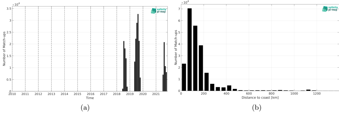
Figure 1: Number of match-ups between Saildrone and SMOS SSS L3 Arctic v2 - 9 Days (CATDS-CEC-LOCEAN) SSS as a function of time (a) and as function of the distance to coast (b) over the Global Ocean Pi-MEP region and for the full satellite product period.
