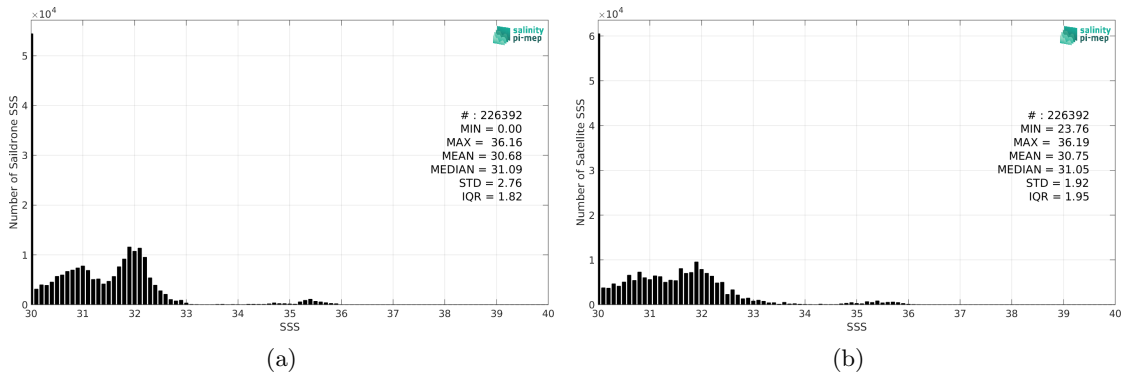
Figure 2: Histograms of SSS from Saildrone (a) and SMOS SSS L3 Arctic v2 - 9 Days (CATDS-CEC-LOCEAN) (b) considering all match-up pairs per bins of 0.1 over the Global Ocean Pi-MEP region and for the full satellite product period.
