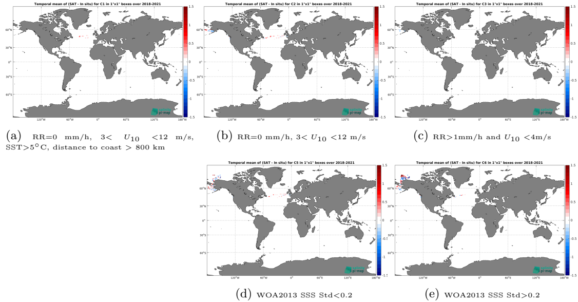
Figure 12: Temporal mean gridded over spatial boxes of size 1^{\circ}\times 1^{\circ} of \Delta\text{SSS} (SMOS SSS L3 Arctic v2 - 9 Days (CATDS-CEC-LOCEAN) - Saildrone) for 5 different subdatasets corresponding to:RR=0 mm/h, 3 < U_{10} < 12 m/s, SST >5^{\circ}\text{C} , distance to coast > 800 km (a), RR=0 mm/h, 3 < U_{10} < 12 m/s (b), RR >1 mm/h and U_{10} < 4 m/s (c), WOA2013 SSS Std <0.2 (d), WOA2013 SSS Std >0.2 (e).
