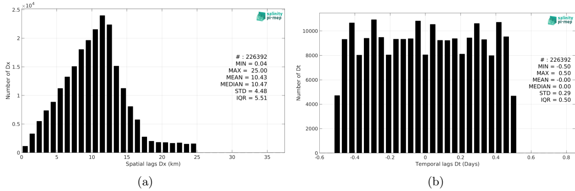
Figure 5: Histograms of the spatial (a) and temporal (b) lags between the location/time of the Saildrone measurement and the date of the corresponding SMOS SSS L3 Arctic v2 - 9 Days (CATDS-CEC-LOCEAN) SSS pixel.
