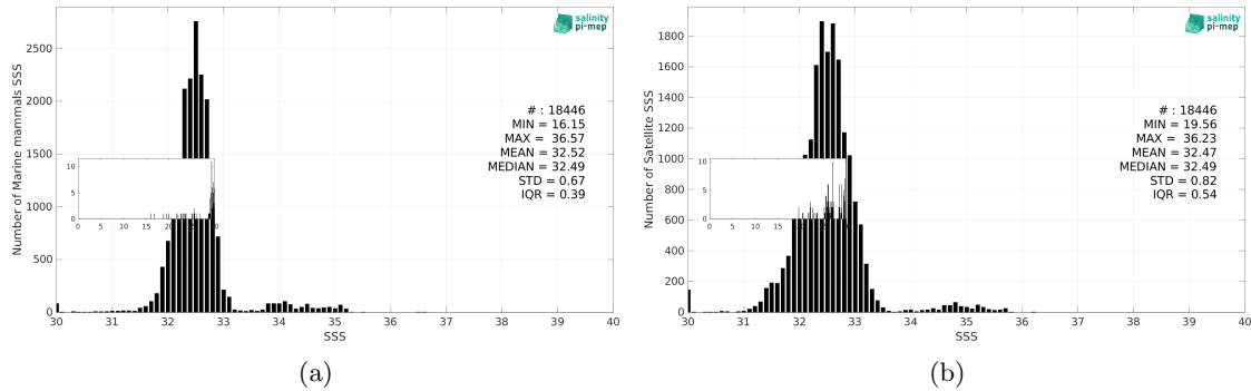
Figure 3: Histograms of SSS from Marine mammals (a) and SMOS SSS L3 Arctic v2 - 9 Days (CATDS-CEC-LOCEAN) (b) considering all match-up pairs per bins of 0.1 over the Global Ocean Pi-MEP region and for the full satellite product period.
