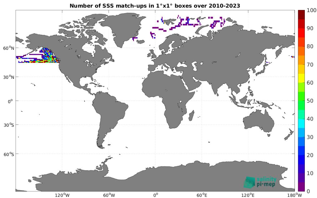
Figure 5: Number of SSS match-ups between Marine mammals SSS and the SMOS SSS L3 Arctic v2 - 9 Days (CATDS-CEC-LOCEAN) SSS product for the Global Ocean Pi-MEP region over 1^\circ \times 1^\circ boxes and for the full satellite product period.
