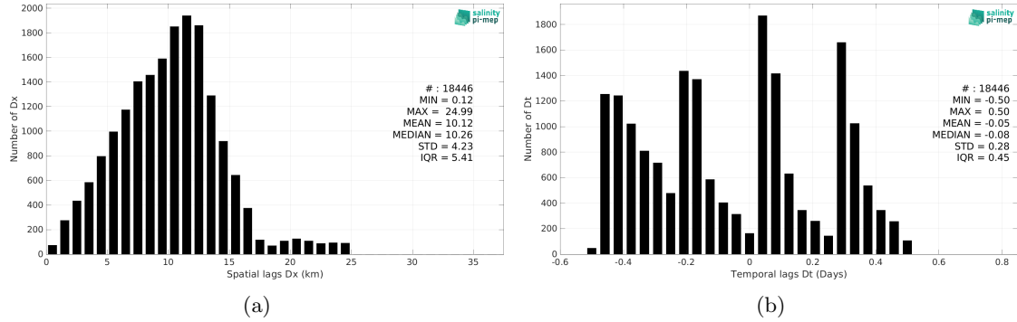
Figure 6: Histograms of the spatial (a) and temporal (b) lags between the location/time of the Marine mammals measurement and the date of the corresponding SMOS SSS L3 Arctic v2 - 9 Days (CATDS-CEC-LOCEAN) SSS pixel.
