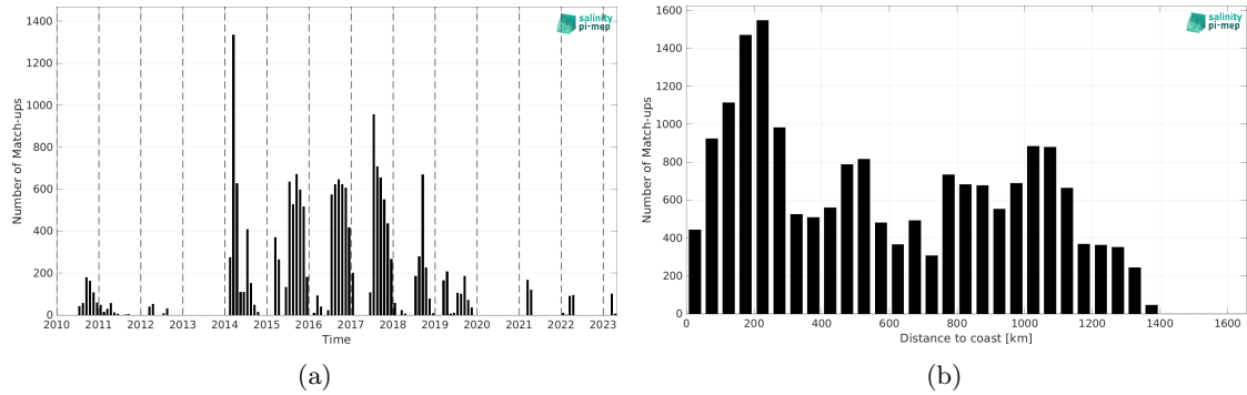
Figure 2: Number of match-ups between Marine mammals and SMOS SSS L3 Arctic v2 - 9 Days (CATDS-CEC-LOCEAN) SSS as a function of time (a) and as function of the distance to coast (b) over the Global Ocean Pi-MEP region and for the full satellite product period.
