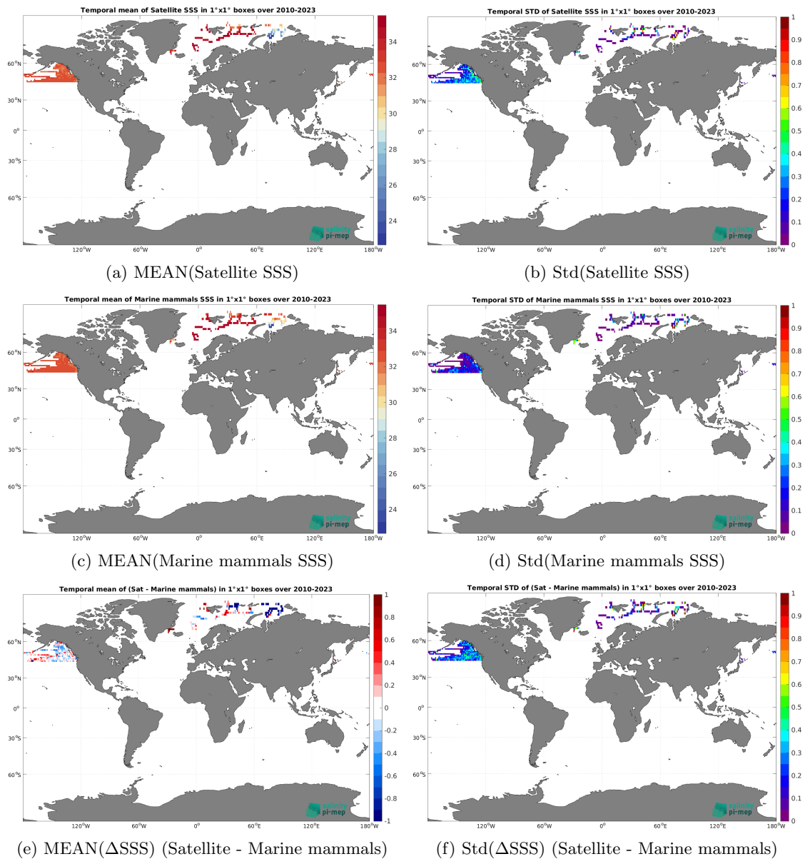
Figure 7: Temporal mean (left) and Std (right) of SSS from SMOS SSS L3 Arctic v2 - 9 Days (CATDS-CEC-LOCEAN) (top), Marine mammals (middle), and of \Delta SSS (Satellite - Marine mammals). Only match-up pairs are used to generate these maps.
