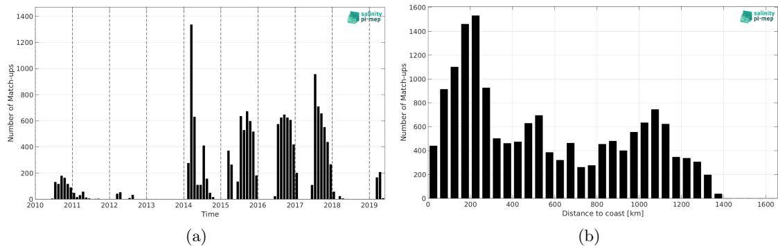
Figure 1: Number of match-ups between Marine mammals and SMOS SSS L3 Arctic v2 - 9 Days (CATDS-CEC-LOCEAN) SSS as a function of time (a) and as function of the distance to coast (b) over the Global Ocean Pi-MEP region and for the full satellite product period.
