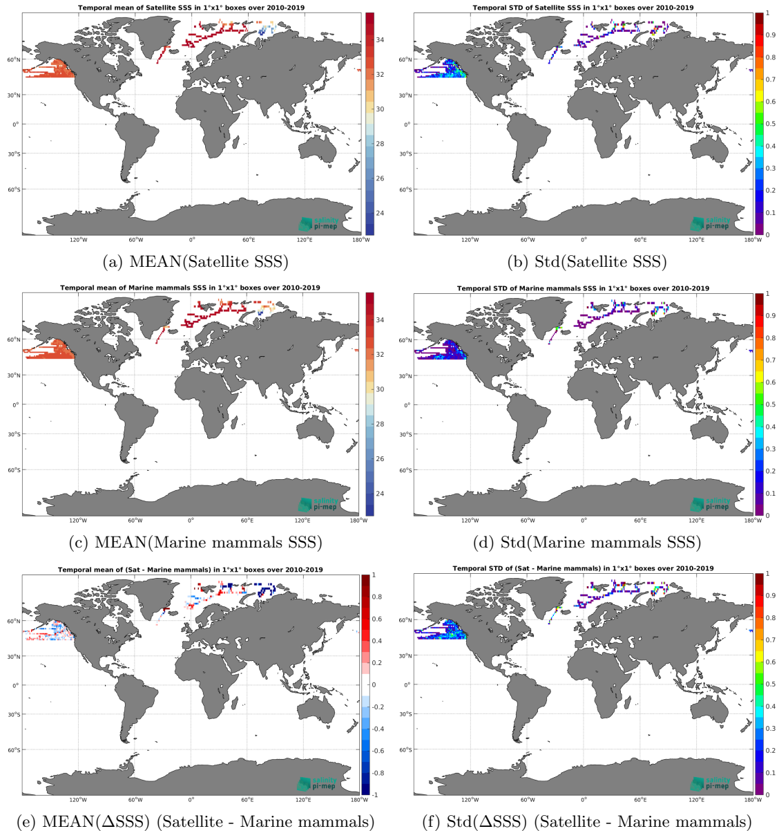
Figure 6: Temporal mean (left) and Std (right) of SSS from SMOS SSS L3 Arctic v2 - 9 Days (CATDS-CEC-LOCEAN) (top), Marine mammals (middle), and of \Delta SSS (Satellite - Marine mammals). Only match-up pairs are used to generate these maps.
