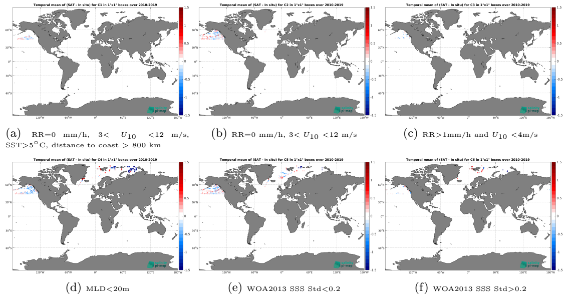
Figure 12: Temporal mean gridded over spatial boxes of size 1^{\circ}\times 1^{\circ} of \Delta\text{SSS} (SMOS SSS L3 Arctic v2 - 9 Days (CATDS-CEC-LOCEAN) - Marine mammals) for 6 different subdatasets corresponding to:RR=0 mm/h, 3 < U_{10} < 12 m/s, SST > 5^{\circ}\text{C} , distance to coast > 800 km (a), RR=0 mm/h, 3 < U_{10} < 12 m/s (b), RR > 1\text{mm/h} and U_{10} < 4\text{m/s} (c),MLD < 20\text{m} (d),WOA2013 SSS Std < 0.2 (e),WOA2013 SSS Std > 0.2 (f).
