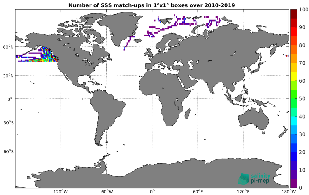
Figure 4: Number of SSS match-ups between Marine mammals SSS and the SMOS SSS L3 Arctic v2 - 9 Days (CATDS-CEC-LOCEAN) SSS product for the Global Ocean Pi-MEP region over 1°×1° boxes and for the full satellite product period.
