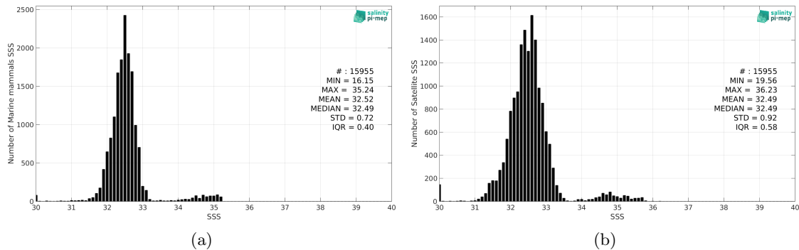
Figure 2: Histograms of SSS from Marine mammals (a) and SMOS SSS L3 Arctic v2 - 9 Days (CATDS-CEC-LOCEAN) (b) considering all match-up pairs per bins of 0.1 over the Global Ocean Pi-MEP region and for the full satellite product period.
