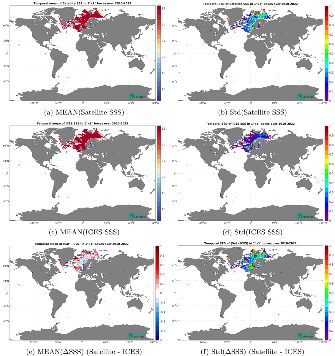
Figure 7: Temporal mean (left) and Std (right) of SSS from SMOS SSS L3 Arctic v2 - 9 Days (CATDS-CEC-LOCEAN) (top), ICES (middle), and of \Delta SSS (Satellite - ICES). Only match-up pairs are used to generate these maps.
