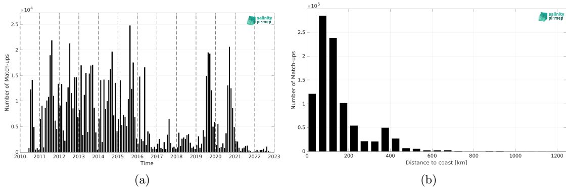
Figure 2: Number of match-ups between ICES and SMOS SSS L3 Arctic v2 - 9 Days (CATDS-CEC-LOCEAN) SSS as a function of time (a) and as function of the distance to coast (b) over the Global Ocean Pi-MEP region and for the full satellite product period.
