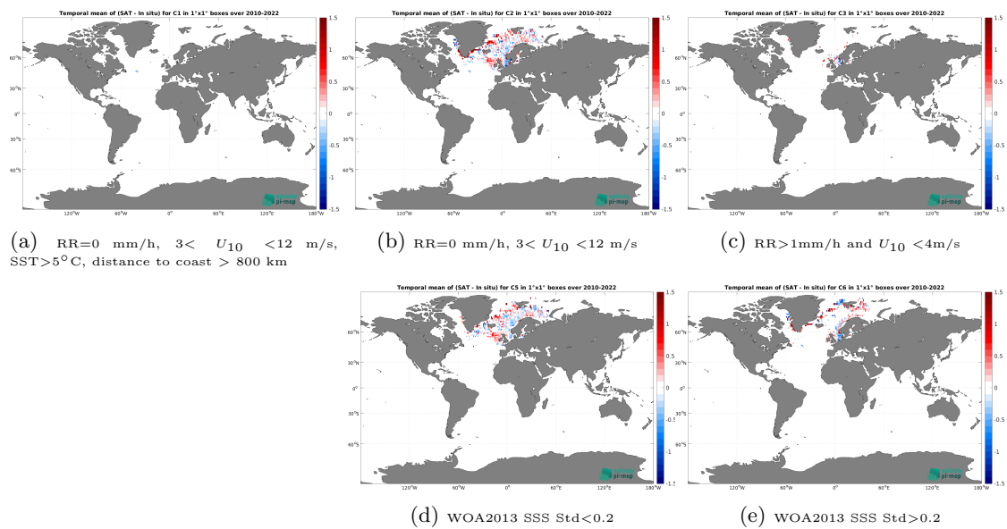
Figure 14: Temporal mean gridded over spatial boxes of size 1^\circ \times 1^\circ of \Delta SSS (SMOS SSS L3 Arctic v2 - 9 Days (CATDS-CEC-LOCEAN) - ICES) for 5 different subdatasets corresponding to: RR=0 mm/h, 3 < U_{10} < 12 m/s, SST > 5^\circ\text{C} , distance to coast > 800 km (a), RR=0 mm/h, 3 < U_{10} < 12 m/s (b), RR > 1 mm/h and U_{10} < 4 m/s (c), WOA2013 SSS Std < 0.2 (d), WOA2013 SSS Std > 0.2 (e).
