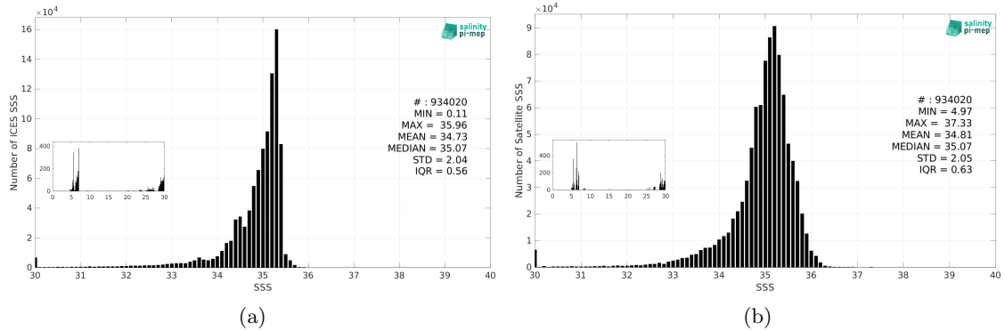
Figure 3: Histograms of SSS from ICES (a) and SMOS SSS L3 Arctic v2 - 9 Days (CATDS-CEC-LOCEAN) (b) considering all match-up pairs per bins of 0.1 over the Global Ocean Pi-MEP region and for the full satellite product period.
