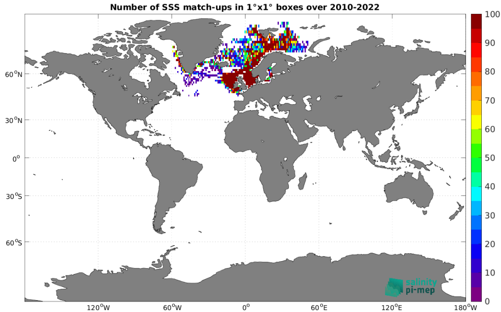
Figure 5: Number of SSS match-ups between ICES SSS and the SMOS SSS L3 Arctic v2 - 9 Days (CATDS-CEC-LOCEAN) SSS product for the Global Ocean Pi-MEP region over 1^\circ \times 1^\circ boxes and for the full satellite product period.
