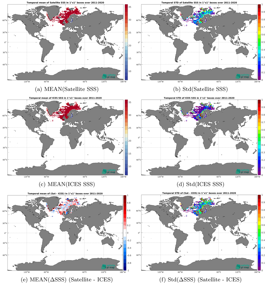
Figure 6: Temporal mean (left) and Std (right) of SSS from SMOS SSS L3 Arctic v2 - 9 Days (CATDS-CEC-LOCEAN) (top), ICES (middle), and of \Delta SSS (Satellite - ICES). Only match-up pairs are used to generate these maps.
