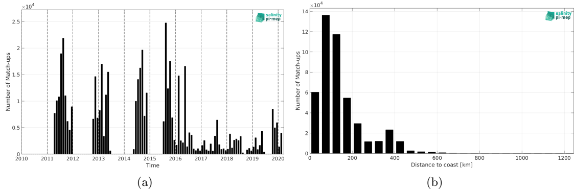
Figure 1: Number of match-ups between ICES and SMOS SSS L3 Arctic v2 - 9 Days (CATDS-CEC-LOCEAN) SSS as a function of time (a) and as function of the distance to coast (b) over the Global Ocean Pi-MEP region and for the full satellite product period.
