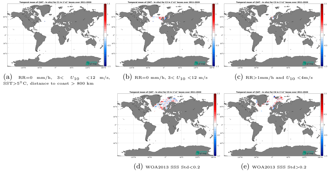
Figure 12: Temporal mean gridded over spatial boxes of size 1^{\circ}\times 1^{\circ} of \Delta\text{SSS} (SMOS SSS L3 Arctic v2 - 9 Days (CATDS-CEC-LOCEAN) - ICES) for 5 different subdatasets corresponding to:RR=0 mm/h, 3 < U_{10} < 12 m/s, SST >5^{\circ}\text{C} , distance to coast > 800 km (a), RR=0 mm/h, 3 < U_{10} < 12 m/s (b), RR >1 mm/h and U_{10} < 4 m/s (c), WOA2013 SSS Std <0.2 (d), WOA2013 SSS Std >0.2 (e).
