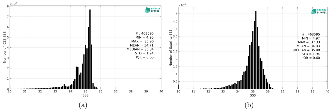
Figure 2: Histograms of SSS from ICES (a) and SMOS SSS L3 Arctic v2 - 9 Days (CATDS-CEC-LOCEAN) (b) considering all match-up pairs per bins of 0.1 over the Global Ocean Pi-MEP region and for the full satellite product period.
