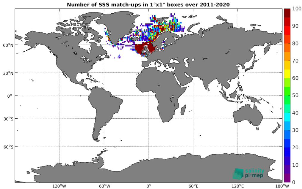
Figure 4: Number of SSS match-ups between ICES SSS and the SMOS SSS L3 Arctic v2 - 9 Days (CATDS-CEC-LOCEAN) SSS product for the Global Ocean Pi-MEP region over 1^\circ \times 1^\circ boxes and for the full satellite product period.
