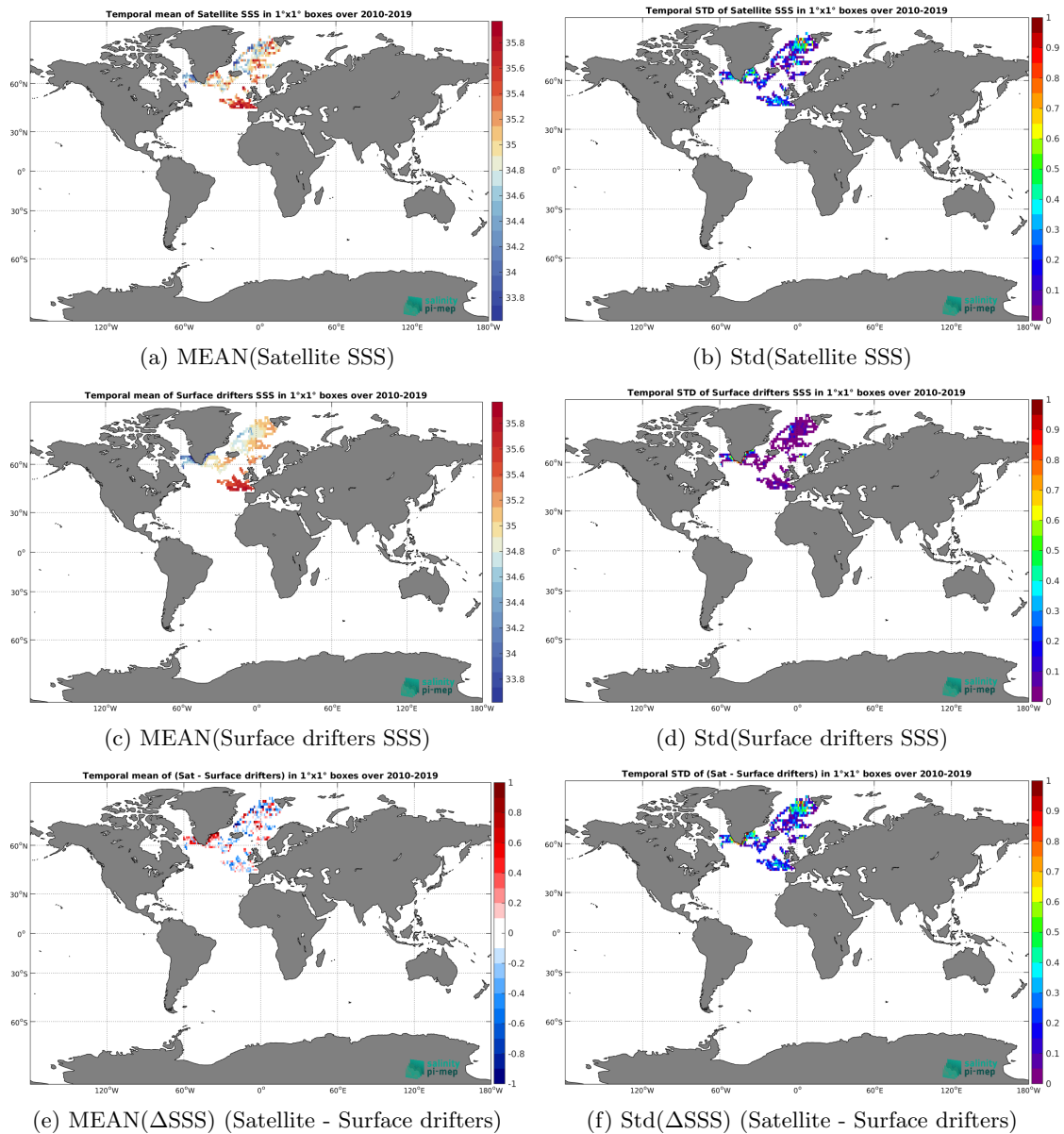
Figure 5: Temporal mean (left) and Std (right) of SSS from SMOS SSS L3 Arctic v2 - 9 Days (CATDS-CEC-LOCEAN) (top), Surface drifters (middle), and of \Delta SSS (Satellite - Surface drifters). Only match-up pairs are used to generate these maps.
