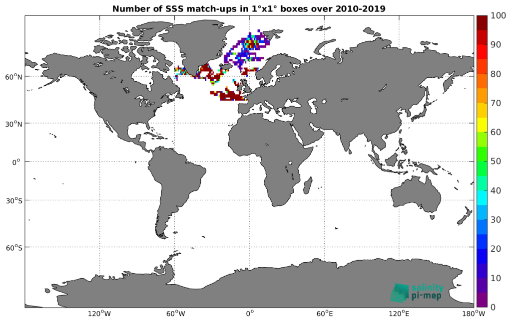
Figure 3: Number of SSS match-ups between Surface drifters SSS and the SMOS SSS L3 Arctic v2 - 9 Days (CATDS-CEC-LOCEAN) SSS product for the Global Ocean Pi-MEP region over 1^\circ \times 1^\circ boxes and for the full satellite product period.
