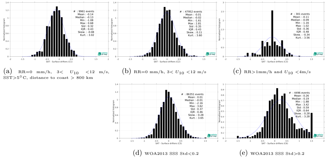
Figure 12: Normalized histogram of \Delta SSS (SMOS SSS L3 Arctic v2 - 9 Days (CATDS-CEC-LOCEAN) - Surface drifters) for 5 different subdatasets corresponding to: RR=0 mm/h, 3 < U_{10} < 12 m/s, SST>5°C, distance to coast > 800 km (a), RR=0 mm/h, 3 < U_{10} < 12 m/s (b), RR>1mm/h and U_{10} < 4 m/s (c), WOA2013 SSS Std<0.2 (d), WOA2013 SSS Std>0.2 (e).
