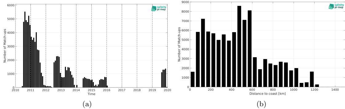
Figure 1: Number of match-ups between Surface drifters and SMOS SSS L3 Arctic v2 - 9 Days (CATDS-CEC-LOCEAN) SSS as a function of time (a) and as function of the distance to coast (b) over the Global Ocean Pi-MEP region and for the full satellite product period.
