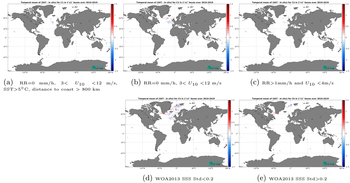
Figure 11: Temporal mean gridded over spatial boxes of size 1^{\circ}\times 1^{\circ} of \Delta\text{SSS} (SMOS SSS L3 Arctic v2 - 9 Days (CATDS-CEC-LOCEAN) - Surface drifters) for 5 different subdatasets corresponding to:RR=0 mm/h, 3 < U_{10} < 12 m/s, SST >5^{\circ}\text{C} , distance to coast > 800 km (a), RR=0 mm/h, 3 < U_{10} < 12 m/s (b), RR >1 mm/h and U_{10} < 4 m/s (c), WOA2013 SSS Std <0.2 (d), WOA2013 SSS Std >0.2 (e).
