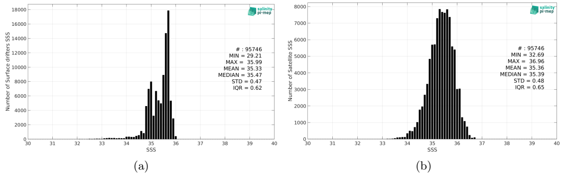
Figure 2: Histograms of SSS from Surface drifters (a) and SMOS SSS L3 Arctic v2 - 9 Days (CATDS-CEC-LOCEAN) (b) considering all match-up pairs per bins of 0.1 over the Global Ocean Pi-MEP region and for the full satellite product period.
