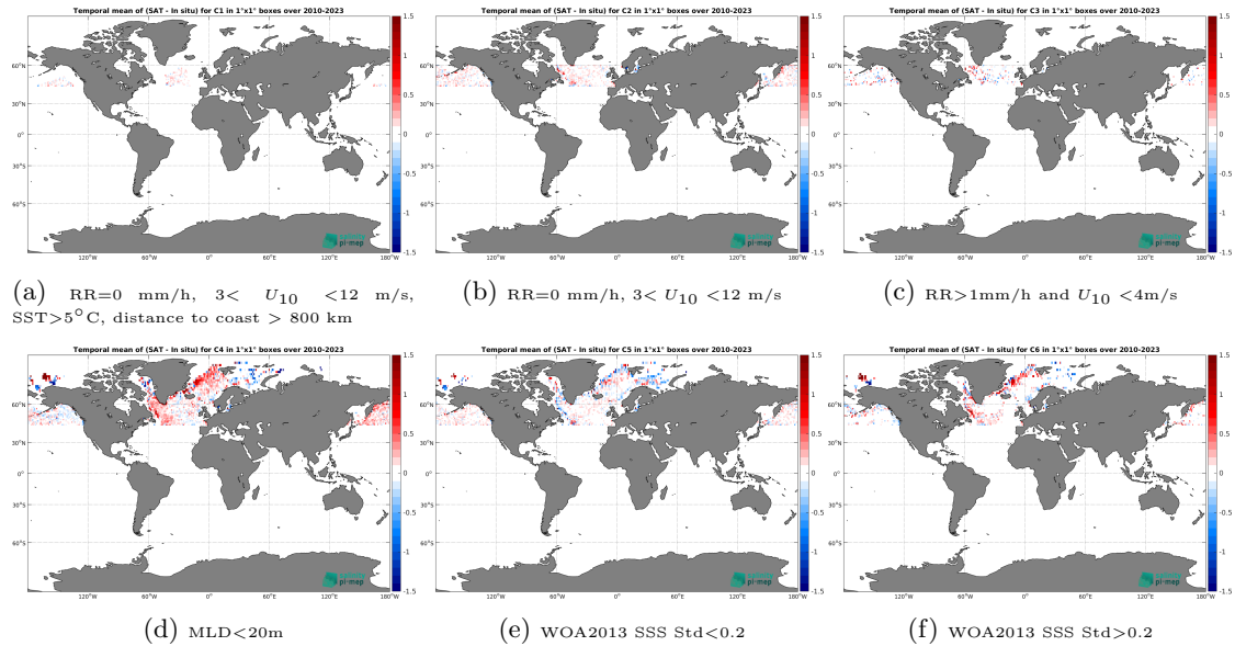
Figure 12: Temporal mean gridded over spatial boxes of size 1^{\circ}\times 1^{\circ} of \Delta\text{SSS} (SMOS SSS L3 Arctic v2 - 9 Days (CATDS-CEC-LOCEAN) - Argo) for 6 different subdatasets corresponding to:RR=0 mm/h, 3 < U_{10} < 12 m/s, SST > 5^{\circ}\text{C} , distance to coast > 800 km (a), RR=0 mm/h, 3 < U_{10} < 12 m/s (b), RR > 1\text{mm/h} and U_{10} < 4\text{m/s} (c),MLD < 20\text{m} (d),WOA2013 SSS Std < 0.2 (e),WOA2013 SSS Std > 0.2 (f).
