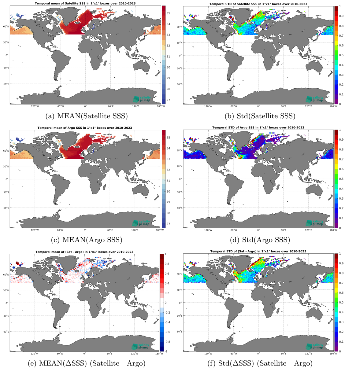
Figure 6: Temporal mean (left) and Std (right) of SSS from SMOS SSS L3 Arctic v2 - 9 Days (CATDS-CEC-LOCEAN) (top), Argo (middle), and of \Delta SSS (Satellite - Argo). Only match-up pairs are used to generate these maps.
