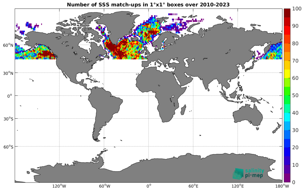
Figure 4: Number of SSS match-ups between Argo SSS and the SMOS SSS L3 Arctic v2 - 9 Days (CATDS-CEC-LOCEAN) SSS product for the Global Ocean Pi-MEP region over 1^\circ \times 1^\circ boxes and for the full satellite product period.
