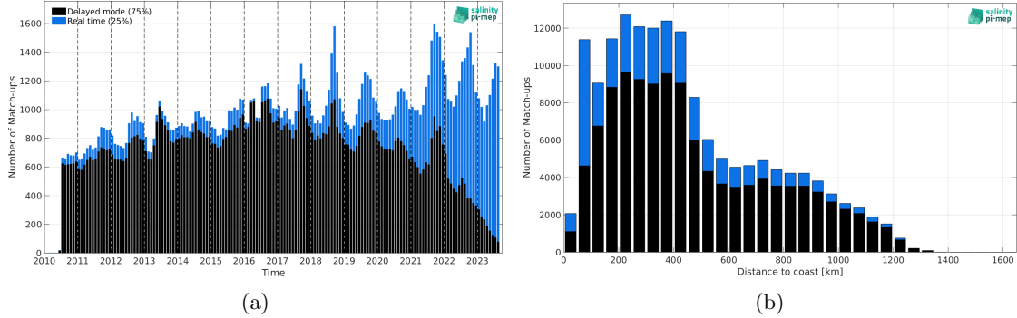
Figure 1: Number of match-ups between Argo and SMOS SSS L3 Arctic v2 - 9 Days (CATDS-CEC-LOCEAN) SSS as a function of time (a) and as function of the distance to coast (b) over the Global Ocean Pi-MEP region and for the full satellite product period.
