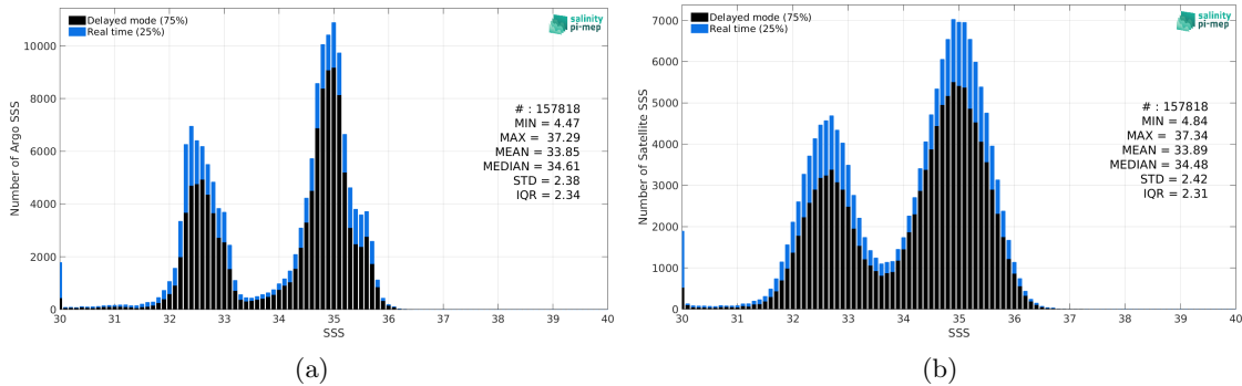
Figure 2: Histograms of SSS from Argo (a) and SMOS SSS L3 Arctic v2 - 9 Days (CATDS-CEC-LOCEAN) (b) considering all match-up pairs per bins of 0.1 over the Global Ocean Pi-MEP region and for the full satellite product period.
