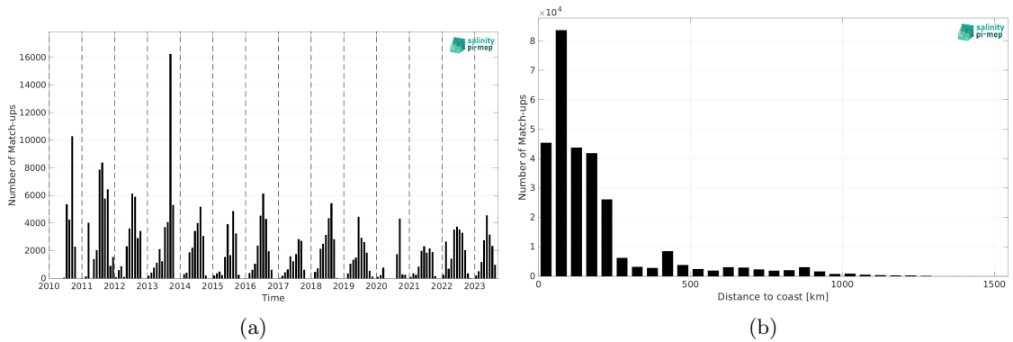
Figure 2: Number of match-ups between TSG (SAMOS) and SMOS SSS L3 Arctic v2 - 18 Days (CATDS-CEC-LOCEAN) SSS as a function of time (a) and as function of the distance to coast (b) over the Global Ocean Pi-MEP region and for the full satellite product period.
