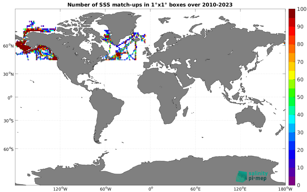
Figure 5: Number of SSS match-ups between TSG (SAMOS) SSS and the SMOS SSS L3 Arctic v2 - 18 Days (CATDS-CEC-LOCEAN) SSS product for the Global Ocean Pi-MEP region over 1^\circ \times 1^\circ boxes and for the full satellite product period.
