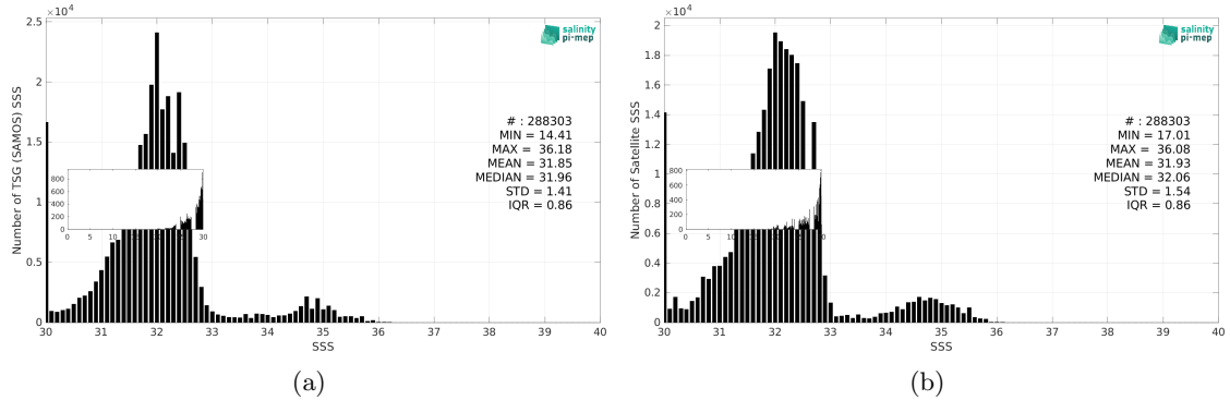
Figure 3: Histograms of SSS from TSG (SAMOS) (a) and SMOS SSS L3 Arctic v2 - 18 Days (CATDS-CEC-LOCEAN) (b) considering all match-up pairs per bins of 0.1 over the Global Ocean Pi-MEP region and for the full satellite product period.
