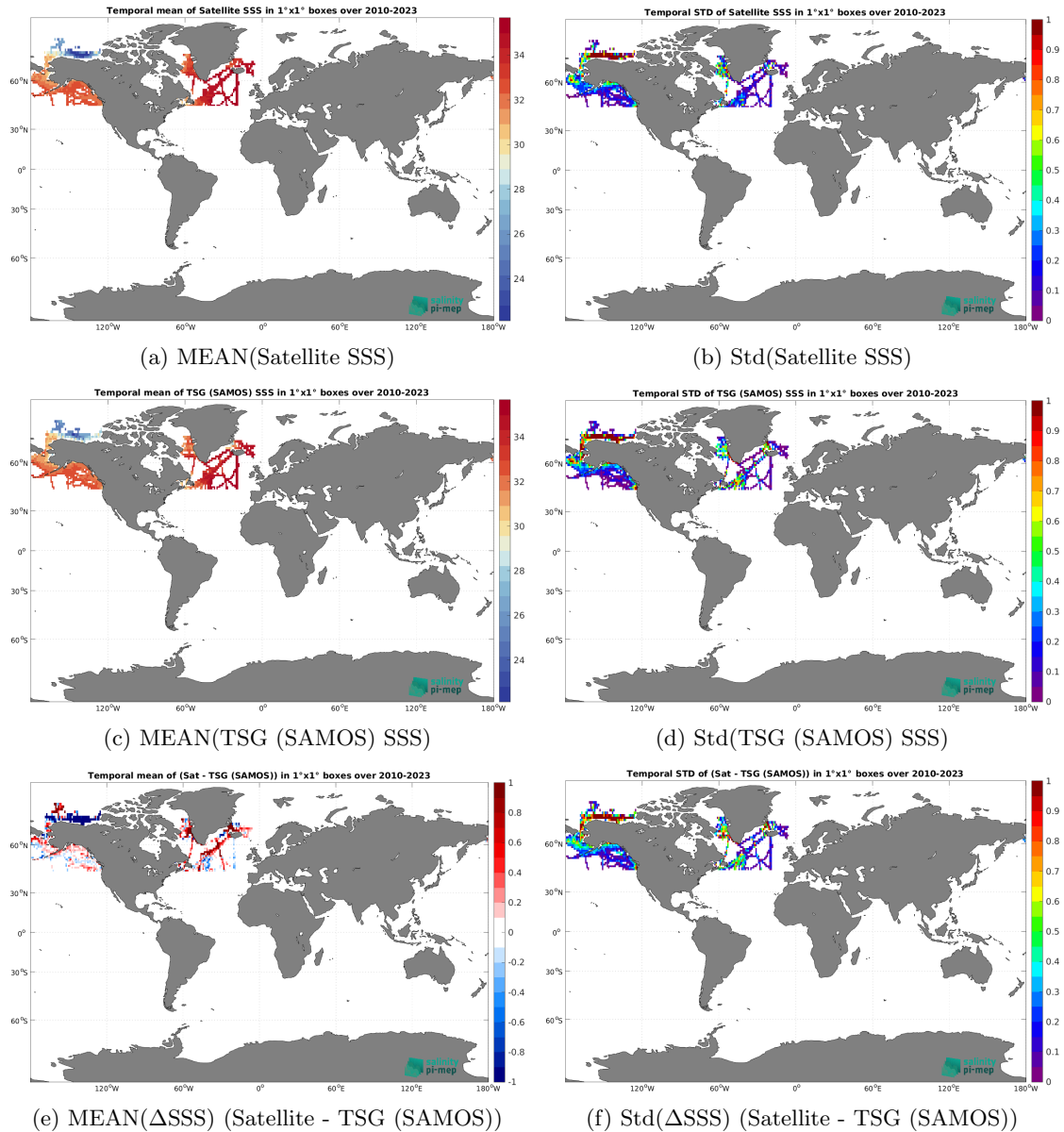
Figure 7: Temporal mean (left) and Std (right) of SSS from SMOS SSS L3 Arctic v2 - 18 Days (CATDS-CEC-LOCEAN) (top), TSG (SAMOS) (middle), and of \Delta SSS (Satellite - TSG (SAMOS)). Only match-up pairs are used to generate these maps.
