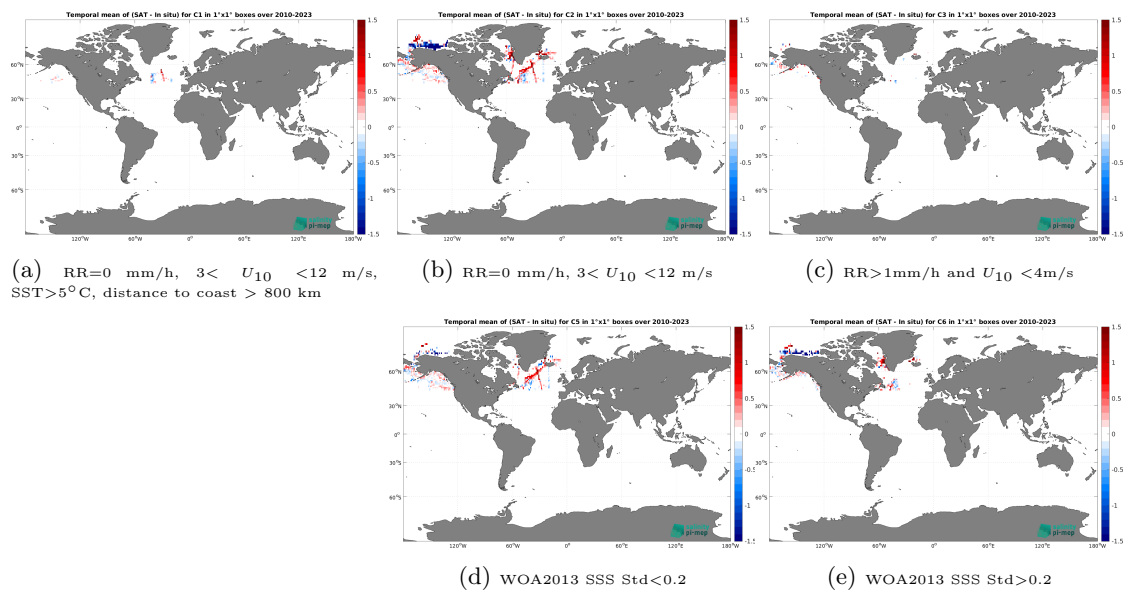
Figure 14: Temporal mean gridded over spatial boxes of size 1^\circ \times 1^\circ of \Delta SSS (SMOS SSS L3 Arctic v2 - 18 Days (CATDS-CEC-LOCEAN) - TSG (SAMOS)) for 5 different subdatasets corresponding to: RR=0 mm/h, 3 < U_{10} < 12 m/s, SST > 5^\circ\text{C} , distance to coast > 800 km (a), RR=0 mm/h, 3 < U_{10} < 12 m/s (b), RR > 1 mm/h and U_{10} < 4 m/s (c), WOA2013 SSS Std < 0.2 (d), WOA2013 SSS Std > 0.2 (e).
