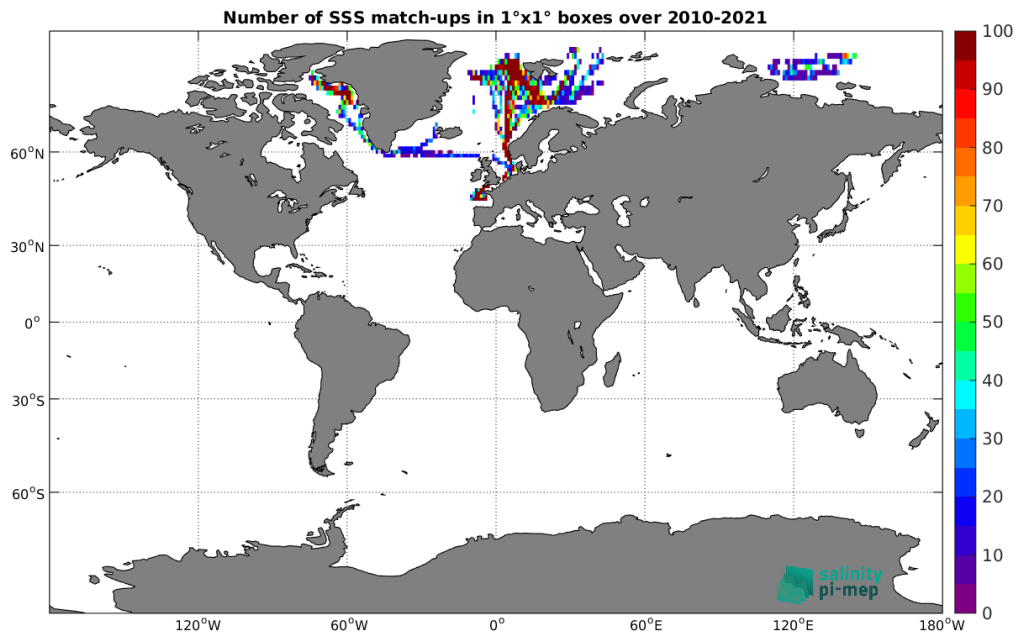
Figure 4: Number of SSS match-ups between TSG (Polarstern) SSS and the SMOS SSS L3 Arctic v2 - 18 Days (CATDS-CEC-LOCEAN) SSS product for the Global Ocean Pi-MEP region over 1^\circ \times 1^\circ boxes and for the full satellite product period.
