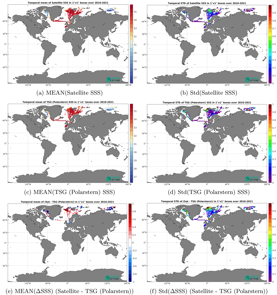
Figure 6: Temporal mean (left) and Std (right) of SSS from SMOS SSS L3 Arctic v2 - 18 Days (CATDS-CEC-LOCEAN) (top), TSG (Polarstern) (middle), and of \Delta SSS (Satellite - TSG (Polarstern)). Only match-up pairs are used to generate these maps.
