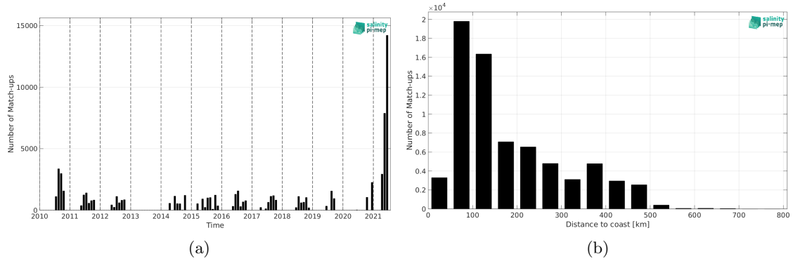
Figure 1: Number of match-ups between TSG (Polarstern) and SMOS SSS L3 Arctic v2 - 18 Days (CATDS-CEC-LOCEAN) SSS as a function of time (a) and as function of the distance to coast (b) over the Global Ocean Pi-MEP region and for the full satellite product period.
