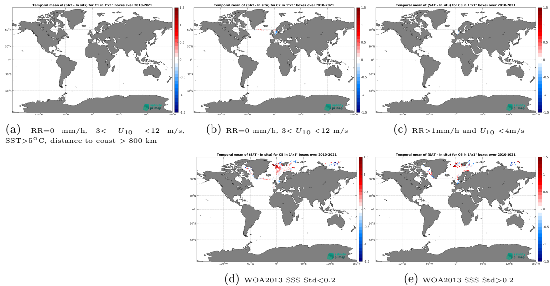
Figure 12: Temporal mean gridded over spatial boxes of size 1^{\circ}\times 1^{\circ} of \Delta\text{SSS} (SMOS SSS L3 Arctic v2 - 18 Days (CATDS-CEC-LOCEAN) - TSG (Polarstern)) for 5 different subdatasets corresponding to:RR=0 mm/h, 3 < U_{10} < 12 m/s, SST > 5^{\circ}\text{C} , distance to coast > 800 km (a), RR=0 mm/h, 3 < U_{10} < 12 m/s (b), RR > 1 mm/h and U_{10} < 4 m/s (c), WOA2013 SSS Std < 0.2 (d), WOA2013 SSS Std > 0.2 (e).
