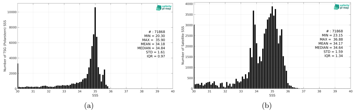
Figure 2: Histograms of SSS from TSG (Polarstern) (a) and SMOS SSS L3 Arctic v2 - 18 Days (CATDS-CEC-LOCEAN) (b) considering all match-up pairs per bins of 0.1 over the Global Ocean Pi-MEP region and for the full satellite product period.
