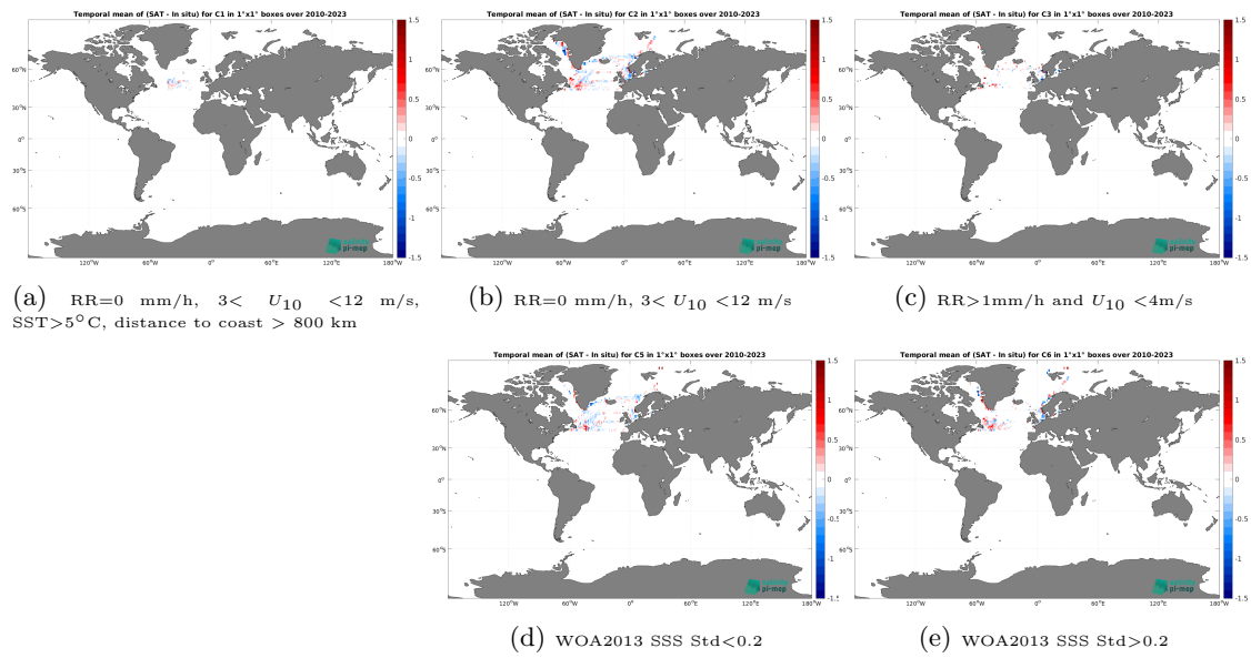
Figure 14: Temporal mean gridded over spatial boxes of size 1^\circ \times 1^\circ of \Delta SSS (SMOS SSS L3 Arctic v2 - 18 Days (CATDS-CEC-LOCEAN) - TSG (LEGOS-DM)) for 5 different subdatasets corresponding to:RR=0 mm/h, 3 < U_{10} < 12 m/s, SST > 5^\circ\text{C} , distance to coast > 800 km (a), RR=0 mm/h, 3 < U_{10} < 12 m/s (b), RR > 1 mm/h and U_{10} < 4 m/s (c), WOA2013 SSS Std < 0.2 (d), WOA2013 SSS Std > 0.2 (e).
