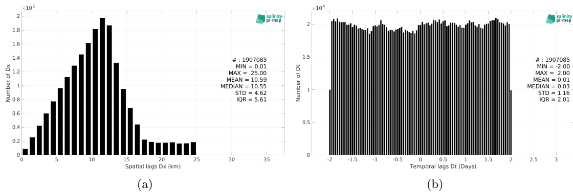
Figure 6: Histograms of the spatial (a) and temporal (b) lags between the location/time of the TSG (LEGOS-DM) measurement and the date of the corresponding SMOS SSS L3 Arctic v2 - 18 Days (CATDS-CEC-LOCEAN) SSS pixel.
