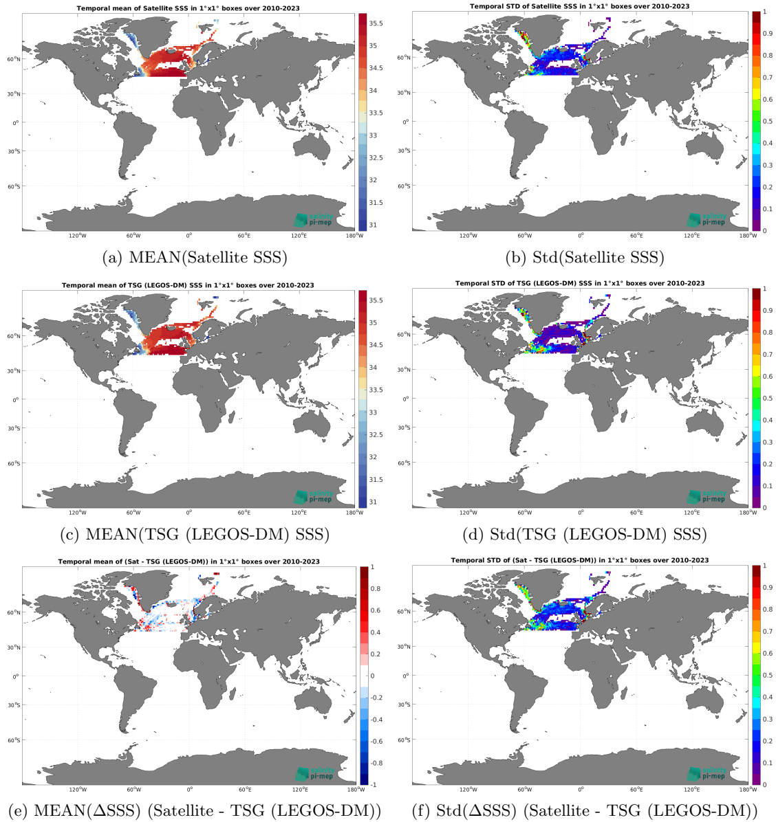
Figure 7: Temporal mean (left) and Std (right) of SSS from SMOS SSS L3 Arctic v2 - 18 Days (CATDS-CEC-LOCEAN) (top), TSG (LEGOS-DM) (middle), and of \Delta SSS (Satellite - TSG (LEGOS-DM)). Only match-up pairs are used to generate these maps.
