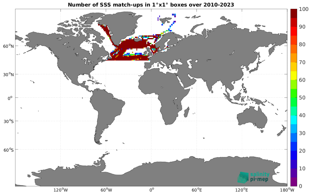
Figure 5: Number of SSS match-ups between TSG (LEGOS-DM) SSS and the SMOS SSS L3 Arctic v2 - 18 Days (CATDS-CEC-LOCEAN) SSS product for the Global Ocean Pi-MEP region over 1^\circ \times 1^\circ boxes and for the full satellite product period.
