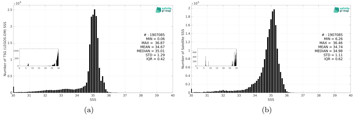
Figure 3: Histograms of SSS from TSG (LEGOS-DM) (a) and SMOS SSS L3 Arctic v2 - 18 Days (CATDS-CEC-LOCEAN) (b) considering all match-up pairs per bins of 0.1 over the Global Ocean Pi-MEP region and for the full satellite product period.
