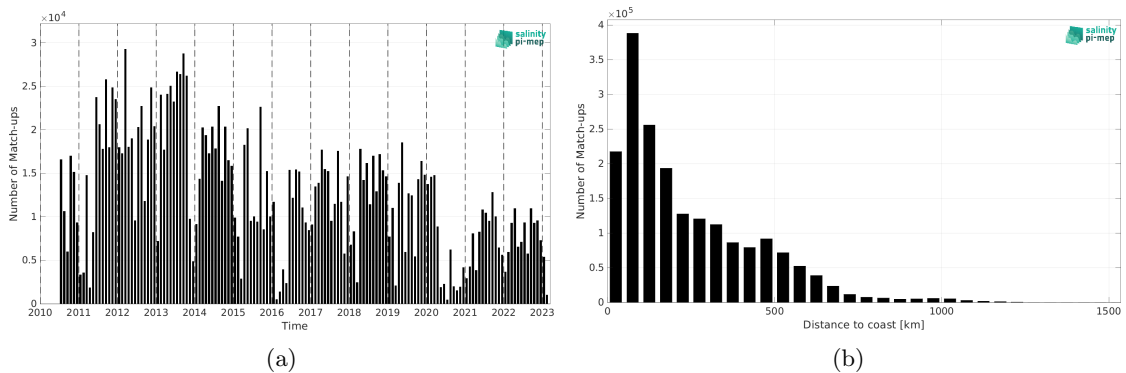
Figure 2: Number of match-ups between TSG (LEGOS-DM) and SMOS SSS L3 Arctic v2 - 18 Days (CATDS-CEC-LOCEAN) SSS as a function of time (a) and as function of the distance to coast (b) over the Global Ocean Pi-MEP region and for the full satellite product period.
