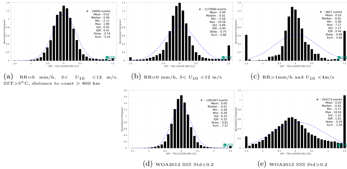
Figure 15: Normalized histogram of \Delta SSS (SMOS SSS L3 Arctic v2 - 18 Days (CATDS-CEC-LOCEAN) - TSG (LEGOS-DM)) for 5 different subdatasets corresponding to: RR=0 mm/h, 3 < U_{10} < 12 m/s, SST > 5°C, distance to coast > 800 km (a), RR=0 mm/h, 3 < U_{10} < 12 m/s (b), RR > 1mm/h and U_{10} < 4 m/s (c), WOA2013 SSS Std < 0.2 (d), WOA2013 SSS Std > 0.2 (e).
