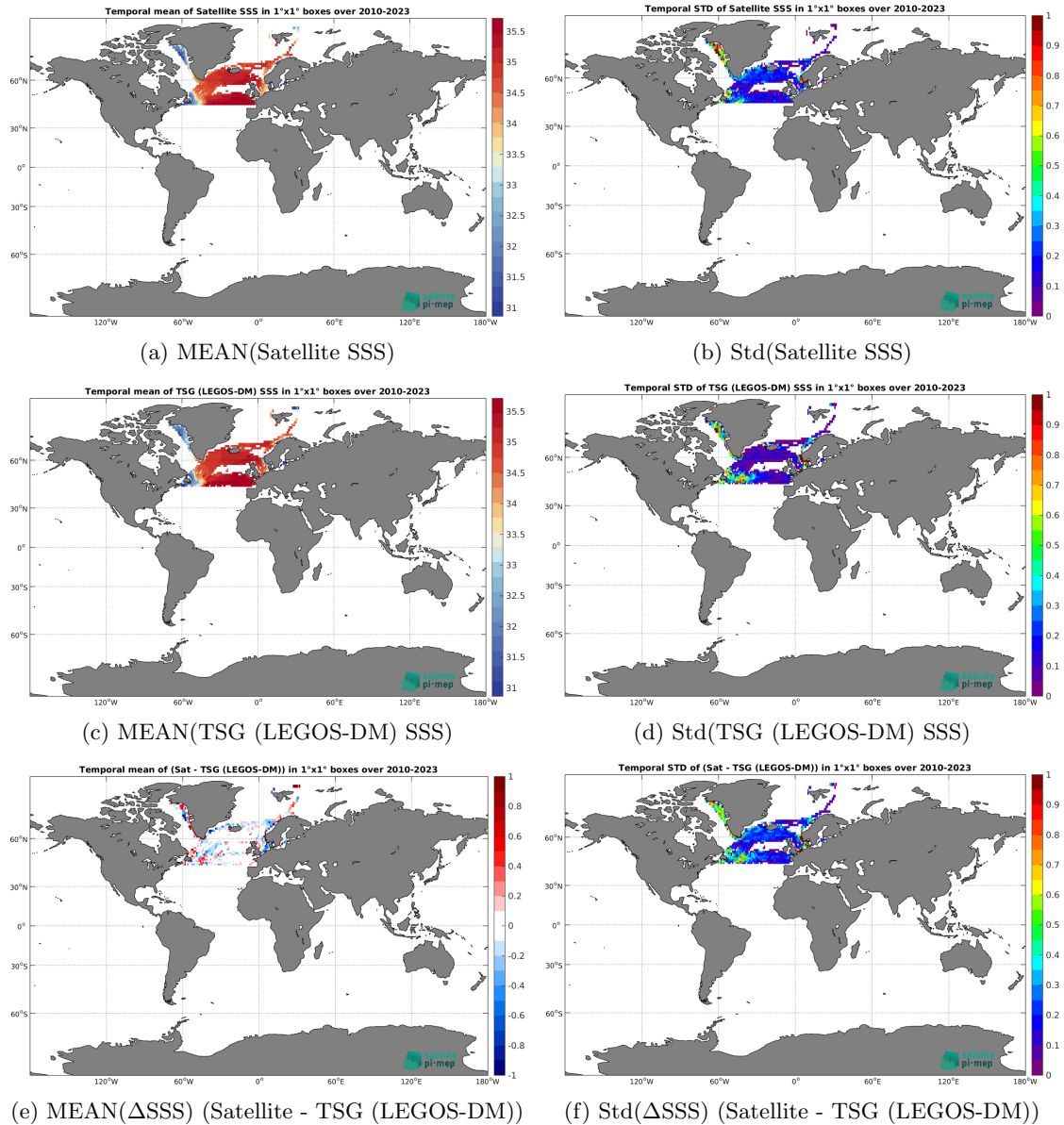
Figure 6: Temporal mean (left) and Std (right) of SSS from SMOS SSS L3 Arctic v2 - 18 Days (CATDS-CEC-LOCEAN) (top), TSG (LEGOS-DM) (middle), and of \Delta SSS (Satellite - TSG (LEGOS-DM)). Only match-up pairs are used to generate these maps.
