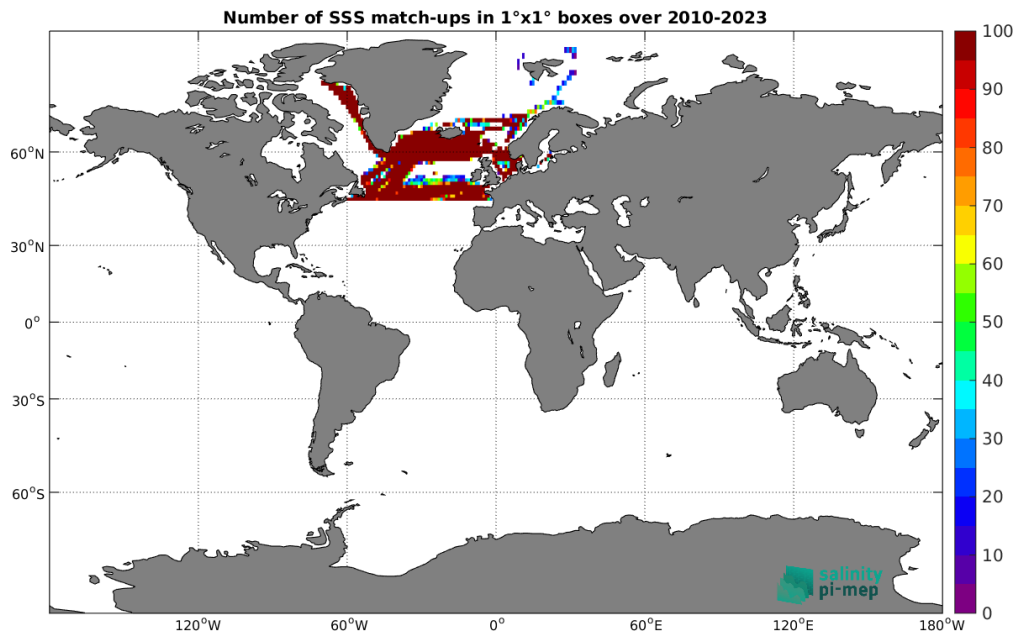
Figure 4: Number of SSS match-ups between TSG (LEGOS-DM) SSS and the SMOS SSS L3 Arctic v2 - 18 Days (CATDS-CEC-LOCEAN) SSS product for the Global Ocean Pi-MEP region over 1^\circ \times 1^\circ boxes and for the full satellite product period.
