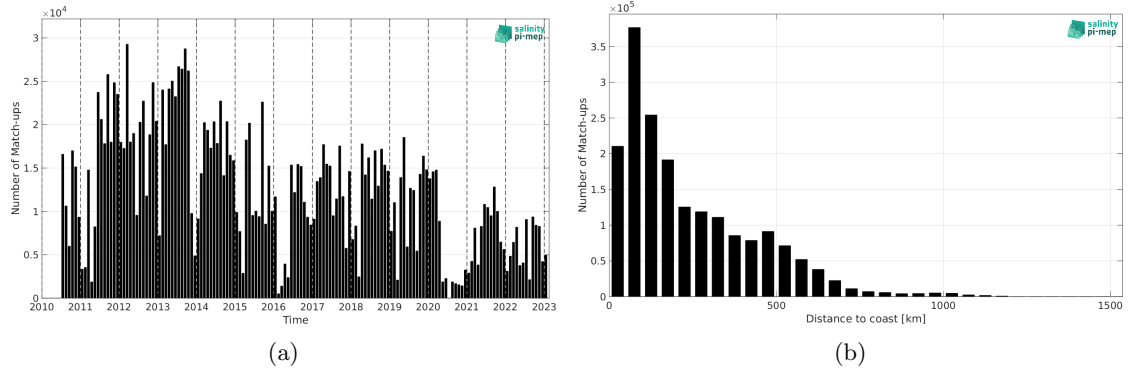
Figure 1: Number of match-ups between TSG (LEGOS-DM) and SMOS SSS L3 Arctic v2 - 18 Days (CATDS-CEC-LOCEAN) SSS as a function of time (a) and as function of the distance to coast (b) over the Global Ocean Pi-MEP region and for the full satellite product period.
