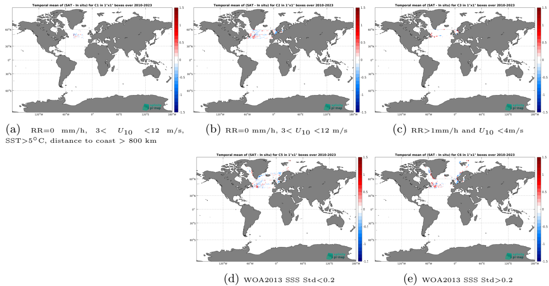
Figure 12: Temporal mean gridded over spatial boxes of size 1^{\circ}\times 1^{\circ} of \Delta\text{SSS} (SMOS SSS L3 Arctic v2 - 18 Days (CATDS-CEC-LOCEAN) - TSG (LEGOS-DM)) for 5 different subdatasets corresponding to:RR=0 mm/h, 3 < U_{10} < 12 m/s, SST > 5^{\circ}\text{C} , distance to coast > 800 km (a), RR=0 mm/h, 3 < U_{10} < 12 m/s (b), RR > 1 mm/h and U_{10} < 4 m/s (c), WOA2013 SSS Std < 0.2 (d), WOA2013 SSS Std > 0.2 (e).
