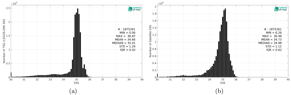
Figure 2: Histograms of SSS from TSG (LEGOS-DM) (a) and SMOS SSS L3 Arctic v2 - 18 Days (CATDS-CEC-LOCEAN) (b) considering all match-up pairs per bins of 0.1 over the Global Ocean Pi-MEP region and for the full satellite product period.
