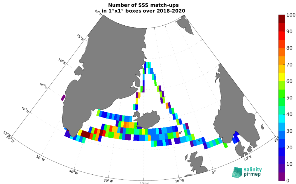
Figure 5: Number of SSS match-ups between TSG (Lauge-Koch) SSS and the SMOS SSS L3 Arctic v2 - 18 Days (CATDS-CEC-LOCEAN) SSS product for the Global Ocean Pi-MEP region over 1^\circ \times 1^\circ boxes and for the full satellite product period.
