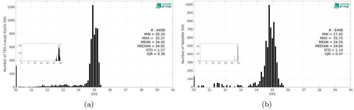
Figure 3: Histograms of SSS from TSG (Lauge-Koch) (a) and SMOS SSS L3 Arctic v2 - 18 Days (CATDS-CEC-LOCEAN) (b) considering all match-up pairs per bins of 0.1 over the Global Ocean Pi-MEP region and for the full satellite product period.
