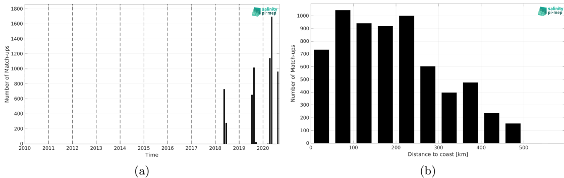
Figure 2: Number of match-ups between TSG (Lauge-Koch) and SMOS SSS L3 Arctic v2 - 18 Days (CATDS-CEC-LOCEAN) SSS as a function of time (a) and as function of the distance to coast (b) over the Global Ocean Pi-MEP region and for the full satellite product period.
