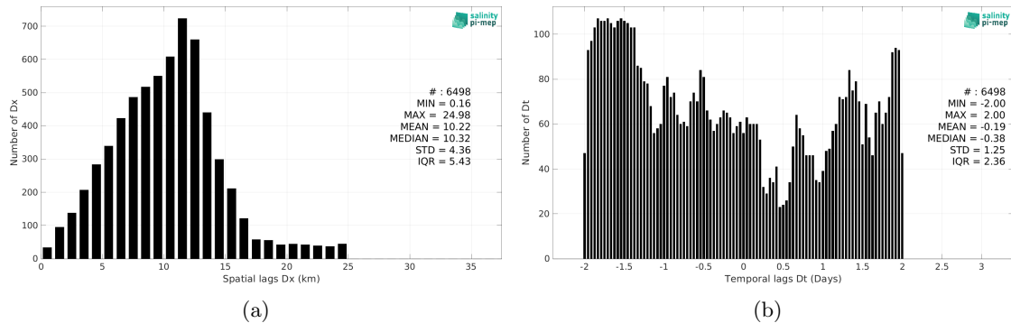
Figure 6: Histograms of the spatial (a) and temporal (b) lags between the location/time of the TSG (Lauge-Koch) measurement and the date of the corresponding SMOS SSS L3 Arctic v2 - 18 Days (CATDS-CEC-LOCEAN) SSS pixel.
