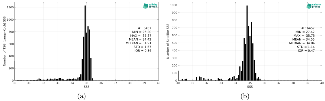
Figure 2: Histograms of SSS from TSG (Lauge-Koch) (a) and SMOS SSS L3 Arctic v2 - 18 Days (CATDS-CEC-LOCEAN) (b) considering all match-up pairs per bins of 0.1 over the Global Ocean Pi-MEP region and for the full satellite product period.
