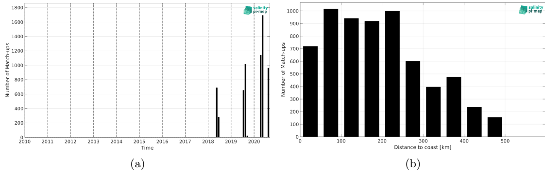
Figure 1: Number of match-ups between TSG (Lauge-Koch) and SMOS SSS L3 Arctic v2 - 18 Days (CATDS-CEC-LOCEAN) SSS as a function of time (a) and as function of the distance to coast (b) over the Global Ocean Pi-MEP region and for the full satellite product period.
