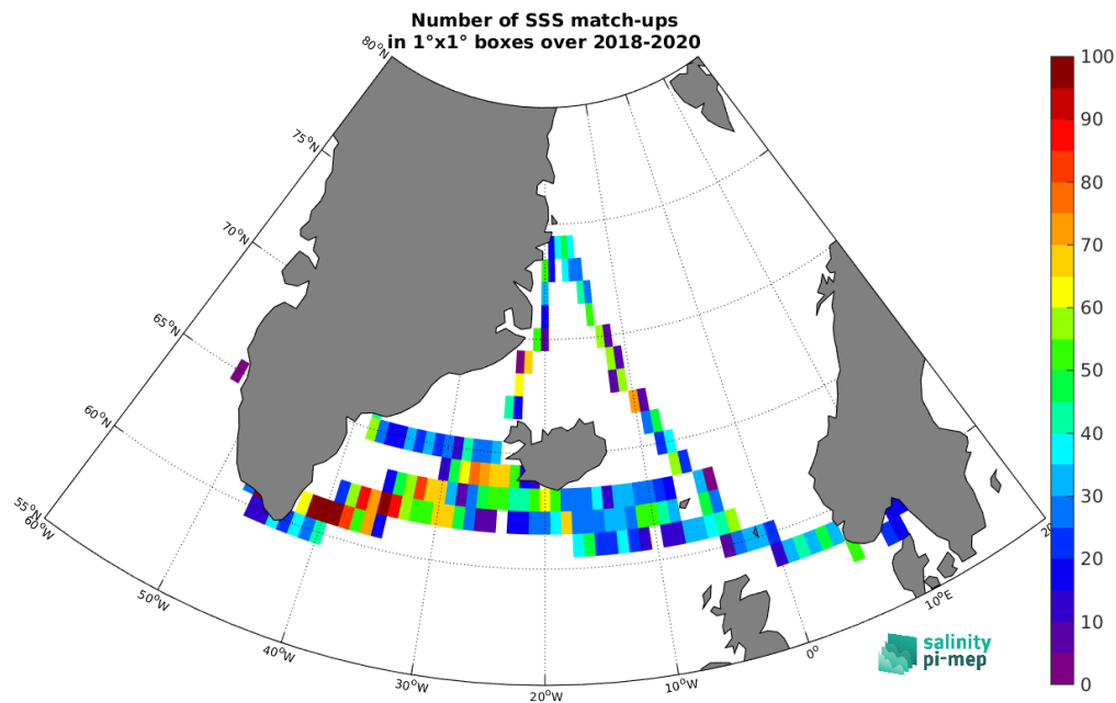
Figure 4: Number of SSS match-ups between TSG (Lauge-Koch) SSS and the SMOS SSS L3 Arctic v2 - 18 Days (CATDS-CEC-LOCEAN) SSS product for the Global Ocean Pi-MEP region over 1^\circ \times 1^\circ boxes and for the full satellite product period.
