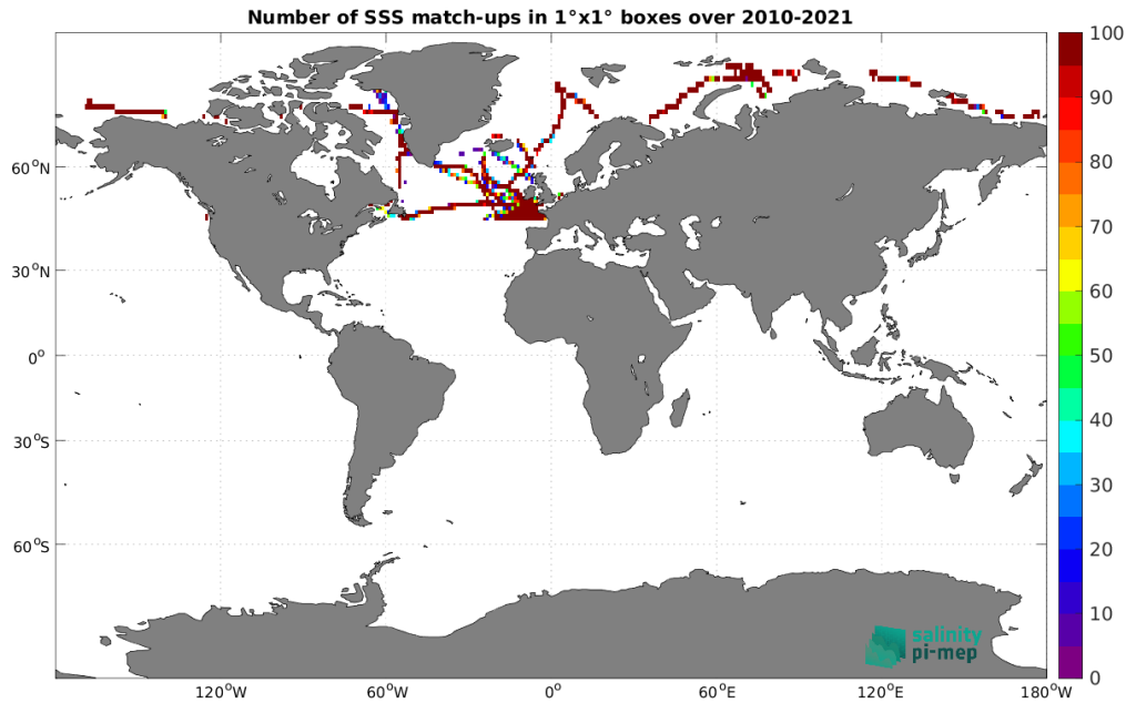
Figure 5: Number of SSS match-ups between TSG (GOSUD-Sailing-ship) SSS and the SMOS SSS L3 Arctic v2 - 18 Days (CATDS-CEC-LOCEAN) SSS product for the Global Ocean Pi-MEP region over 1^\circ \times 1^\circ boxes and for the full satellite product period.
