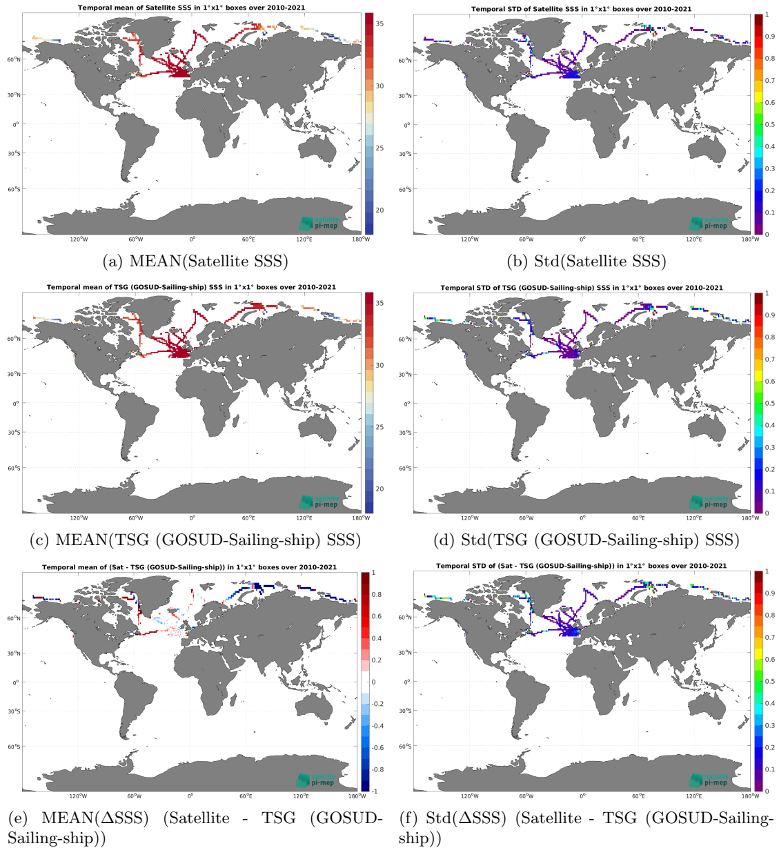
Figure 7: Temporal mean (left) and Std (right) of SSS from SMOS SSS L3 Arctic v2 - 18 Days (CATDS-CEC-LOCEAN) (top), TSG (GOSUD-Sailing-ship) (middle), and of \Delta SSS (Satellite - TSG (GOSUD-Sailing-ship)). Only match-up pairs are used to generate these maps.
