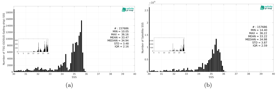
Figure 3: Histograms of SSS from TSG (GOSUD-Sailing-ship) (a) and SMOS SSS L3 Arctic v2 - 18 Days (CATDS-CEC-LOCEAN) (b) considering all match-up pairs per bins of 0.1 over the Global Ocean Pi-MEP region and for the full satellite product period.
