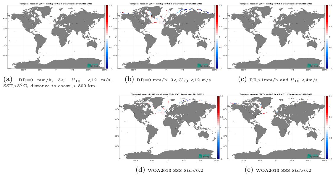
Figure 14: Temporal mean gridded over spatial boxes of size 1^\circ \times 1^\circ of \Delta SSS (SMOS SSS L3 Arctic v2 - 18 Days (CATDS-CEC-LOCEAN) - TSG (GOSUD-Sailing-ship)) for 5 different subdatasets corresponding to:RR=0 mm/h, 3 < U_{10} < 12 m/s, SST > 5^\circ\text{C} , distance to coast > 800 km (a), RR=0 mm/h, 3 < U_{10} < 12 m/s (b), RR > 1 mm/h and U_{10} < 4 m/s (c), WOA2013 SSS Std < 0.2 (d), WOA2013 SSS Std > 0.2 (e).
