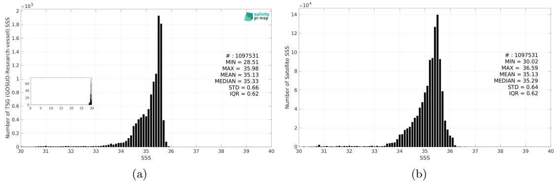
Figure 3: Histograms of SSS from TSG (GOSUD-Research-vessel) (a) and SMOS SSS L3 Arctic v2 - 18 Days (CATDS-CEC-LOCEAN) (b) considering all match-up pairs per bins of 0.1 over the Global Ocean Pi-MEP region and for the full satellite product period.
