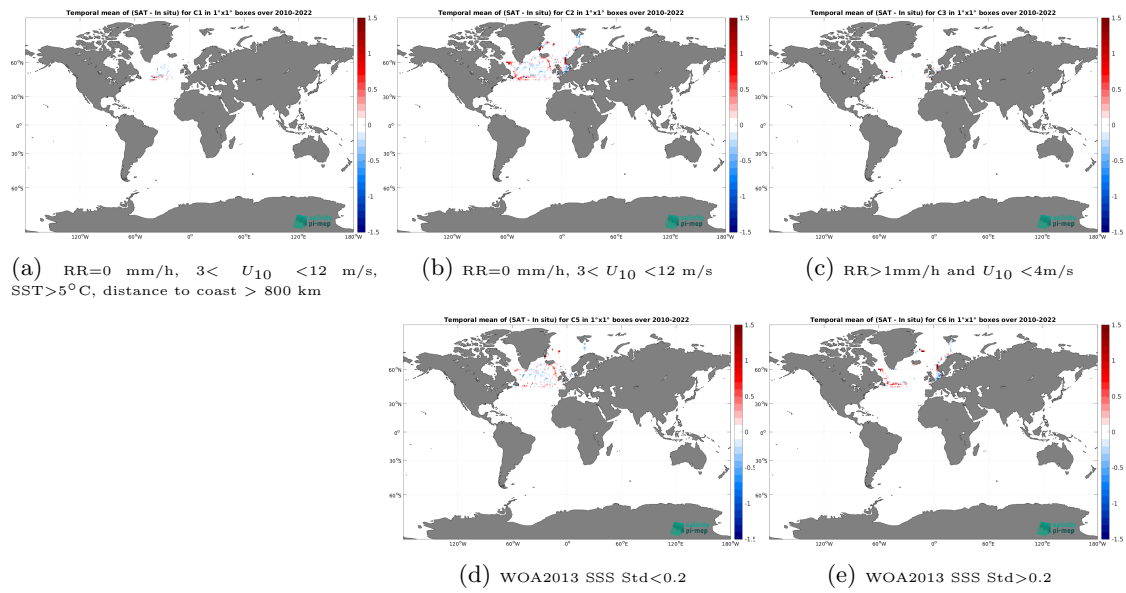
Figure 14: Temporal mean gridded over spatial boxes of size 1^\circ \times 1^\circ of \Delta SSS (SMOS SSS L3 Arctic v2 - 18 Days (CATDS-CEC-LOCEAN) - TSG (GOSUD-Research-vessel)) for 5 different subdatasets corresponding to:RR=0 mm/h, 3 < U_{10} < 12 m/s, SST > 5^\circ\text{C} , distance to coast > 800 km (a), RR=0 mm/h, 3 < U_{10} < 12 m/s (b), RR > 1 mm/h and U_{10} < 4 m/s (c), WOA2013 SSS Std < 0.2 (d), WOA2013 SSS Std > 0.2 (e).
