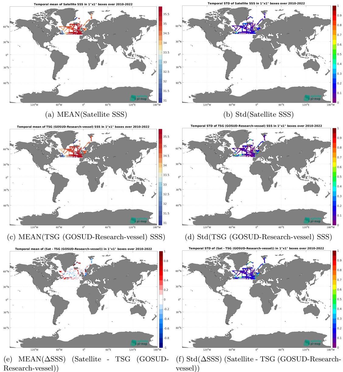
Figure 7: Temporal mean (left) and Std (right) of SSS from SMOS SSS L3 Arctic v2 - 18 Days (CATDS-CEC-LOCEAN) (top), TSG (GOSUD-Research-vessel) (middle), and of \Delta SSS (Satellite - TSG (GOSUD-Research-vessel)). Only match-up pairs are used to generate these maps.
