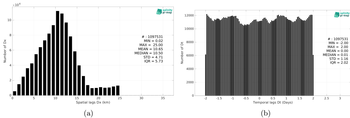
Figure 6: Histograms of the spatial (a) and temporal (b) lags between the location/time of the TSG (GOSUD-Research-vessel) measurement and the date of the corresponding SMOS SSS L3 Arctic v2 - 18 Days (CATDS-CEC-LOCEAN) SSS pixel.
