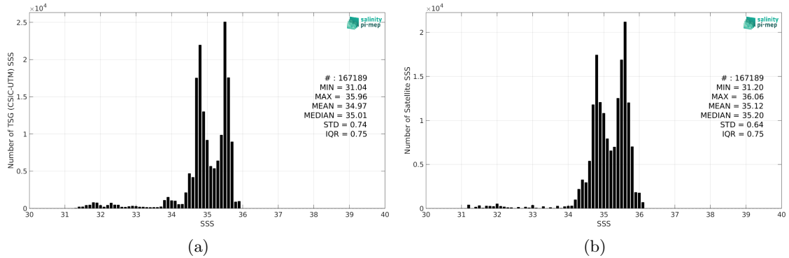
Figure 2: Histograms of SSS from TSG (CSIC-UTM) (a) and SMOS SSS L3 Arctic v2 - 18 Days (CATDS-CEC-LOCEAN) (b) considering all match-up pairs per bins of 0.1 over the Global Ocean Pi-MEP region and for the full satellite product period.
