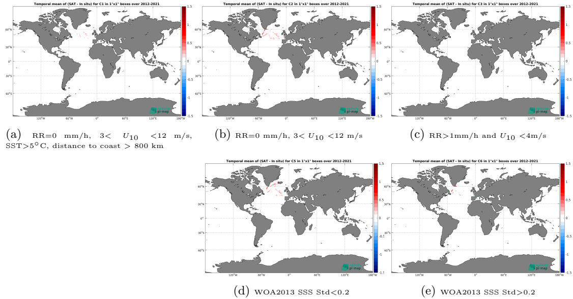
Figure 12: Temporal mean gridded over spatial boxes of size 1^{\circ}\times 1^{\circ} of \Delta\text{SSS} (SMOS SSS L3 Arctic v2 - 18 Days (CATDS-CEC-LOCEAN) - TSG (CSIC-UTM)) for 5 different subdatasets corresponding to:RR=0 mm/h, 3 < U_{10} < 12 m/s, SST >5^{\circ}\text{C} , distance to coast > 800 km (a), RR=0 mm/h, 3 < U_{10} < 12 m/s (b), RR >1 mm/h and U_{10} < 4 m/s (c), WOA2013 SSS Std <0.2 (d), WOA2013 SSS Std >0.2 (e).
