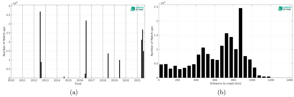
Figure 1: Number of match-ups between TSG (CSIC-UTM) and SMOS SSS L3 Arctic v2 - 18 Days (CATDS-CEC-LOCEAN) SSS as a function of time (a) and as function of the distance to coast (b) over the Global Ocean Pi-MEP region and for the full satellite product period.
