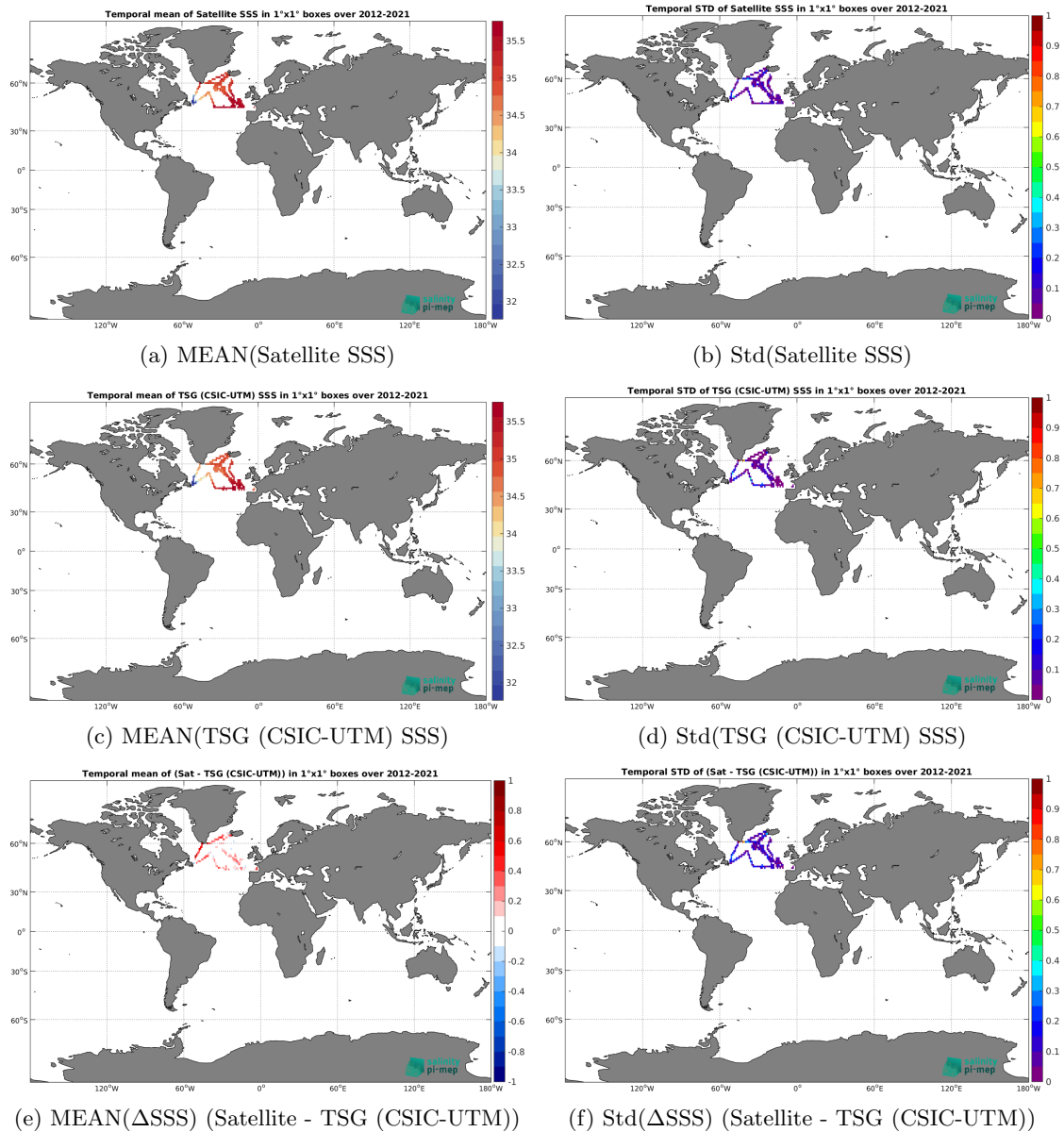
Figure 6: Temporal mean (left) and Std (right) of SSS from SMOS SSS L3 Arctic v2 - 18 Days (CATDS-CEC-LOCEAN) (top), TSG (CSIC-UTM) (middle), and of \Delta SSS (Satellite - TSG (CSIC-UTM)). Only match-up pairs are used to generate these maps.
