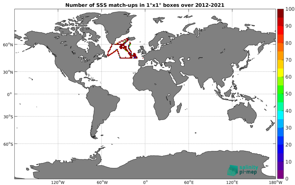
Figure 4: Number of SSS match-ups between TSG (CSIC-UTM) SSS and the SMOS SSS L3 Arctic v2 - 18 Days (CATDS-CEC-LOCEAN) SSS product for the Global Ocean Pi-MEP region over 1^\circ \times 1^\circ boxes and for the full satellite product period.
