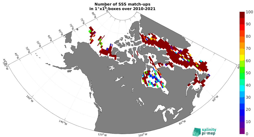
Figure 5: Number of SSS match-ups between TSG (Amundsen) SSS and the SMOS SSS L3 Arctic v2 - 18 Days (CATDS-CEC-LOCEAN) SSS product for the Global Ocean Pi-MEP region over 1^\circ \times 1^\circ boxes and for the full satellite product period.
