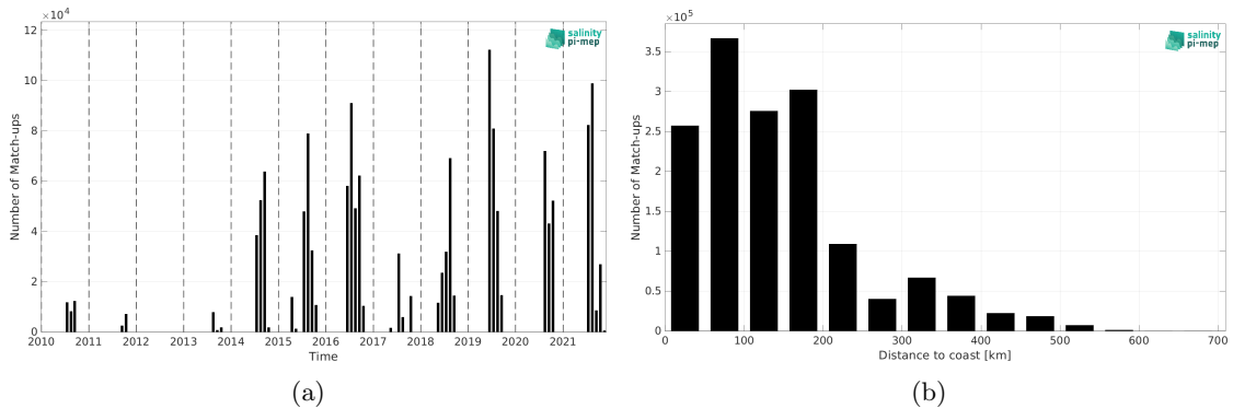
Figure 2: Number of match-ups between TSG (Amundsen) and SMOS SSS L3 Arctic v2 - 18 Days (CATDS-CEC-LOCEAN) SSS as a function of time (a) and as function of the distance to coast (b) over the Global Ocean Pi-MEP region and for the full satellite product period.
