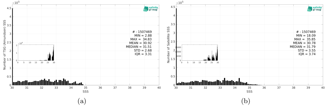
Figure 3: Histograms of SSS from TSG (Amundsen) (a) and SMOS SSS L3 Arctic v2 - 18 Days (CATDS-CEC-LOCEAN) (b) considering all match-up pairs per bins of 0.1 over the Global Ocean Pi-MEP region and for the full satellite product period.
