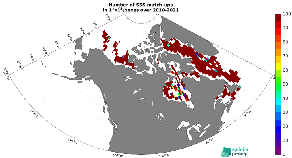
Figure 5: Number of SSS match-ups between TSG (Amundsen) SSS and the SMOS SSS L3 Arctic v2 - 18 Days (CATDS-CEC-LOCEAN) SSS product for the Global Ocean Pi-MEP region over 1°×1° boxes and for the full satellite product period.
