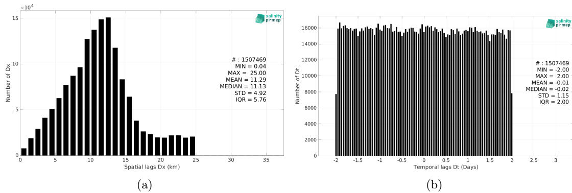
Figure 6: Histograms of the spatial (a) and temporal (b) lags between the location/time of the TSG (Amundsen) measurement and the date of the corresponding SMOS SSS L3 Arctic v2 - 18 Days (CATDS-CEC-LOCEAN) SSS pixel.
