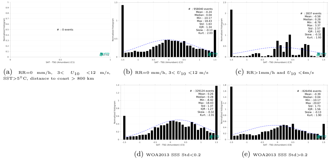
Figure 15: Normalized histogram of \Delta SSS (SMOS SSS L3 Arctic v2 - 18 Days (CATDS-CEC-LOCEAN) - TSG (Amundsen)) for 5 different subdatasets corresponding to: RR=0 mm/h, 3 < U_{10} < 12 m/s, SST > 5°C, distance to coast > 800 km (a), RR=0 mm/h, 3 < U_{10} < 12 m/s (b), RR > 1mm/h and U_{10} < 4 m/s (c), WOA2013 SSS Std < 0.2 (d), WOA2013 SSS Std > 0.2 (e).
