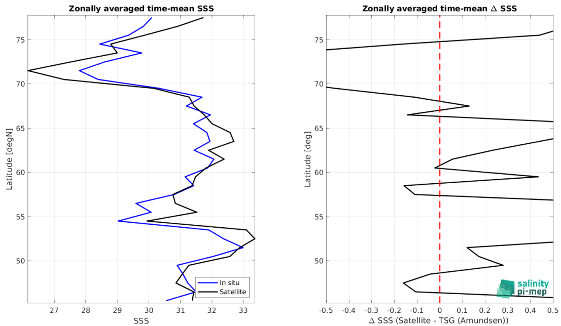
Figure 9: Left panel: Zonal mean SSS from SMOS SSS L3 Arctic v2 - 18 Days (CATDS-CEC-LOCEAN) satellite product (black) and from TSG (Amundsen) (blue). Right panel: Zonal mean of \Delta SSS (Satellite - TSG (Amundsen)) for all the collected Pi-MEP match-up pairs estimated over the full satellite product period.
