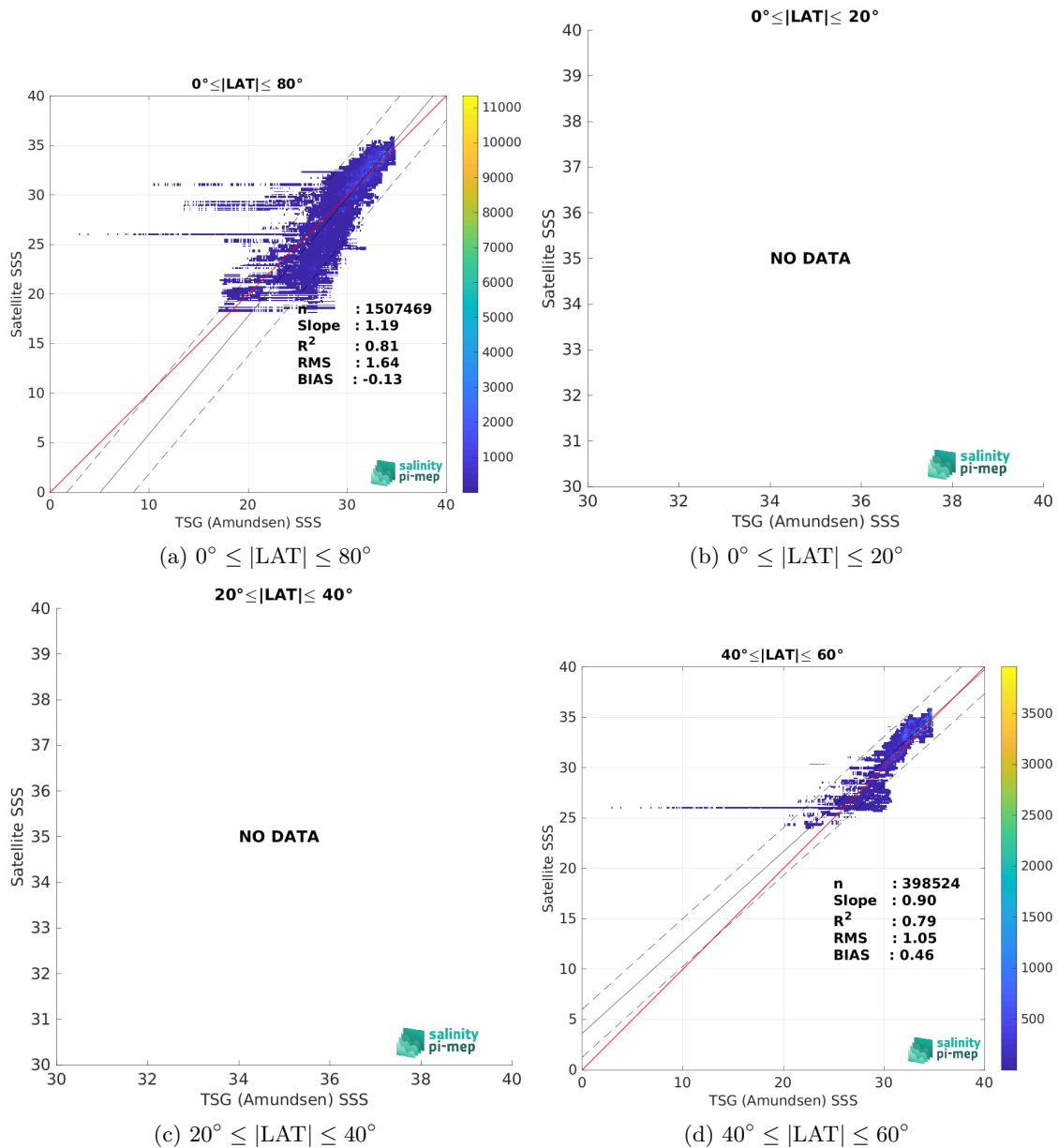
Figure 10: Contour maps of the concentration of SMOS SSS L3 Arctic v2 - 18 Days (CATDS-CEC-LOCEAN) SSS (y-axis) versus TSG (Amundsen) SSS (x-axis) at match-up pairs for different latitude bands. For each plot, the red line shows x=y . The black thin and dashed lines indicate a linear fit through the data cloud and the \pm 95\% confidence levels, respectively. The number match-up pairs n , the slope and R^2 coefficient of the linear fit, the root mean square (RMS) and the mean bias between satellite and in situ data are indicated for each latitude band in each plots.
