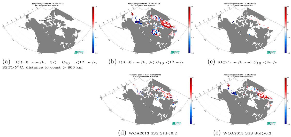
Figure 14: Temporal mean gridded over spatial boxes of size 1^\circ \times 1^\circ of \Delta SSS (SMOS SSS L3 Arctic v2 - 18 Days (CATDS-CEC-LOCEAN) - TSG (Amundsen)) for 5 different subdatasets corresponding to:RR=0 mm/h, 3 < U_{10} < 12 m/s, SST > 5°C, distance to coast > 800 km (a), RR=0 mm/h, 3 < U_{10} < 12 m/s (b), RR > 1mm/h and U_{10} < 4 m/s (c), WOA2013 SSS Std < 0.2 (d), WOA2013 SSS Std > 0.2 (e).
