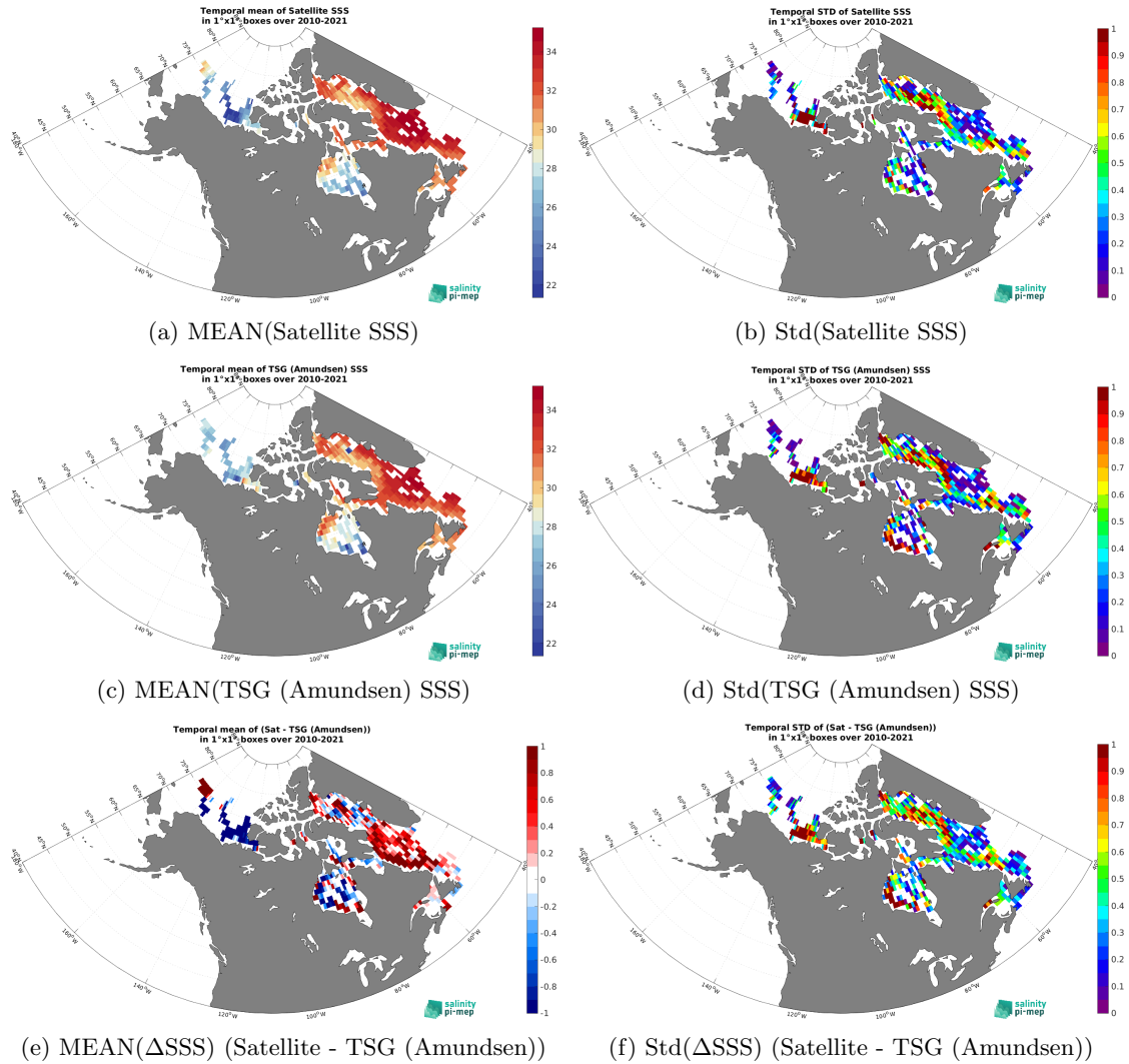
Figure 7: Temporal mean (left) and Std (right) of SSS from SMOS SSS L3 Arctic v2 - 18 Days (CATDS-CEC-LOCEAN) (top), TSG (Amundsen) (middle), and of \Delta SSS (Satellite - TSG (Amundsen)). Only match-up pairs are used to generate these maps.
