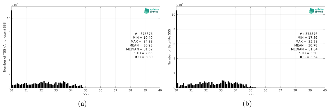
Figure 2: Histograms of SSS from TSG (Amundsen) (a) and SMOS SSS L3 Arctic v2 - 18 Days (CATDS-CEC-LOCEAN) (b) considering all match-up pairs per bins of 0.1 over the Global Ocean Pi-MEP region and for the full satellite product period.
