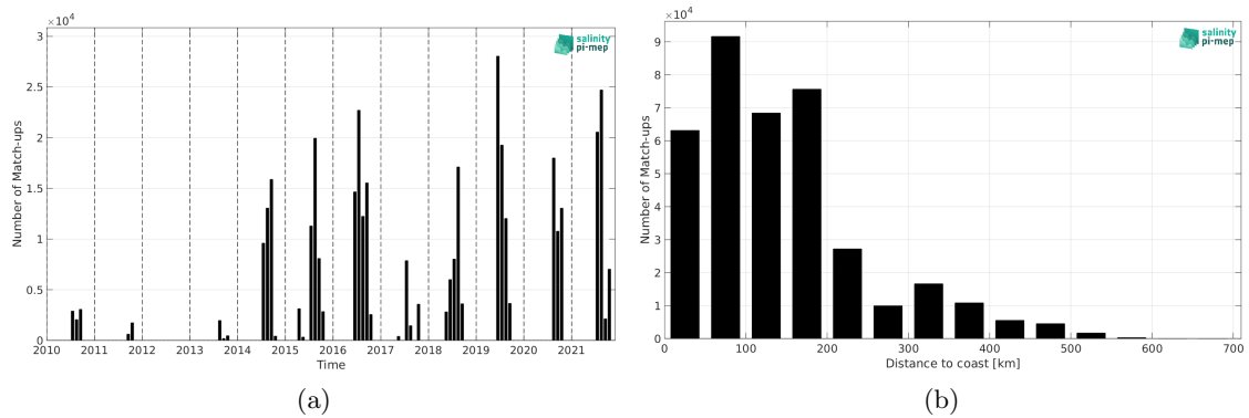
Figure 1: Number of match-ups between TSG (Amundsen) and SMOS SSS L3 Arctic v2 - 18 Days (CATDS-CEC-LOCEAN) SSS as a function of time (a) and as function of the distance to coast (b) over the Global Ocean Pi-MEP region and for the full satellite product period.
