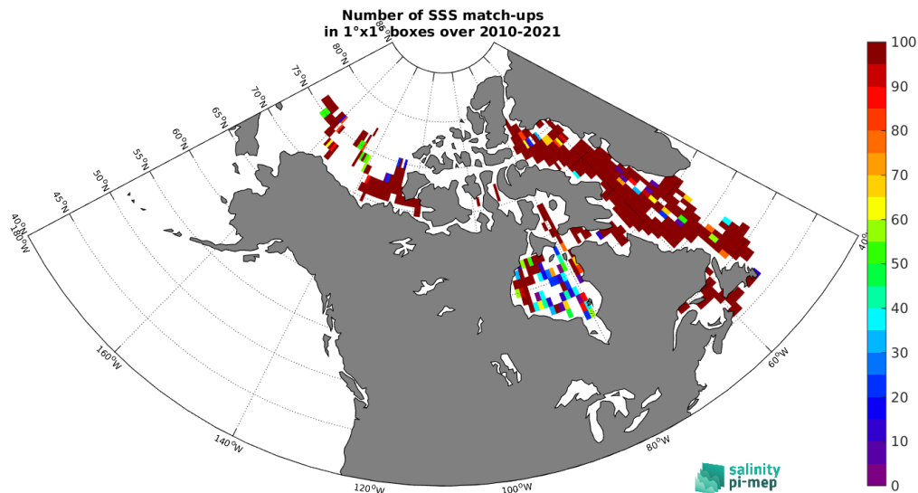
Figure 4: Number of SSS match-ups between TSG (Amundsen) SSS and the SMOS SSS L3 Arctic v2 - 18 Days (CATDS-CEC-LOCEAN) SSS product for the Global Ocean Pi-MEP region over 1^\circ \times 1^\circ boxes and for the full satellite product period.
