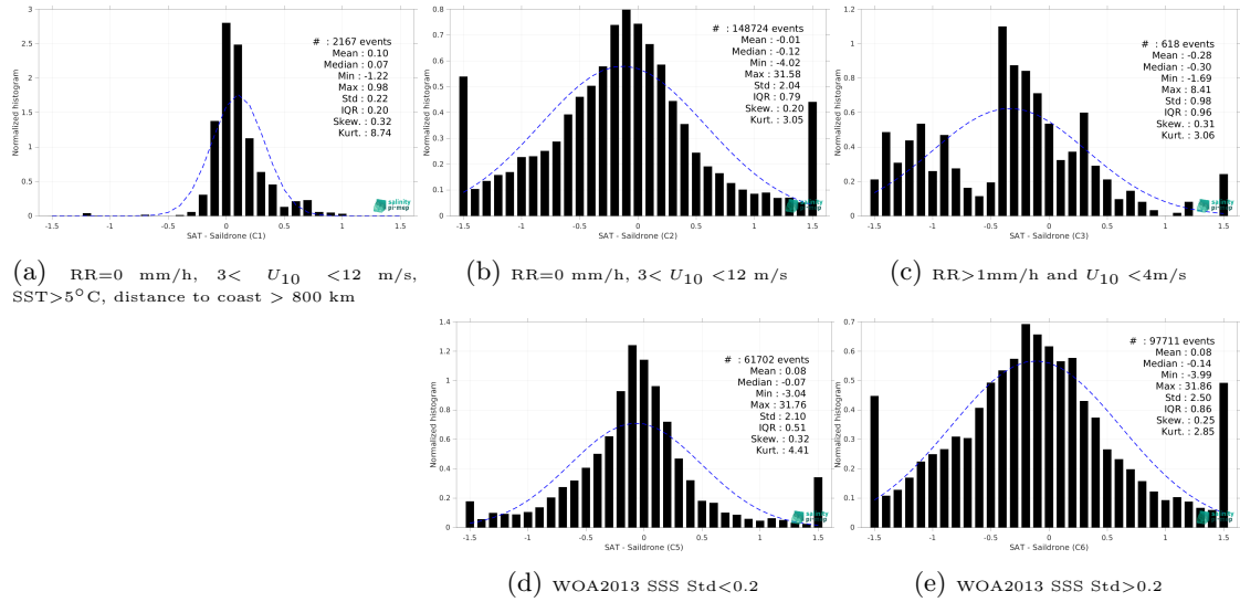
Figure 15: Normalized histogram of \Delta SSS (SMOS SSS L3 Arctic v2 - 18 Days (CATDS-CEC-LOCEAN) - Sailldrone) for 5 different subdatasets corresponding to: RR=0 mm/h, 3 < U_{10} < 12 m/s, SST > 5°C, distance to coast > 800 km (a), RR=0 mm/h, 3 < U_{10} < 12 m/s (b), RR > 1mm/h and U_{10} < 4 m/s (c), WOA2013 SSS Std < 0.2 (d), WOA2013 SSS Std > 0.2 (e).
