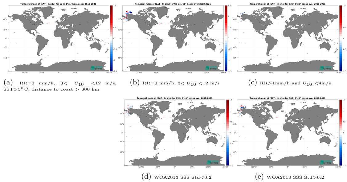
Figure 14: Temporal mean gridded over spatial boxes of size 1^\circ \times 1^\circ of \Delta SSS (SMOS SSS L3 Arctic v2 - 18 Days (CATDS-CEC-LOCEAN) - Sairdrone) for 5 different subdatasets corresponding to:RR=0 mm/h, 3 < U_{10} < 12 m/s, SST > 5^\circ\text{C} , distance to coast > 800 km (a), RR=0 mm/h, 3 < U_{10} < 12 m/s (b), RR > 1 mm/h and U_{10} < 4 m/s (c), WOA2013 SSS Std < 0.2 (d), WOA2013 SSS Std > 0.2 (e).
