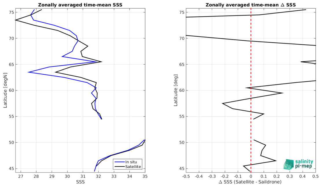
Figure 8: Left panel: Zonal mean SSS from SMOS SSS L3 Arctic v2 - 18 Days (CATDS-CEC-LOCEAN) satellite product (black) and from Sairdrone (blue). Right panel: Zonal mean of \Delta SSS (Satellite - Sairdrone) for all the collected Pi-MEP match-up pairs estimated over the full satellite product period.
