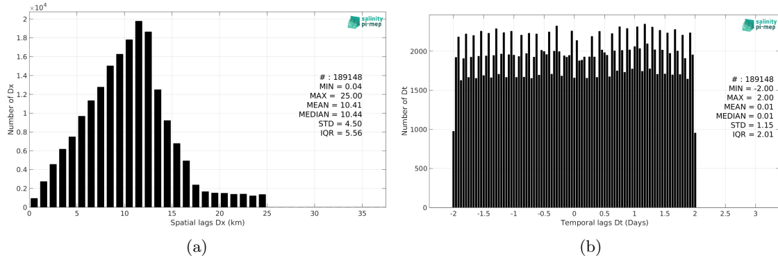
Figure 5: Histograms of the spatial (a) and temporal (b) lags between the location/time of the Saildrone measurement and the date of the corresponding SMOS SSS L3 Arctic v2 - 18 Days (CATDS-CEC-LOCEAN) SSS pixel.
