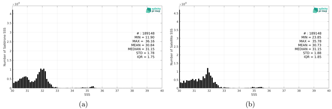
Figure 2: Histograms of SSS from Saildrone (a) and SMOS SSS L3 Arctic v2 - 18 Days (CATDS-CEC-LOCEAN) (b) considering all match-up pairs per bins of 0.1 over the Global Ocean Pi-MEP region and for the full satellite product period.
