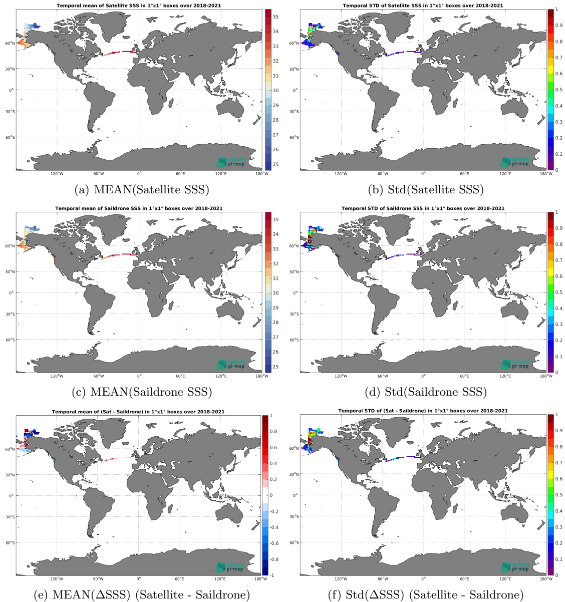
Figure 6: Temporal mean (left) and Std (right) of SSS from SMOS SSS L3 Arctic v2 - 18 Days (CATDS-CEC-LOCEAN) (top), Saildrone (middle), and of \Delta SSS (Satellite - Saildrone). Only match-up pairs are used to generate these maps.
