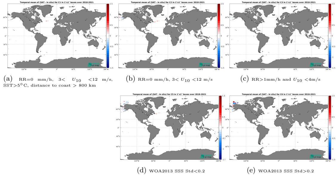
Figure 12: Temporal mean gridded over spatial boxes of size 1^{\circ}\times 1^{\circ} of \Delta\text{SSS} (SMOS SSS L3 Arctic v2 - 18 Days (CATDS-CEC-LOCEAN) - Sailydrone) for 5 different subdatasets corresponding to:RR=0 mm/h, 3 < U_{10} < 12 m/s, SST >5^{\circ}\text{C} , distance to coast > 800 km (a), RR=0 mm/h, 3 < U_{10} < 12 m/s (b), RR >1 mm/h and U_{10} < 4 m/s (c), WOA2013 SSS Std <0.2 (d), WOA2013 SSS Std >0.2 (e).
