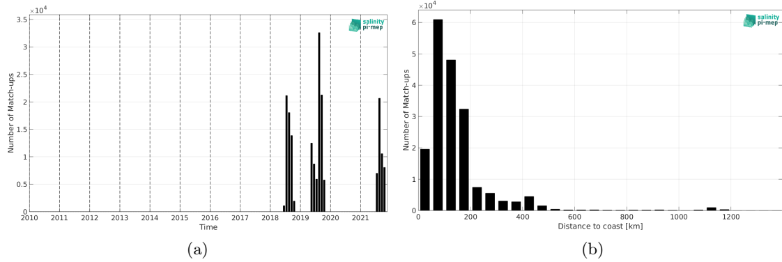
Figure 1: Number of match-ups between Saildrone and SMOS SSS L3 Arctic v2 - 18 Days (CATDS-CEC-LOCEAN) SSS as a function of time (a) and as function of the distance to coast (b) over the Global Ocean Pi-MEP region and for the full satellite product period.
