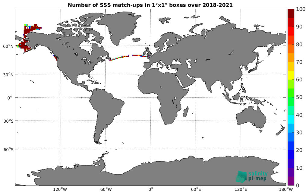
Figure 4: Number of SSS match-ups between Saildrone SSS and the SMOS SSS L3 Arctic v2 - 18 Days (CATDS-CEC-LOCEAN) SSS product for the Global Ocean Pi-MEP region over 1^\circ \times 1^\circ boxes and for the full satellite product period.
