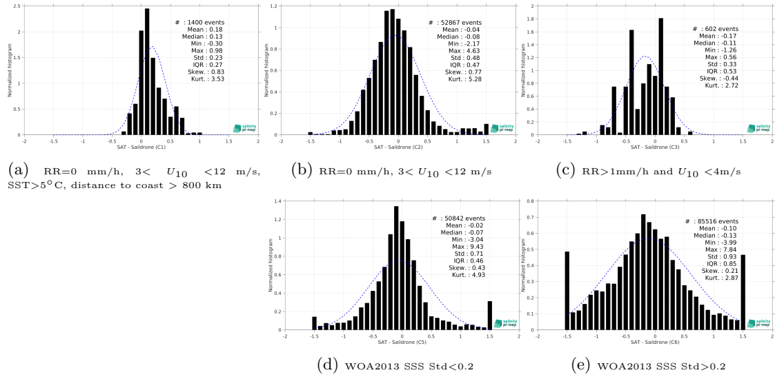
Figure 13: Normalized histogram of \Delta SSS (SMOS SSS L3 Arctic v2 - 18 Days (CATDS-CEC-LOCEAN) - Saildrone) for 5 different subdatasets corresponding to: RR=0 mm/h, 3 < U_{10} < 12 m/s, SST>5°C, distance to coast > 800 km (a), RR=0 mm/h, 3 < U_{10} < 12 m/s (b), RR>1mm/h and U_{10} < 4 m/s (c), WOA2013 SSS Std<0.2 (d), WOA2013 SSS Std>0.2 (e).
