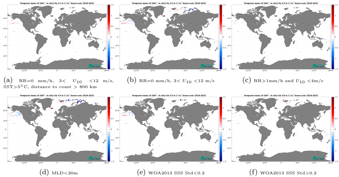
Figure 14: Temporal mean gridded over spatial boxes of size 1^\circ \times 1^\circ of \Delta SSS (SMOS SSS L3 Arctic v2 - 18 Days (CATDS-CEC-LOCEAN) - Marine mammals) for 6 different subdatasets corresponding to:RR=0 mm/h, 3 < U_{10} < 12 m/s, SST >5^\circ C, distance to coast > 800 km (a), RR=0 mm/h, 3 < U_{10} < 12 m/s (b), RR >1 mm/h and U_{10} < 4 m/s (c),MLD <20 m (d),WOA2013 SSS Std <0.2 (e),WOA2013 SSS Std >0.2 (f).
