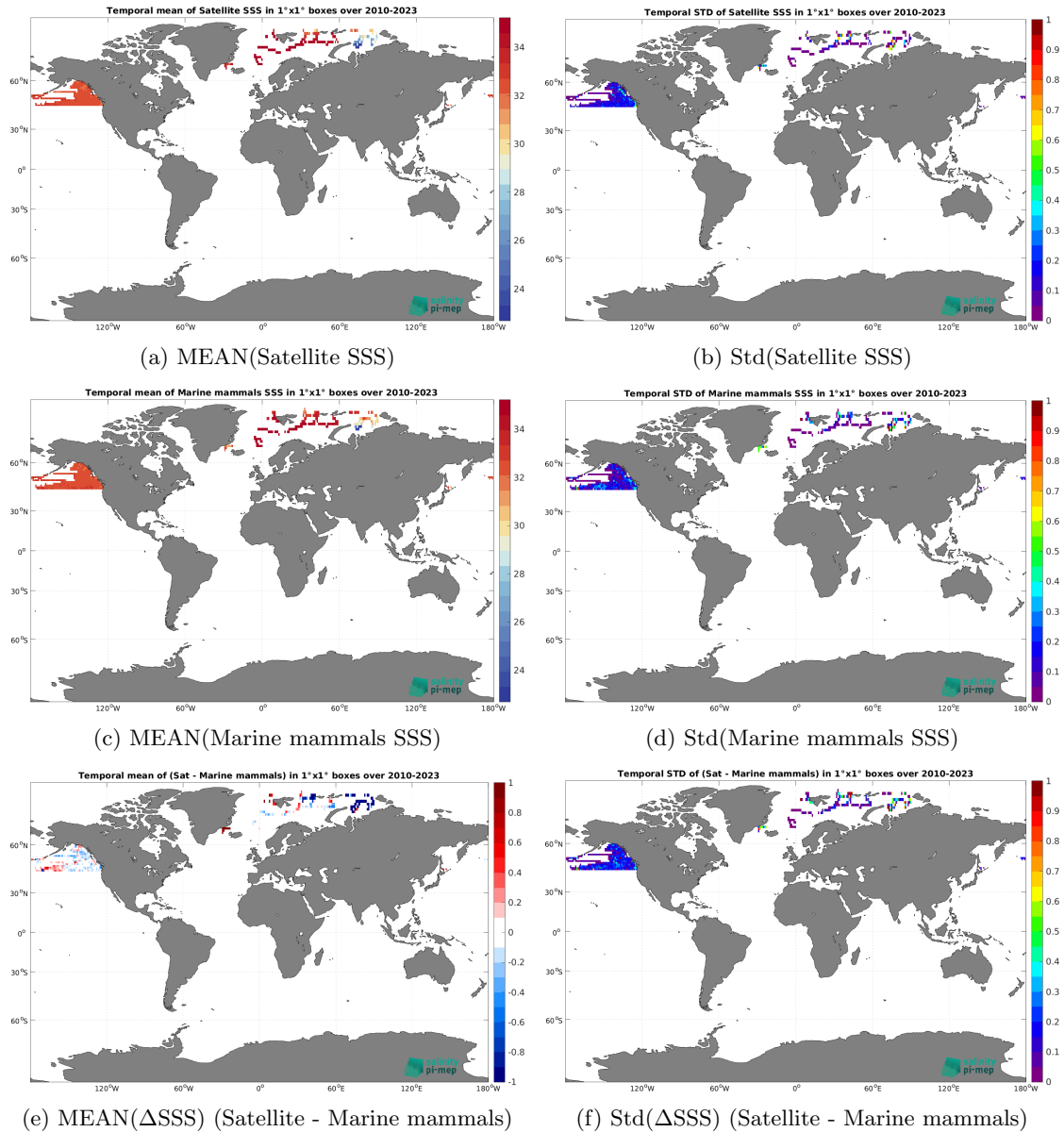
Figure 7: Temporal mean (left) and Std (right) of SSS from SMOS SSS L3 Arctic v2 - 18 Days (CATDS-CEC-LOCEAN) (top), Marine mammals (middle), and of \Delta SSS (Satellite - Marine mammals). Only match-up pairs are used to generate these maps.
