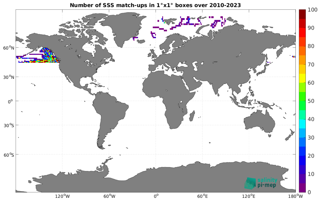
Figure 5: Number of SSS match-ups between Marine mammals SSS and the SMOS SSS L3 Arctic v2 - 18 Days (CATDS-CEC-LOCEAN) SSS product for the Global Ocean Pi-MEP region over 1^\circ \times 1^\circ boxes and for the full satellite product period.
