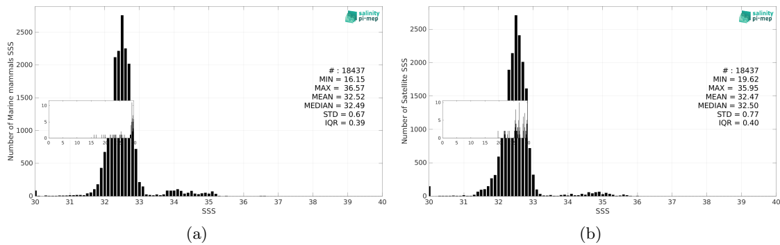
Figure 3: Histograms of SSS from Marine mammals (a) and SMOS SSS L3 Arctic v2 - 18 Days (CATDS-CEC-LOCEAN) (b) considering all match-up pairs per bins of 0.1 over the Global Ocean Pi-MEP region and for the full satellite product period.
