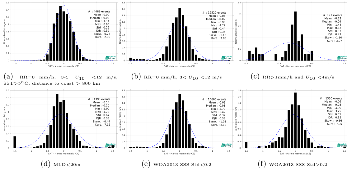
Figure 15: Normalized histogram of \Delta SSS (SMOS SSS L3 Arctic v2 - 18 Days (CATDS-CEC-LOCEAN) - Marine mammals) for 6 different subdatasets corresponding to: RR=0 mm/h, 3 < U_{10} < 12 m/s, SST > 5°C, distance to coast > 800 km (a), RR=0 mm/h, 3 < U_{10} < 12 m/s (b), RR > 1mm/h and U_{10} < 4 m/s (c), MLD < 20m (d), WOA2013 SSS Std < 0.2 (e), WOA2013 SSS Std > 0.2 (f).
