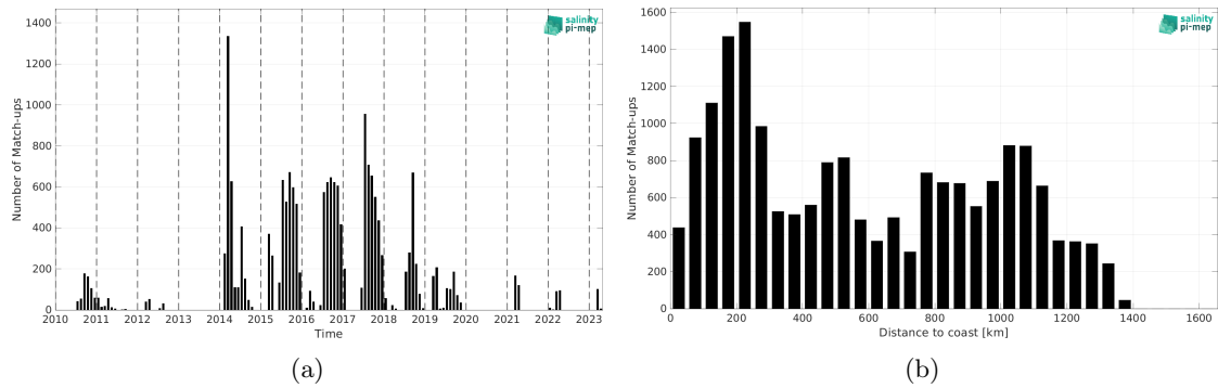
Figure 2: Number of match-ups between Marine mammals and SMOS SSS L3 Arctic v2 - 18 Days (CATDS-CEC-LOCEAN) SSS as a function of time (a) and as function of the distance to coast (b) over the Global Ocean Pi-MEP region and for the full satellite product period.
