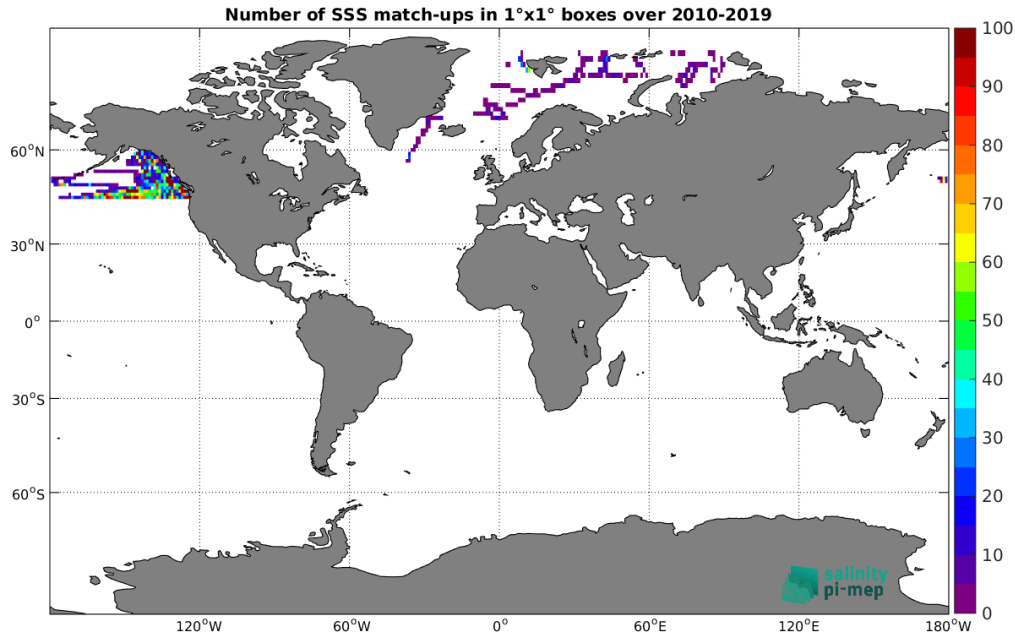
Figure 4: Number of SSS match-ups between Marine mammals SSS and the SMOS SSS L3 Arctic v2 - 18 Days (CATDS-CEC-LOCEAN) SSS product for the Global Ocean Pi-MEP region over 1^\circ \times 1^\circ boxes and for the full satellite product period.
