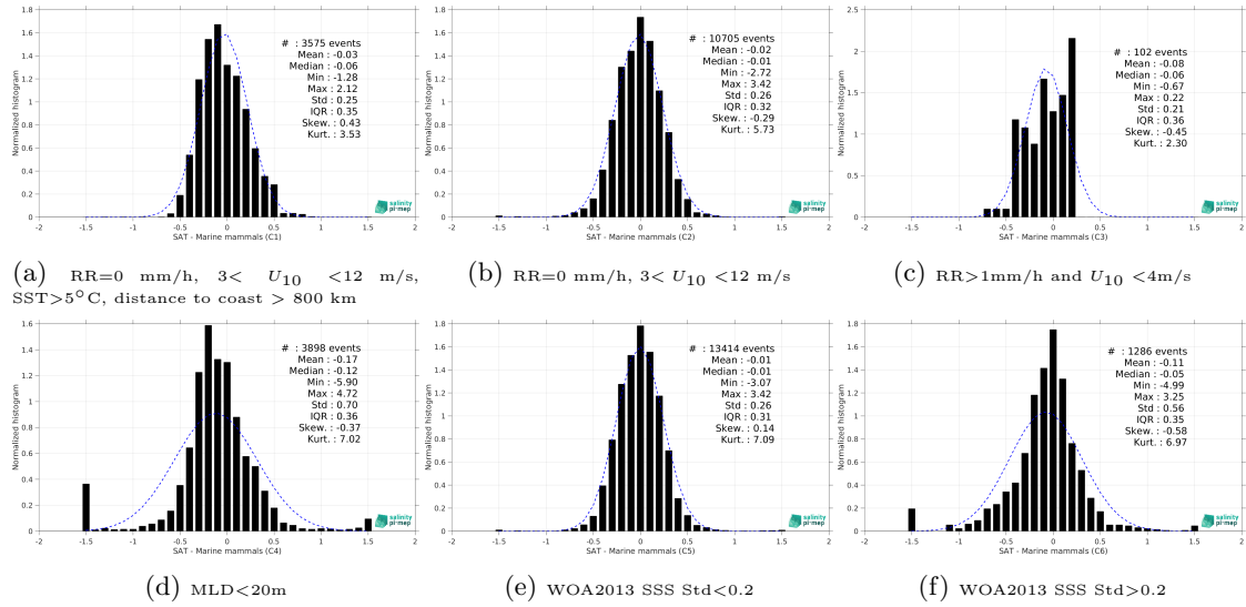
Figure 13: Normalized histogram of \Delta SSS (SMOS SSS L3 Arctic v2 - 18 Days (CATDS-CEC-LOCEAN) - Marine mammals) for 6 different subdatasets corresponding to: RR=0 mm/h, 3 < U_{10} < 12 m/s, SST > 5°C, distance to coast > 800 km (a), RR=0 mm/h, 3 < U_{10} < 12 m/s (b), RR > 1mm/h and U_{10} < 4 m/s (c), MLD < 20m (d), WOA2013 SSS Std < 0.2 (e), WOA2013 SSS Std > 0.2 (f).
