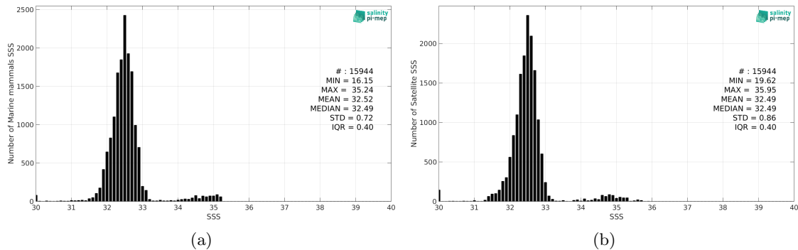
Figure 2: Histograms of SSS from Marine mammals (a) and SMOS SSS L3 Arctic v2 - 18 Days (CATDS-CEC-LOCEAN) (b) considering all match-up pairs per bins of 0.1 over the Global Ocean Pi-MEP region and for the full satellite product period.
