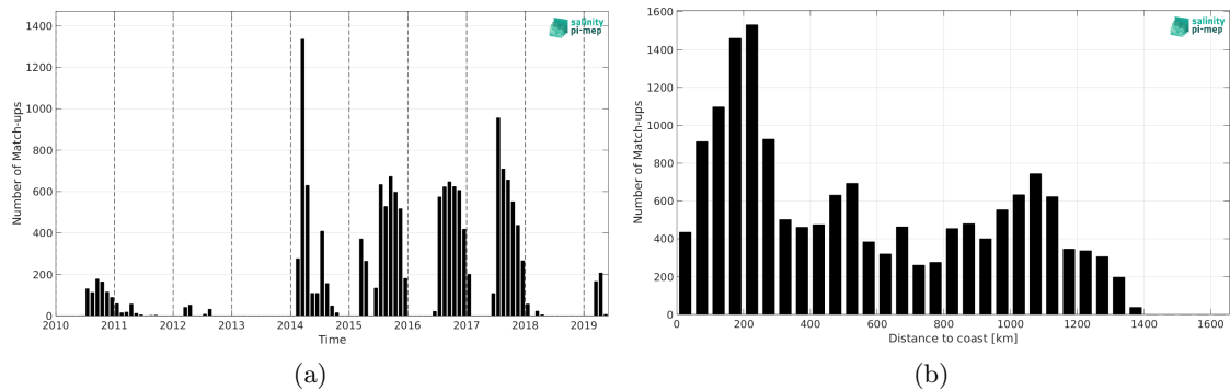
Figure 1: Number of match-ups between Marine mammals and SMOS SSS L3 Arctic v2 - 18 Days (CATDS-CEC-LOCEAN) SSS as a function of time (a) and as function of the distance to coast (b) over the Global Ocean Pi-MEP region and for the full satellite product period.
