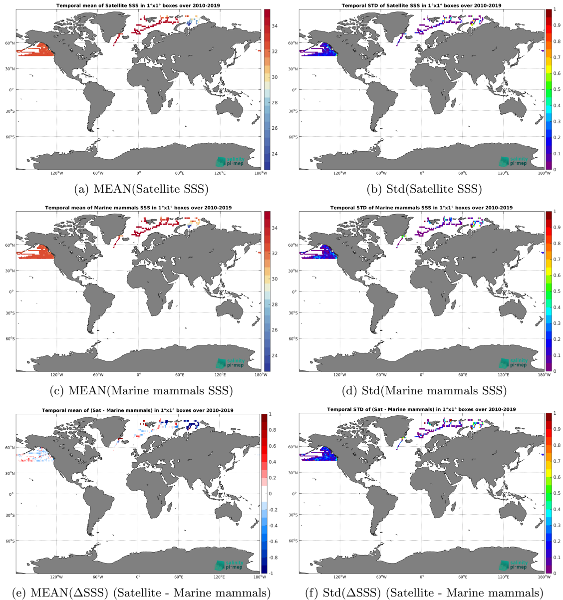
Figure 6: Temporal mean (left) and Std (right) of SSS from SMOS SSS L3 Arctic v2 - 18 Days (CATDS-CEC-LOCEAN) (top), Marine mammals (middle), and of \Delta SSS (Satellite - Marine mammals). Only match-up pairs are used to generate these maps.
