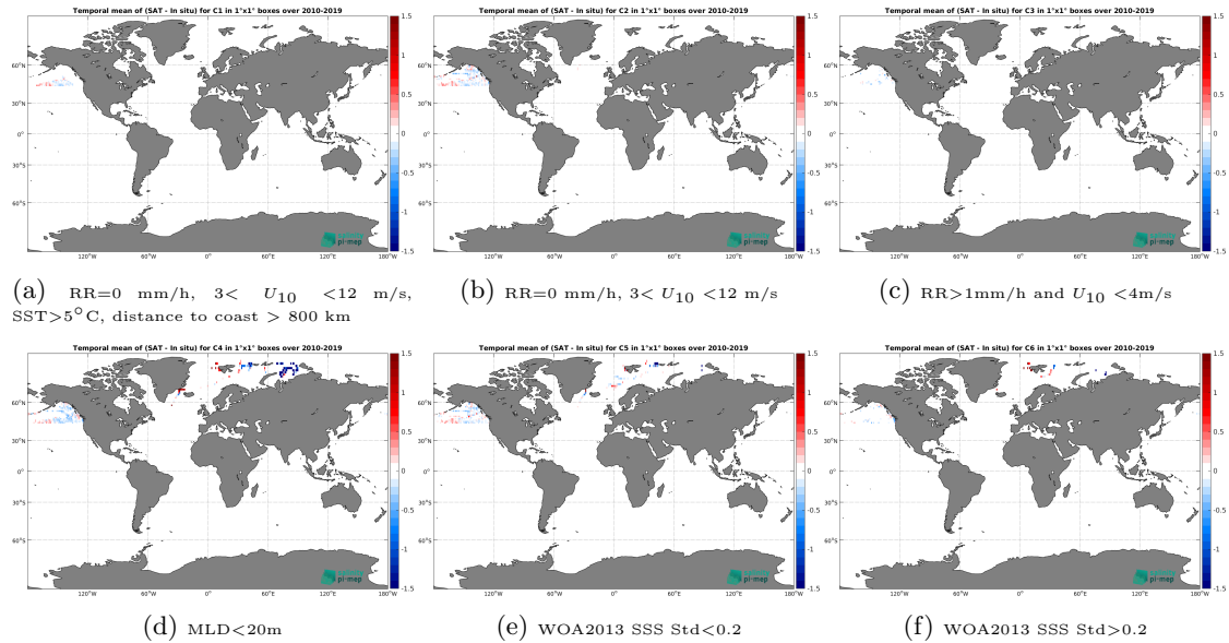
Figure 12: Temporal mean gridded over spatial boxes of size 1^{\circ}\times 1^{\circ} of \Delta\text{SSS} (SMOS SSS L3 Arctic v2 - 18 Days (CATDS-CEC-LOCEAN) - Marine mammals) for 6 different subdatasets corresponding to: RR=0 mm/h, 3 < U_{10} < 12 m/s, SST > 5^{\circ}\text{C} , distance to coast > 800 km (a), RR=0 mm/h, 3 < U_{10} < 12 m/s (b), RR > 1\text{mm/h} and U_{10} < 4\text{m/s} (c), MLD < 20\text{m} (d), WOA2013 SSS Std < 0.2 (e), WOA2013 SSS Std > 0.2 (f).
