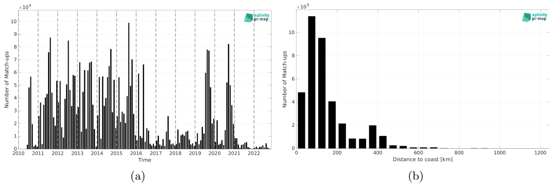
Figure 2: Number of match-ups between ICES and SMOS SSS L3 Arctic v2 - 18 Days (CATDS-CEC-LOCEAN) SSS as a function of time (a) and as function of the distance to coast (b) over the Global Ocean Pi-MEP region and for the full satellite product period.
