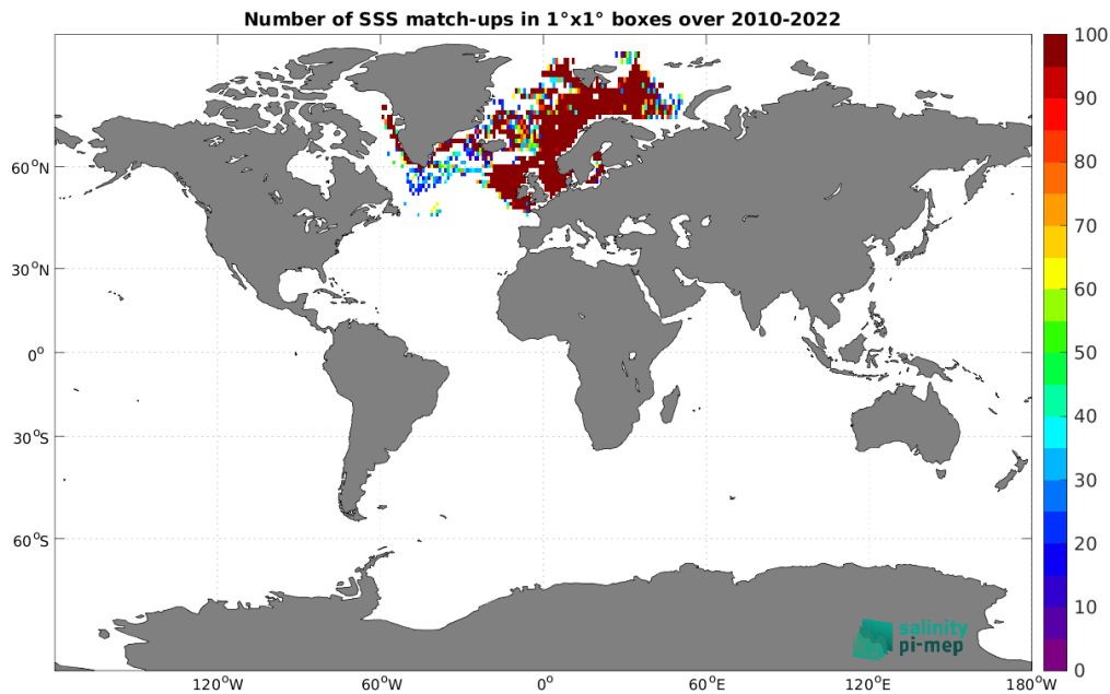
Figure 5: Number of SSS match-ups between ICES SSS and the SMOS SSS L3 Arctic v2 - 18 Days (CATDS-CEC-LOCEAN) SSS product for the Global Ocean Pi-MEP region over 1^\circ \times 1^\circ boxes and for the full satellite product period.
