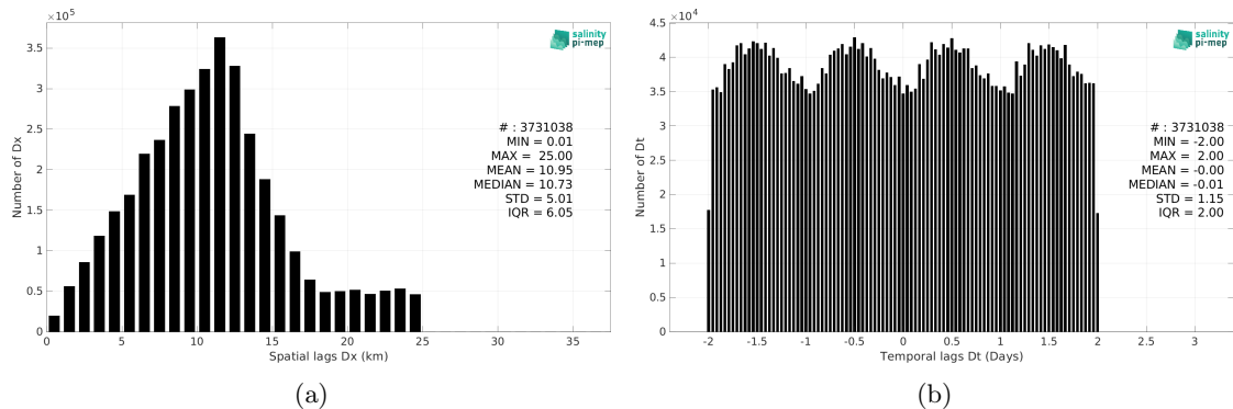
Figure 6: Histograms of the spatial (a) and temporal (b) lags between the location/time of the ICES measurement and the date of the corresponding SMOS SSS L3 Arctic v2 - 18 Days (CATDS-CEC-LOCEAN) SSS pixel.
