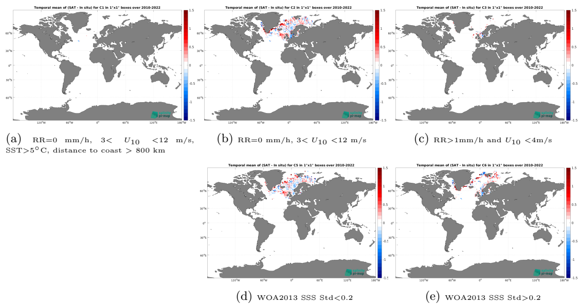
Figure 14: Temporal mean gridded over spatial boxes of size 1^\circ \times 1^\circ of \Delta SSS (SMOS SSS L3 Arctic v2 - 18 Days (CATDS-CEC-LOCEAN) - ICES) for 5 different subdatasets corresponding to: RR=0 mm/h, 3 < U_{10} < 12 m/s, SST > 5^\circ\text{C} , distance to coast > 800 km (a), RR=0 mm/h, 3 < U_{10} < 12 m/s (b), RR > 1 mm/h and U_{10} < 4 m/s (c), WOA2013 SSS Std < 0.2 (d), WOA2013 SSS Std > 0.2 (e).
