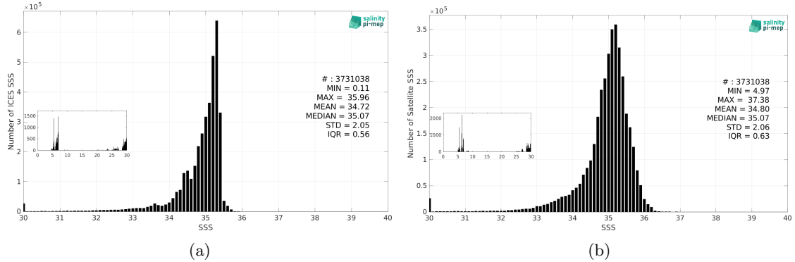
Figure 3: Histograms of SSS from ICES (a) and SMOS SSS L3 Arctic v2 - 18 Days (CATDS-CEC-LOCEAN) (b) considering all match-up pairs per bins of 0.1 over the Global Ocean Pi-MEP region and for the full satellite product period.
