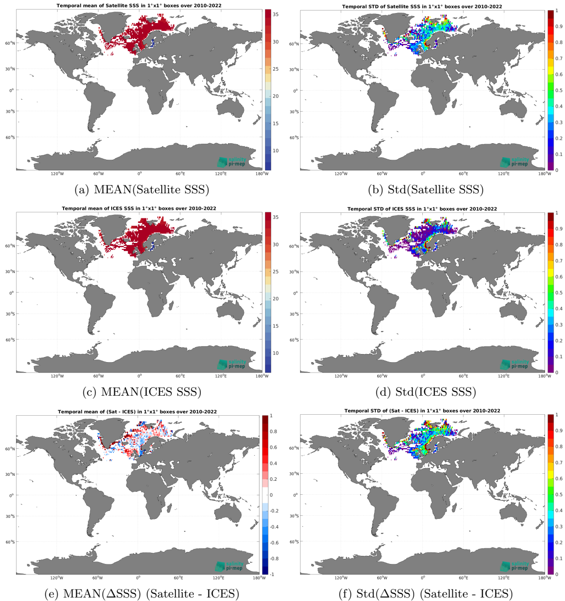
Figure 7: Temporal mean (left) and Std (right) of SSS from SMOS SSS L3 Arctic v2 - 18 Days (CATDS-CEC-LOCEAN) (top), ICES (middle), and of \Delta SSS (Satellite - ICES). Only match-up pairs are used to generate these maps.
