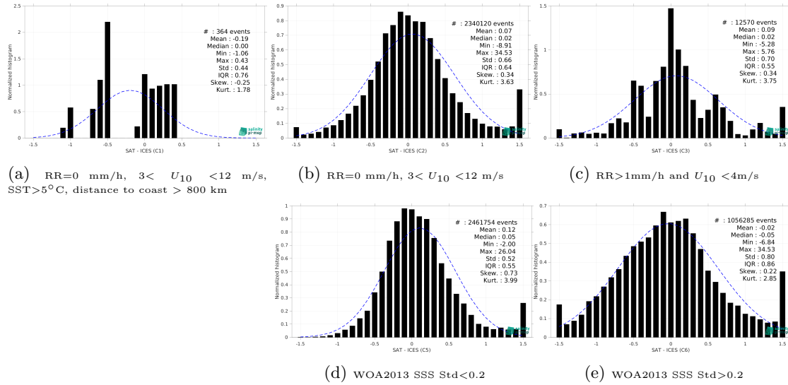
Figure 15: Normalized histogram of \Delta SSS (SMOS SSS L3 Arctic v2 - 18 Days (CATDS-CEC-LOCEAN) - ICES) for 5 different subdatasets corresponding to: RR=0 mm/h, 3 < U_{10} < 12 m/s, SST>5°C, distance to coast > 800 km (a), RR=0 mm/h, 3 < U_{10} < 12 m/s (b), RR>1mm/h and U_{10} < 4 m/s (c), WOA2013 SSS Std<0.2 (d), WOA2013 SSS Std>0.2 (e).
