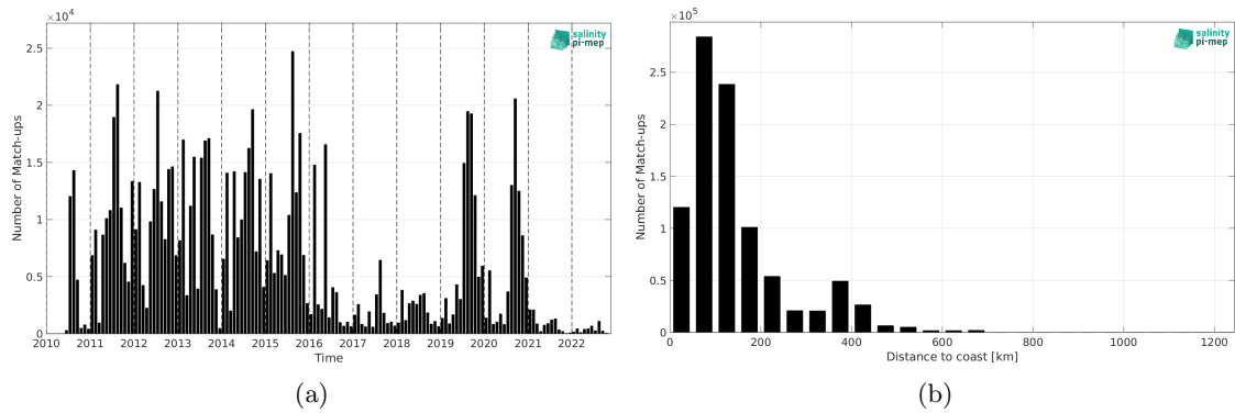
Figure 1: Number of match-ups between ICES and SMOS SSS L3 Arctic v2 - 18 Days (CATDS-CEC-LOCEAN) SSS as a function of time (a) and as function of the distance to coast (b) over the Global Ocean Pi-MEP region and for the full satellite product period.
