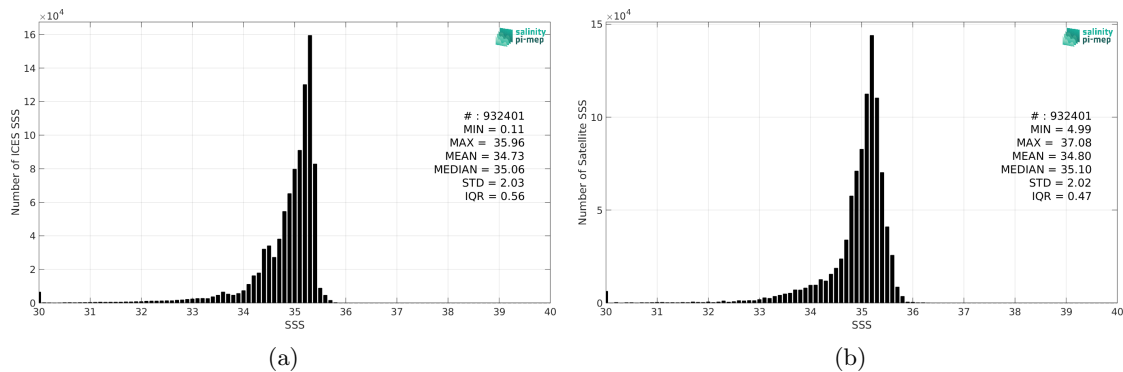
Figure 2: Histograms of SSS from ICES (a) and SMOS SSS L3 Arctic v2 - 18 Days (CATDS-CEC-LOCEAN) (b) considering all match-up pairs per bins of 0.1 over the Global Ocean Pi-MEP region and for the full satellite product period.
