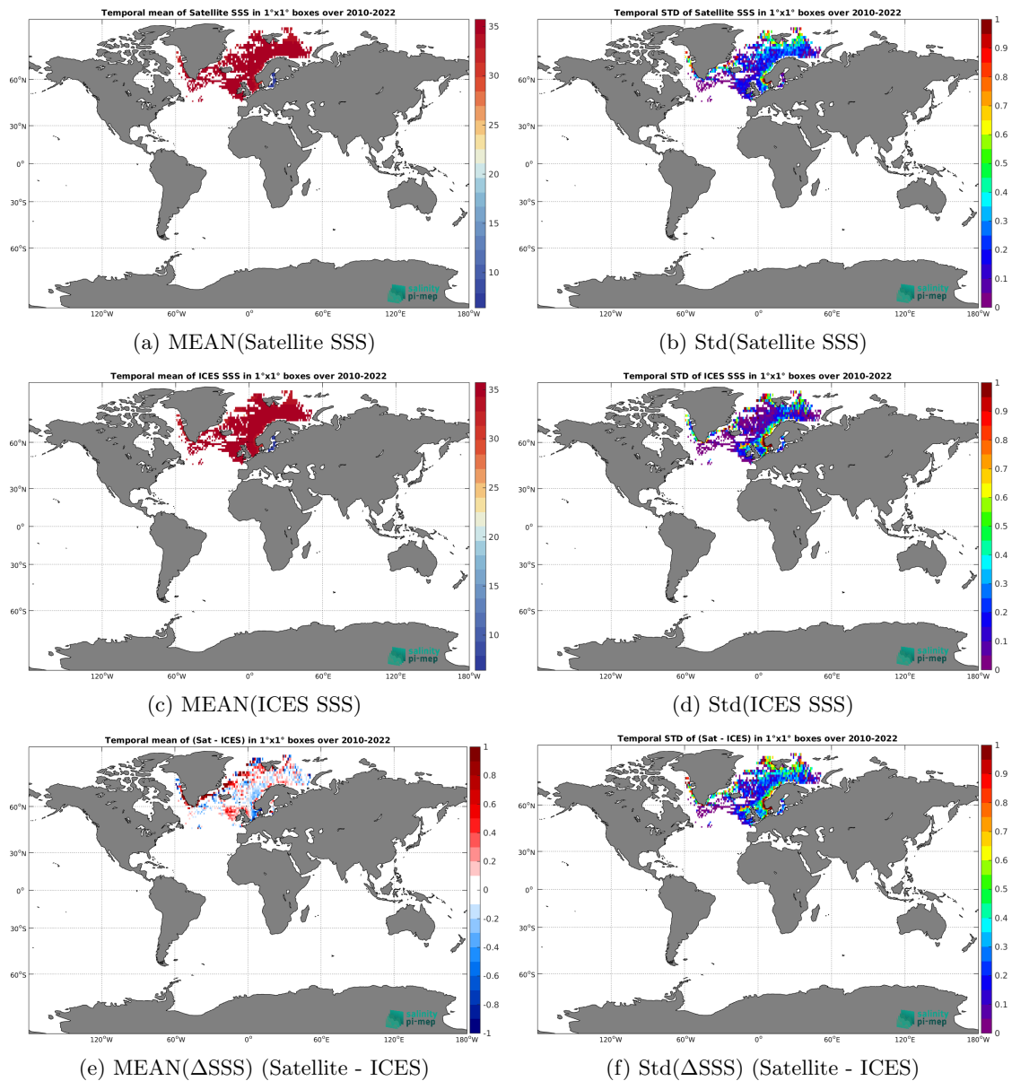
Figure 6: Temporal mean (left) and Std (right) of SSS from SMOS SSS L3 Arctic v2 - 18 Days (CATDS-CEC-LOCEAN) (top), ICES (middle), and of \Delta SSS (Satellite - ICES). Only match-up pairs are used to generate these maps.
