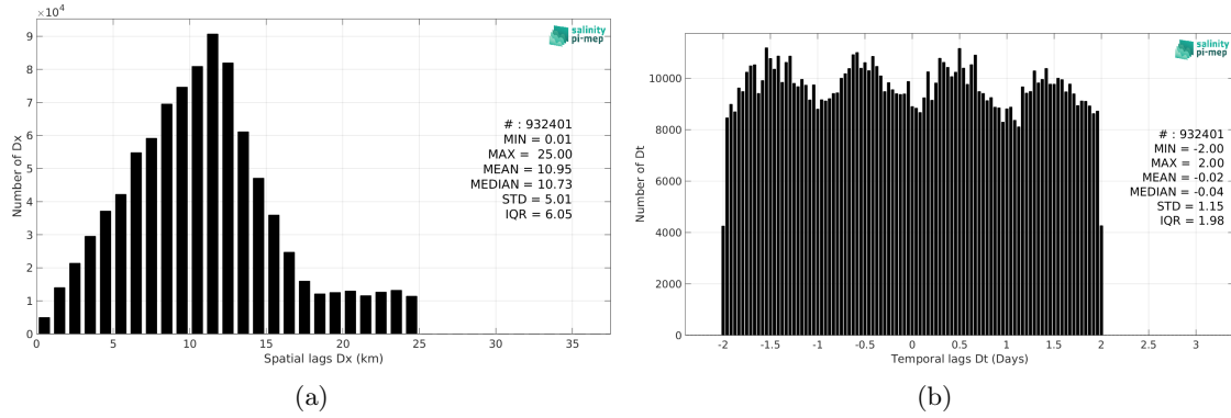
Figure 5: Histograms of the spatial (a) and temporal (b) lags between the location/time of the ICES measurement and the date of the corresponding SMOS SSS L3 Arctic v2 - 18 Days (CATDS-CEC-LOCEAN) SSS pixel.
