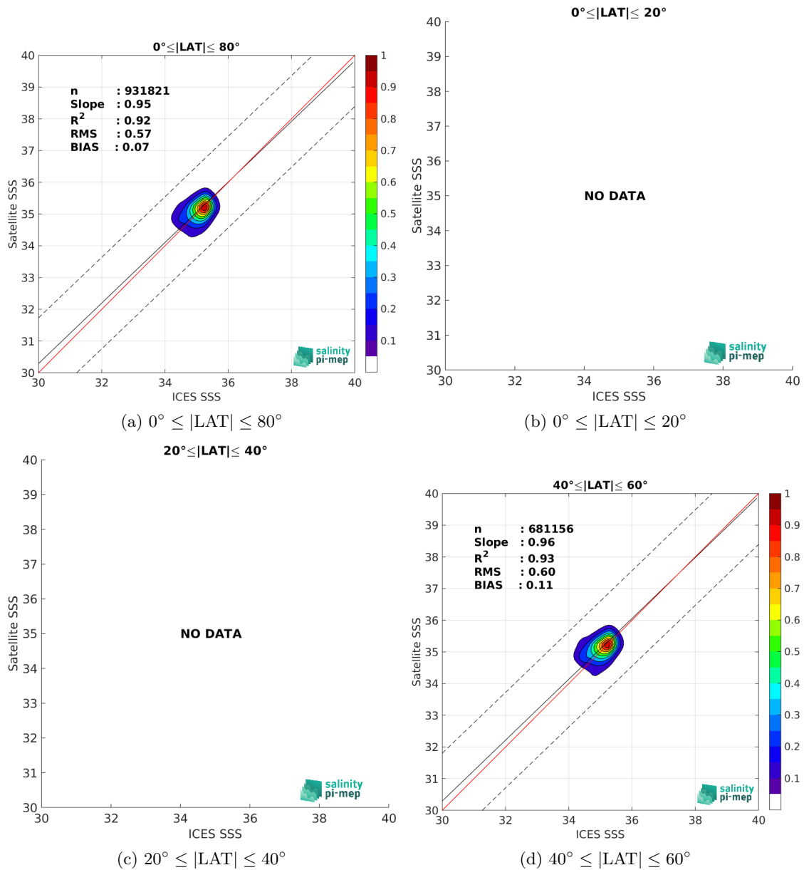
Figure 9: Contour maps of the concentration of SMOS SSS L3 Arctic v2 - 18 Days (CATDS-CEC-LOCEAN) SSS (y-axis) versus ICES SSS (x-axis) at match-up pairs for different latitude bands. For each plot, the red line shows x=y . The black thin and dashed lines indicate a linear fit through the data cloud and the \pm 95\% confidence levels, respectively. The number match-up pairs n , the slope and R^2 coefficient of the linear fit, the root mean square (RMS) and the mean bias between satellite and in situ data are indicated for each latitude band in each plots.
