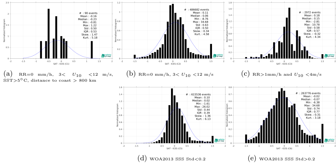
Figure 13: Normalized histogram of \Delta SSS (SMOS SSS L3 Arctic v2 - 18 Days (CATDS-CEC-LOCEAN) - ICES) for 5 different subdatasets corresponding to: RR=0 mm/h, 3 < U_{10} < 12 m/s, SST > 5°C, distance to coast > 800 km (a), RR=0 mm/h, 3 < U_{10} < 12 m/s (b), RR > 1mm/h and U_{10} < 4 m/s (c), WOA2013 SSS Std < 0.2 (d), WOA2013 SSS Std > 0.2 (e).
