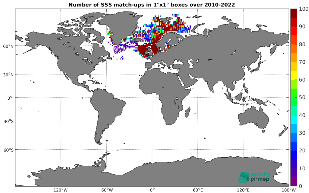
Figure 4: Number of SSS match-ups between ICES SSS and the SMOS SSS L3 Arctic v2 - 18 Days (CATDS-CEC-LOCEAN) SSS product for the Global Ocean Pi-MEP region over 1^\circ \times 1^\circ boxes and for the full satellite product period.
