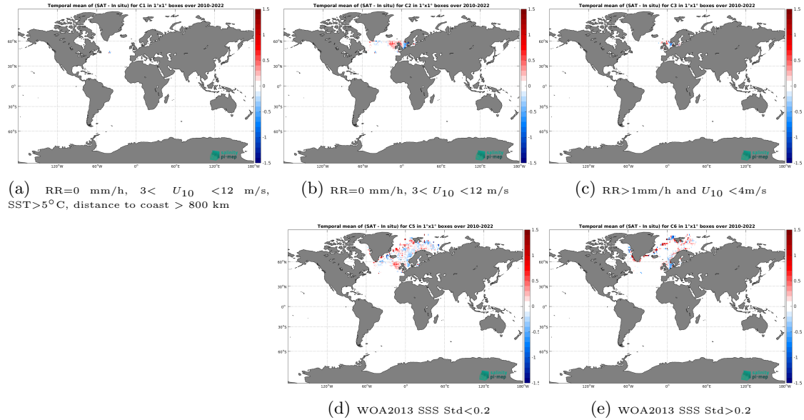
Figure 12: Temporal mean gridded over spatial boxes of size 1^{\circ}\times 1^{\circ} of \Delta\text{SSS} (SMOS SSS L3 Arctic v2 - 18 Days (CATDS-CEC-LOCEAN) - ICES) for 5 different subdatasets corresponding to:RR=0 mm/h, 3 < U_{10} < 12 m/s, SST >5^{\circ}\text{C} , distance to coast > 800 km (a), RR=0 mm/h, 3 < U_{10} < 12 m/s (b), RR >1 mm/h and U_{10} < 4 m/s (c), WOA2013 SSS Std <0.2 (d), WOA2013 SSS Std >0.2 (e).
