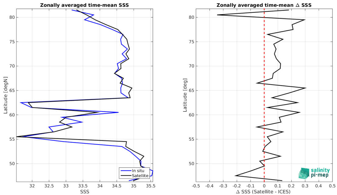
Figure 8: Left panel: Zonal mean SSS from SMOS SSS L3 Arctic v2 - 18 Days (CATDS-CEC-LOCEAN) satellite product (black) and from ICES (blue). Right panel: Zonal mean of \Delta SSS (Satellite - ICES) for all the collected Pi-MEP match-up pairs estimated over the full satellite product period.
