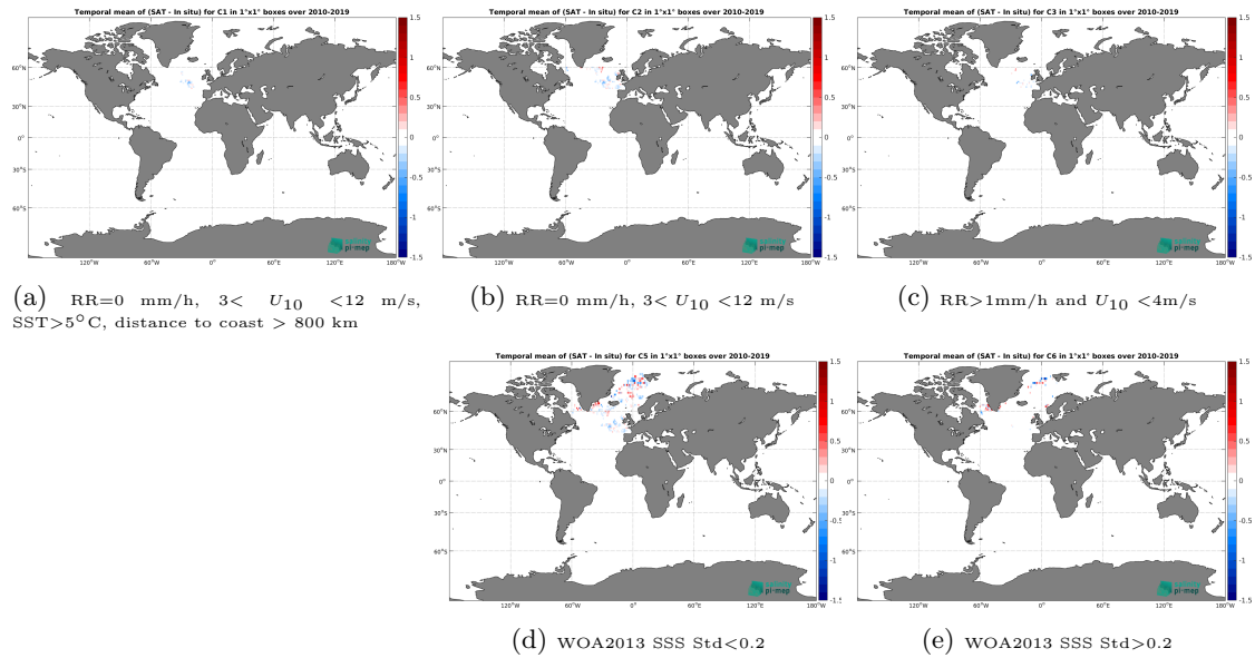
Figure 11: Temporal mean gridded over spatial boxes of size 1^{\circ}\times 1^{\circ} of \Delta\text{SSS} (SMOS SSS L3 Arctic v2 - 18 Days (CATDS-CEC-LOCEAN) - Surface drifters) for 5 different subdatasets corresponding to:RR=0 mm/h, 3 < U_{10} < 12 m/s, SST >5^{\circ}\text{C} , distance to coast > 800 km (a), RR=0 mm/h, 3 < U_{10} < 12 m/s (b), RR >1 mm/h and U_{10} < 4 m/s (c), WOA2013 SSS Std <0.2 (d), WOA2013 SSS Std >0.2 (e).
