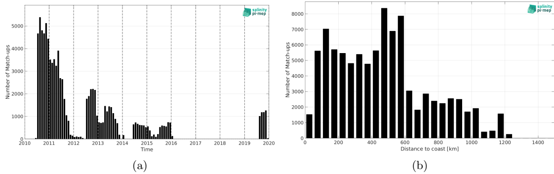
Figure 1: Number of match-ups between Surface drifters and SMOS SSS L3 Arctic v2 - 18 Days (CATDS-CEC-LOCEAN) SSS as a function of time (a) and as function of the distance to coast (b) over the Global Ocean Pi-MEP region and for the full satellite product period.
