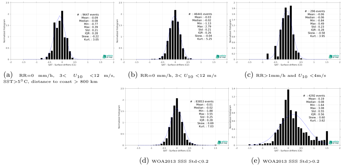
Figure 12: Normalized histogram of \Delta SSS (SMOS SSS L3 Arctic v2 - 18 Days (CATDS-CEC-LOCEAN) - Surface drifters) for 5 different subdatasets corresponding to: RR=0 mm/h, 3 < U_{10} < 12 m/s, SST>5°C, distance to coast > 800 km (a), RR=0 mm/h, 3 < U_{10} < 12 m/s (b), RR>1mm/h and U_{10} < 4 m/s (c), WOA2013 SSS Std<0.2 (d), WOA2013 SSS Std>0.2 (e).
