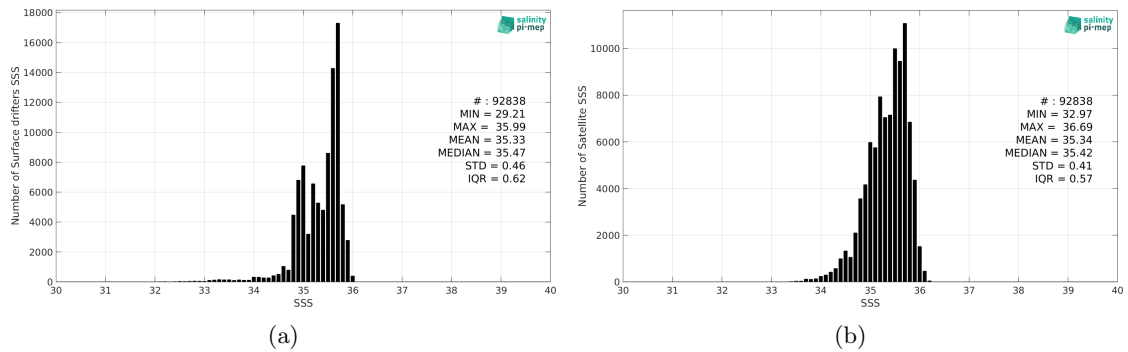
Figure 2: Histograms of SSS from Surface drifters (a) and SMOS SSS L3 Arctic v2 - 18 Days (CATDS-CEC-LOCEAN) (b) considering all match-up pairs per bins of 0.1 over the Global Ocean Pi-MEP region and for the full satellite product period.
