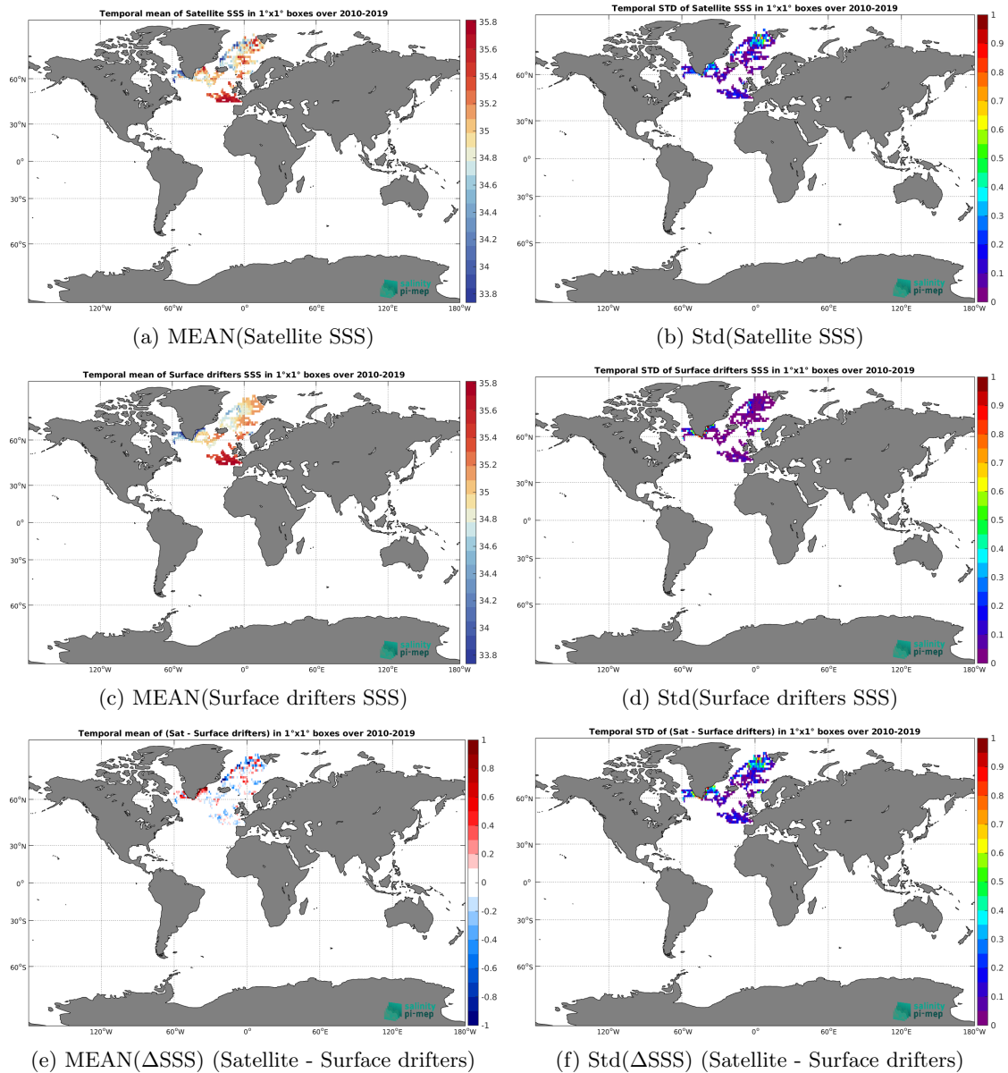
Figure 5: Temporal mean (left) and Std (right) of SSS from SMOS SSS L3 Arctic v2 - 18 Days (CATDS-CEC-LOCEAN) (top), Surface drifters (middle), and of \Delta SSS (Satellite - Surface drifters). Only match-up pairs are used to generate these maps.
