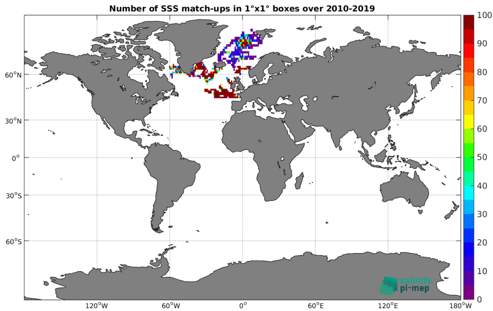
Figure 3: Number of SSS match-ups between Surface drifters SSS and the SMOS SSS L3 Arctic v2 - 18 Days (CATDS-CEC-LOCEAN) SSS product for the Global Ocean Pi-MEP region over 1^\circ \times 1^\circ boxes and for the full satellite product period.
