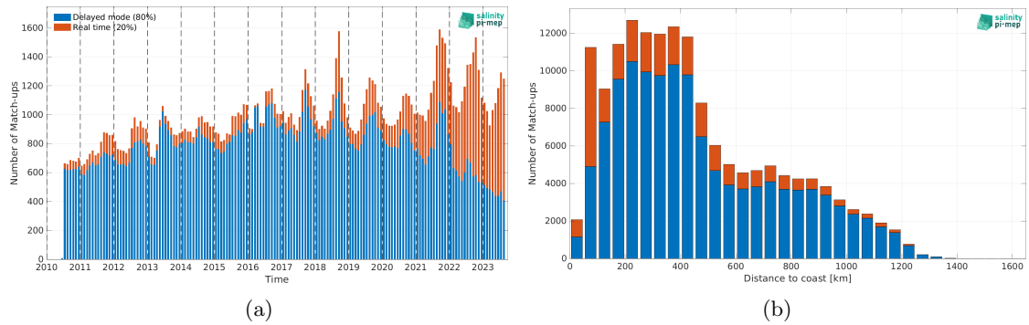
Figure 2: Number of match-ups between Argo and SMOS SSS L3 Arctic v2 - 18 Days (CATDS-CEC-LOCEAN) SSS as a function of time (a) and as function of the distance to coast (b) over the Global Ocean Pi-MEP region and for the full satellite product period.
