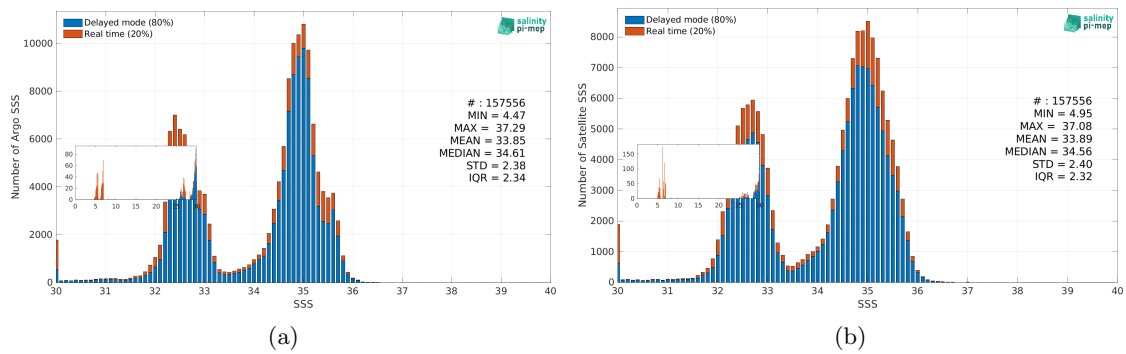
Figure 3: Histograms of SSS from Argo (a) and SMOS SSS L3 Arctic v2 - 18 Days (CATDS-CEC-LOCEAN) (b) considering all match-up pairs per bins of 0.1 over the Global Ocean Pi-MEP region and for the full satellite product period.
