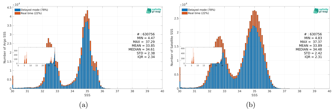
Figure 3: Histograms of SSS from Argo (a) and SMOS SSS L3 Arctic v2 - 18 Days (CATDS-CEC-LOCEAN) (b) considering all match-up pairs per bins of 0.1 over the Global Ocean Pi-MEP region and for the full satellite product period.
