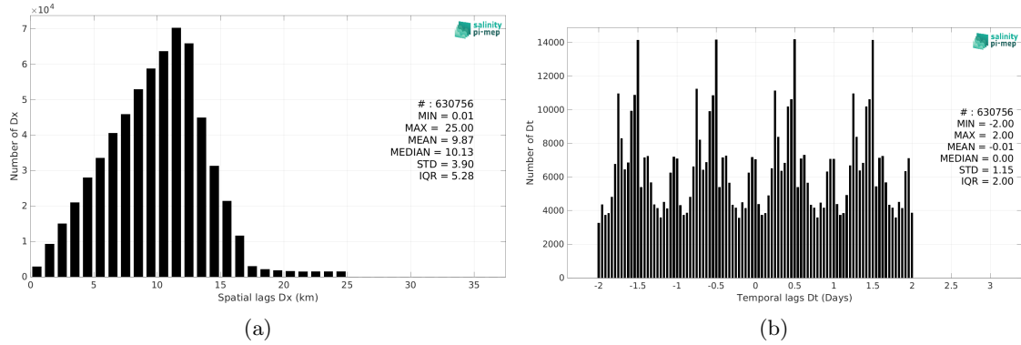
Figure 6: Histograms of the spatial (a) and temporal (b) lags between the location/time of the Argo measurement and the date of the corresponding SMOS SSS L3 Arctic v2 - 18 Days (CATDS-CEC-LOCEAN) SSS pixel.
