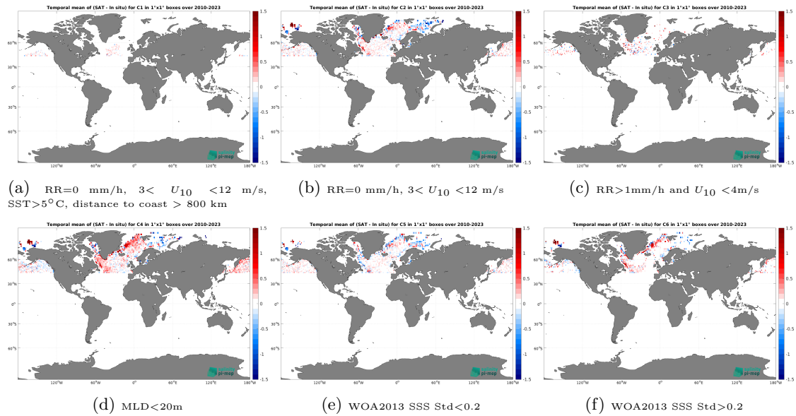
Figure 14: Temporal mean gridded over spatial boxes of size 1^\circ \times 1^\circ of \Delta SSS (SMOS SSS L3 Arctic v2 - 18 Days (CATDS-CEC-LOCEAN) - Argo) for 6 different subdatasets corresponding to:RR=0 mm/h, 3 < U_{10} < 12 m/s, SST>5°C, distance to coast > 800 km (a), RR=0 mm/h, 3 < U_{10} < 12 m/s (b), RR>1mm/h and U_{10} < 4 m/s (c),MLD<20m (d),WOA2013 SSS Std<0.2 (e),WOA2013 SSS Std>0.2 (f).
