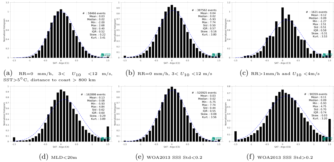
Figure 15: Normalized histogram of \Delta SSS (SMOS SSS L3 Arctic v2 - 18 Days (CATDS-CEC-LOCEAN) - Argo) for 6 different subdatasets corresponding to: RR=0 mm/h, 3 < U_{10} < 12 m/s, SST>5°C, distance to coast > 800 km (a), RR=0 mm/h, 3 < U_{10} < 12 m/s (b), RR>1mm/h and U_{10} < 4 m/s (c), MLD<20m (d), WOA2013 SSS Std<0.2 (e), WOA2013 SSS Std>0.2 (f).
