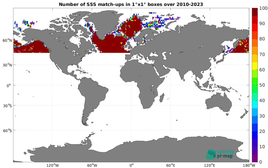
Figure 5: Number of SSS match-ups between Argo SSS and the SMOS SSS L3 Arctic v2 - 18 Days (CATDS-CEC-LOCEAN) SSS product for the Global Ocean Pi-MEP region over 1^\circ \times 1^\circ boxes and for the full satellite product period.
