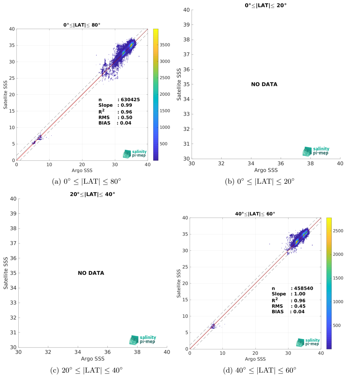
Figure 10: Contour maps of the concentration of SMOS SSS L3 Arctic v2 - 18 Days (CATDS-CEC-LOCEAN) SSS (y-axis) versus Argo SSS (x-axis) at match-up pairs for different latitude bands. For each plot, the red line shows x=y . The black thin and dashed lines indicate a linear fit through the data cloud and the \pm 95\% confidence levels, respectively. The number match-up pairs n , the slope and R^2 coefficient of the linear fit, the root mean square (RMS) and the mean bias between satellite and in situ data are indicated for each latitude band in each plots.
