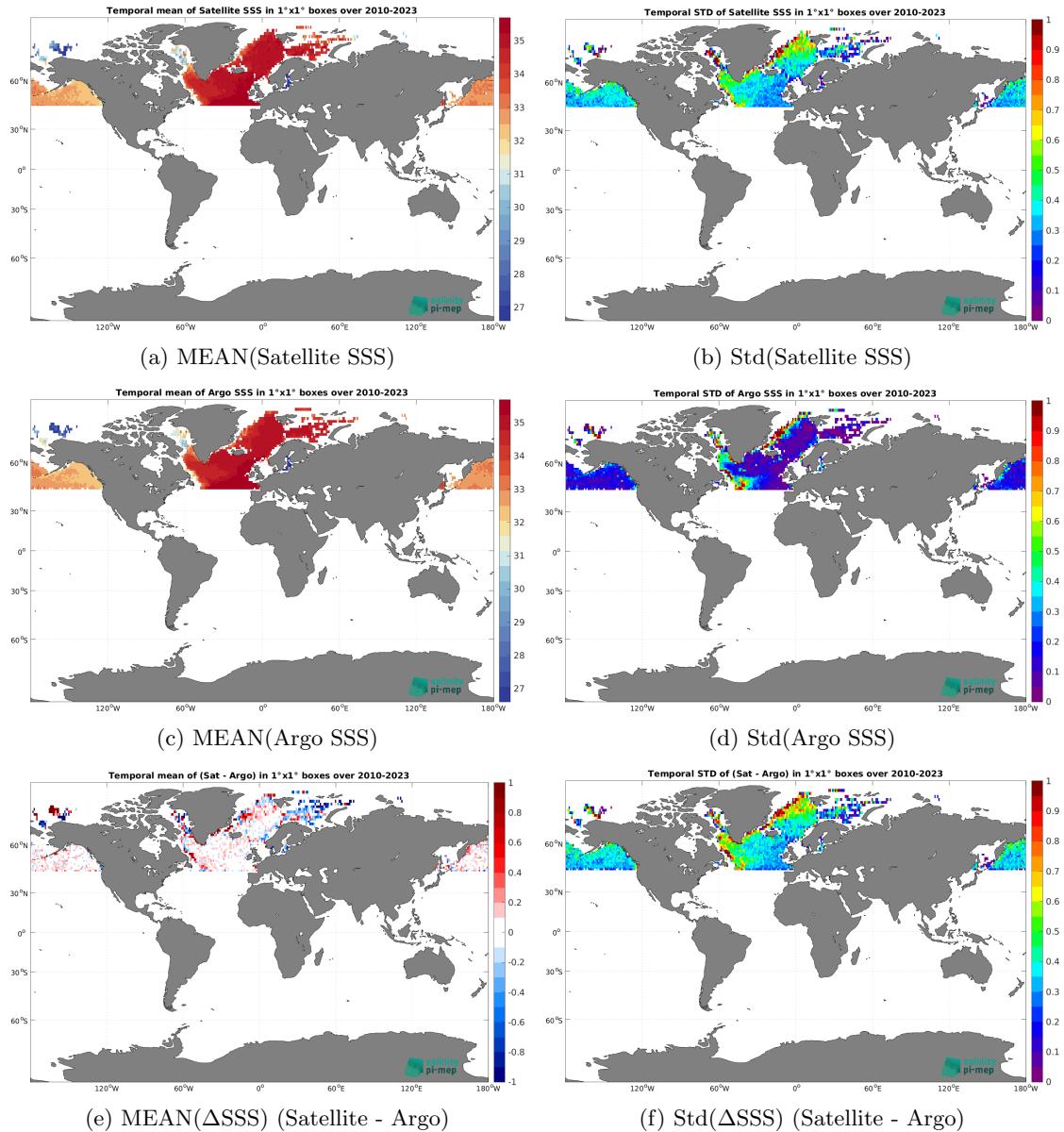
Figure 7: Temporal mean (left) and Std (right) of SSS from SMOS SSS L3 Arctic v2 - 18 Days (CATDS-CEC-LOCEAN) (top), Argo (middle), and of \Delta SSS (Satellite - Argo). Only match-up pairs are used to generate these maps.
