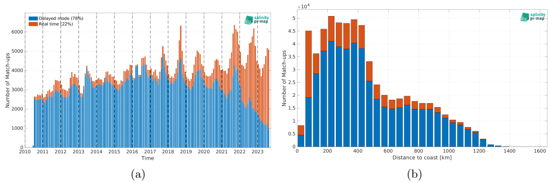
Figure 2: Number of match-ups between Argo and SMOS SSS L3 Arctic v2 - 18 Days (CATDS-CEC-LOCEAN) SSS as a function of time (a) and as function of the distance to coast (b) over the Global Ocean Pi-MEP region and for the full satellite product period.
