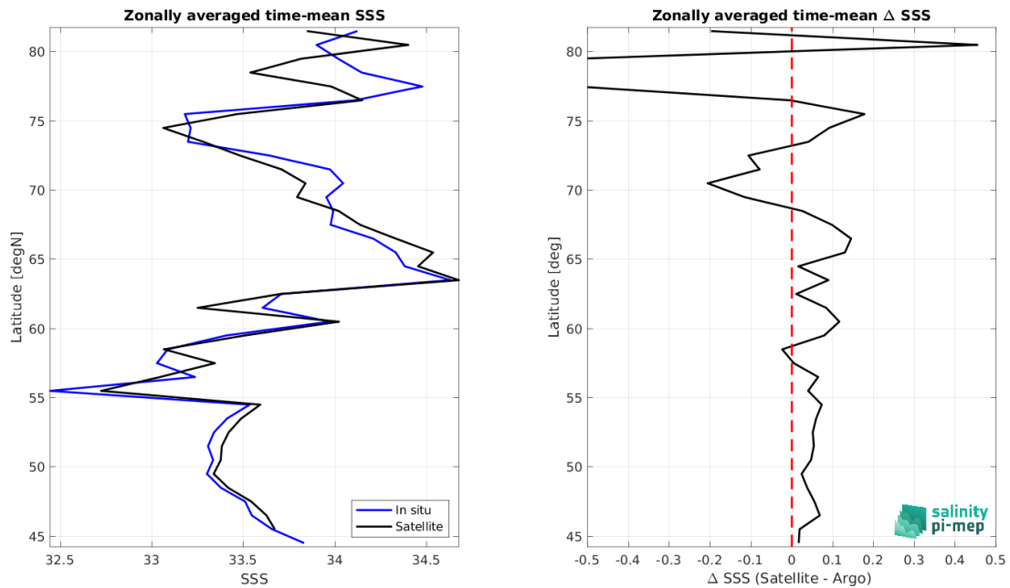
Figure 9: Left panel: Zonal mean SSS from SMOS SSS L3 Arctic v2 - 18 Days (CATDS-CEC-LOCEAN) satellite product (black) and from Argo (blue). Right panel: Zonal mean of \Delta SSS (Satellite - Argo) for all the collected Pi-MEP match-up pairs estimated over the full satellite product period.
