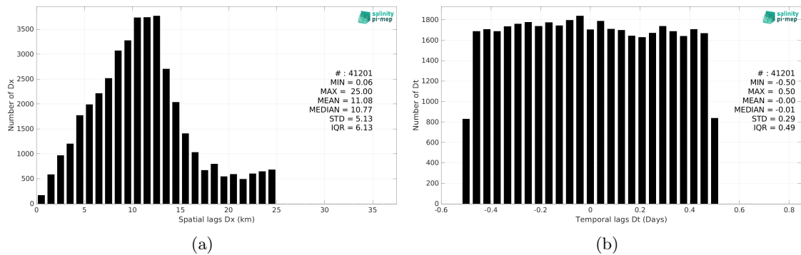
Figure 5: Histograms of the spatial (a) and temporal (b) lags between the location/time of the TSG (SAMOS) measurement and the date of the corresponding SMOS SSS L3 Arctic v1.1 - 7-Day running mean (CATDS-CEC-LOCEAN) SSS pixel.
