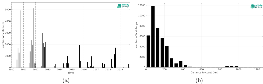
Figure 1: Number of match-ups between TSG (SAMOS) and SMOS SSS L3 Arctic v1.1 - 7-Day running mean (CATDS-CEC-LOCEAN) SSS as a function of time (a) and as function of the distance to coast (b) over the Global Ocean Pi-MEP region and for the full satellite product period.
