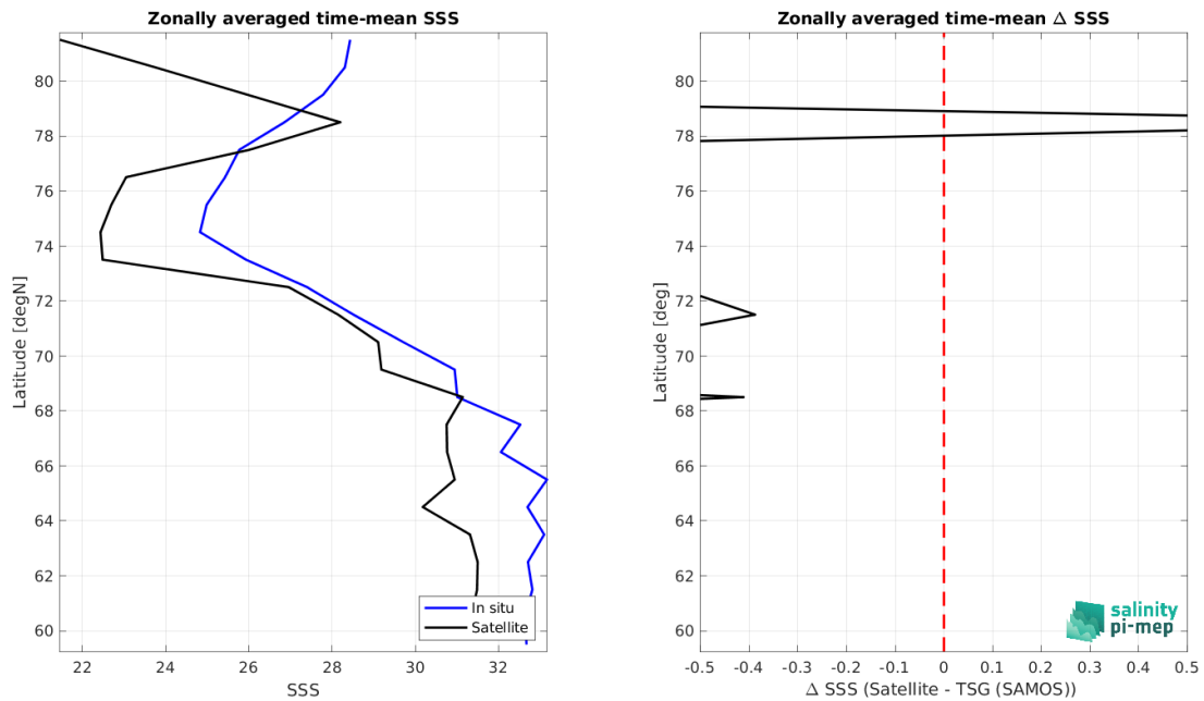
Figure 8: Left panel: Zonal mean SSS from SMOS SSS L3 Arctic v1.1 - 7-Day running mean (CATDS-CEC-LOCEAN) satellite product (black) and from TSG (SAMOS) (blue). Right panel: Zonal mean of \Delta SSS (Satellite - TSG (SAMOS)) for all the collected Pi-MEP match-up pairs estimated over the full satellite product period.
