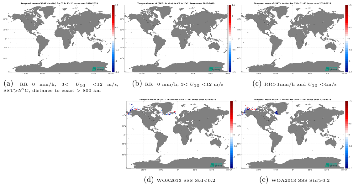
Figure 12: Temporal mean gridded over spatial boxes of size 1^{\circ}\times 1^{\circ} of \Delta\text{SSS} (SMOS SSS L3 Arctic v1.1 - 7-Day running mean (CATDS-CEC-LOCEAN) - TSG (SAMOS)) for 5 different subdatasets corresponding to:RR=0 mm/h, 3 < U_{10} < 12 m/s, SST > 5^{\circ}\text{C} , distance to coast > 800 km (a), RR=0 mm/h, 3 < U_{10} < 12 m/s (b), RR > 1 mm/h and U_{10} < 4 m/s (c), WOA2013 SSS Std < 0.2 (d), WOA2013 SSS Std > 0.2 (e).
