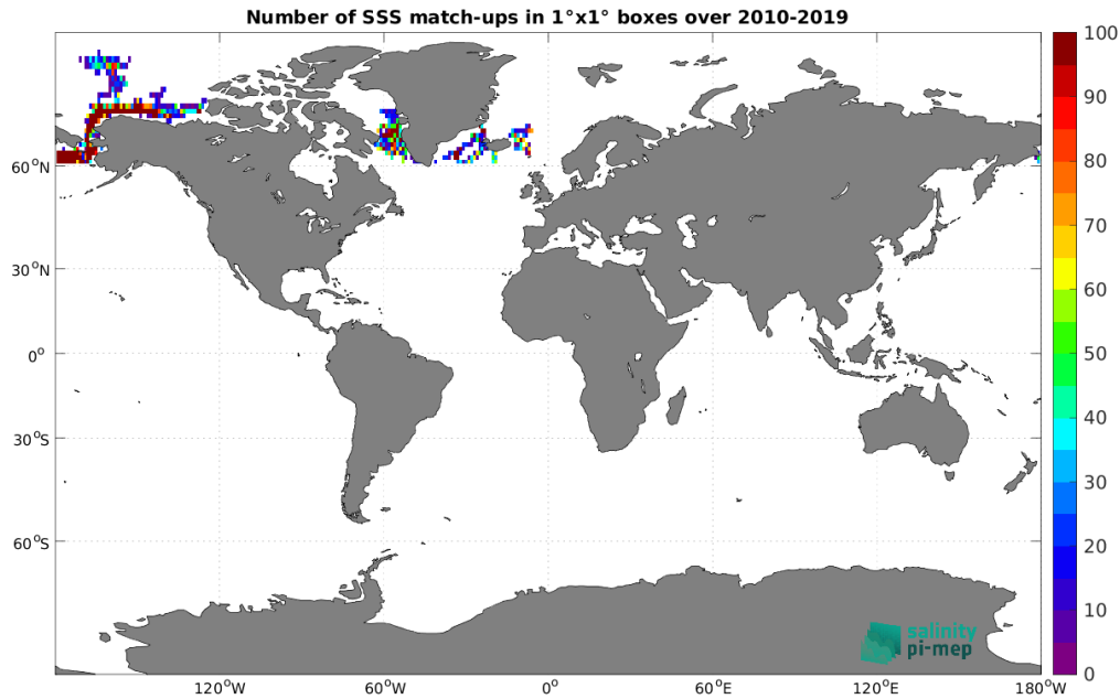
Figure 4: Number of SSS match-ups between TSG (SAMOS) SSS and the SMOS SSS L3 Arctic v1.1 - 7-Day running mean (CATDS-CEC-LOCEAN) SSS product for the Global Ocean Pi-MEP region over 1^\circ \times 1^\circ boxes and for the full satellite product period.
