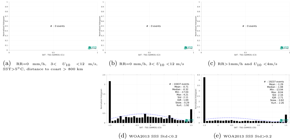
Figure 13: Normalized histogram of \Delta SSS (SMOS SSS L3 Arctic v1.1 - 7-Day runing mean (CATDS-CEC-LOCEAN) - TSG (SAMOS)) for 5 different subdatasets corresponding to: RR=0 mm/h, 3 < U_{10} < 12 m/s, SST > 5°C, distance to coast > 800 km (a), RR=0 mm/h, 3 < U_{10} < 12 m/s (b), RR > 1mm/h and U_{10} < 4 m/s (c), WOA2013 SSS Std < 0.2 (d), WOA2013 SSS Std > 0.2 (e).
