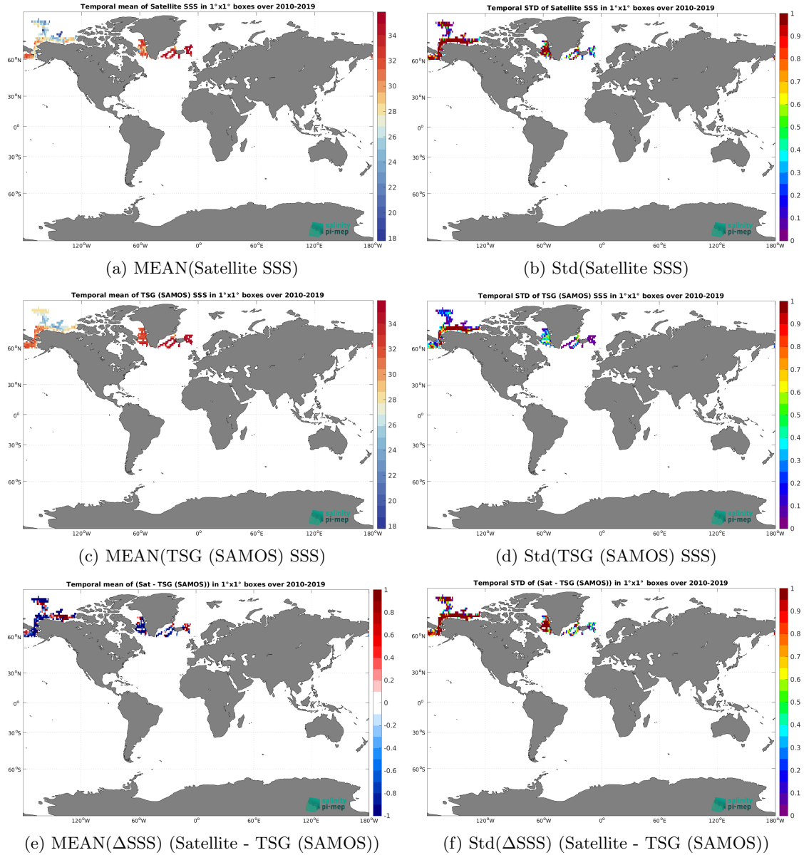
Figure 6: Temporal mean (left) and Std (right) of SSS from SMOS SSS L3 Arctic v1.1 - 7-Day running mean (CATDS-CEC-LOCEAN) (top), TSG (SAMOS) (middle), and of \Delta SSS (Satellite - TSG (SAMOS)). Only match-up pairs are used to generate these maps.
