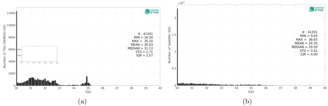
Figure 2: Histograms of SSS from TSG (SAMOS) (a) and SMOS SSS L3 Arctic v1.1 - 7-Day running mean (CATDS-CEC-LOCEAN) (b) considering all match-up pairs per bins of 0.1 over the Global Ocean Pi-MEP region and for the full satellite product period.
