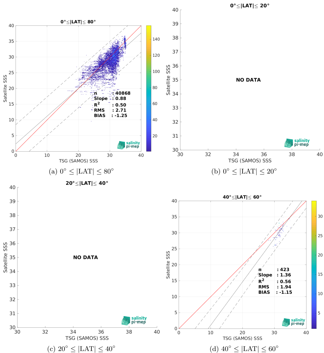
Figure 9: Contour maps of the concentration of SMOS SSS L3 Arctic v1.1 - 7-Day running mean (CATDS-CEC-LOCEAN) SSS (y-axis) versus TSG (SAMOS) SSS (x-axis) at match-up pairs for different latitude bands. For each plot, the red line shows x=y . The black thin and dashed lines indicate a linear fit through the data cloud and the \pm 95\% confidence levels, respectively. The number match-up pairs n , the slope and R^2 coefficient of the linear fit, the root mean square (RMS) and the mean bias between satellite and in situ data are indicated for each latitude band in each plots.
