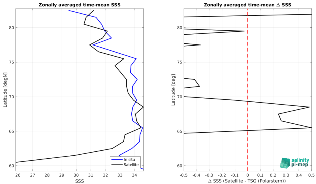
Figure 8: Left panel: Zonal mean SSS from SMOS SSS L3 Arctic v1.1 - 7-Day running mean (CATDS-CEC-LOCEAN) satellite product (black) and from TSG (Polarstern) (blue). Right panel: Zonal mean of \Delta SSS (Satellite - TSG (Polarstern)) for all the collected Pi-MEP match-up pairs estimated over the full satellite product period.
