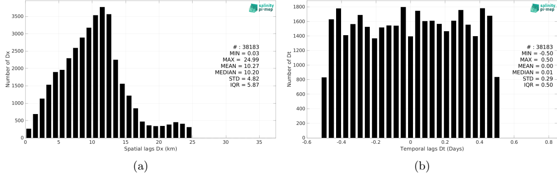
Figure 5: Histograms of the spatial (a) and temporal (b) lags between the location/time of the TSG (Polarstern) measurement and the date of the corresponding SMOS SSS L3 Arctic v1.1 - 7-Day running mean (CATDS-CEC-LOCEAN) SSS pixel.
