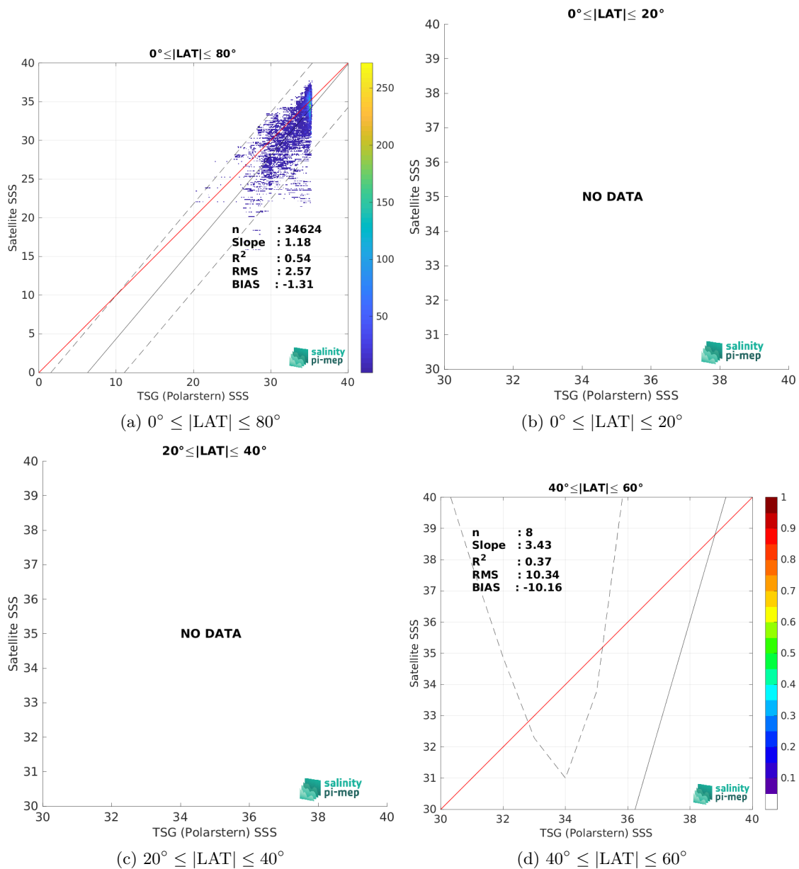
Figure 9: Contour maps of the concentration of SMOS SSS L3 Arctic v1.1 - 7-Day running mean (CATDS-CEC-LOCEAN) SSS (y-axis) versus TSG (Polarstern) SSS (x-axis) at match-up pairs for different latitude bands. For each plot, the red line shows x=y . The black thin and dashed lines indicate a linear fit through the data cloud and the \pm 95\% confidence levels, respectively. The number match-up pairs n , the slope and R^2 coefficient of the linear fit, the root mean square (RMS) and the mean bias between satellite and in situ data are indicated for each latitude band in each plots.
