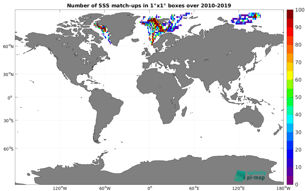
Figure 4: Number of SSS match-ups between TSG (Polarstern) SSS and the SMOS SSS L3 Arctic v1.1 - 7-Day running mean (CATDS-CEC-LOCEAN) SSS product for the Global Ocean Pi-MEP region over 1^\circ \times 1^\circ boxes and for the full satellite product period.
