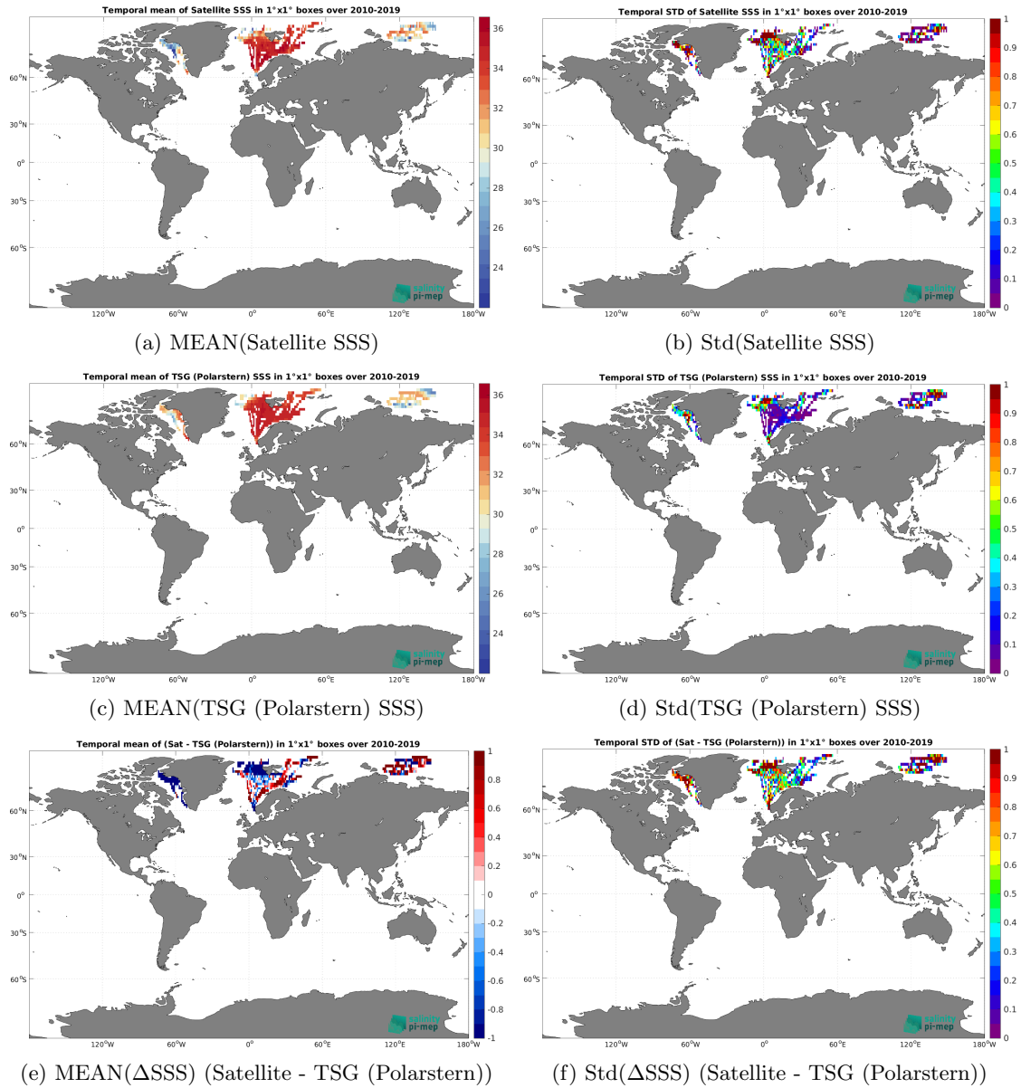
Figure 6: Temporal mean (left) and Std (right) of SSS from SMOS SSS L3 Arctic v1.1 - 7-Day running mean (CATDS-CEC-LOCEAN) (top), TSG (Polarstern) (middle), and of \Delta SSS (Satellite - TSG (Polarstern)). Only match-up pairs are used to generate these maps.
