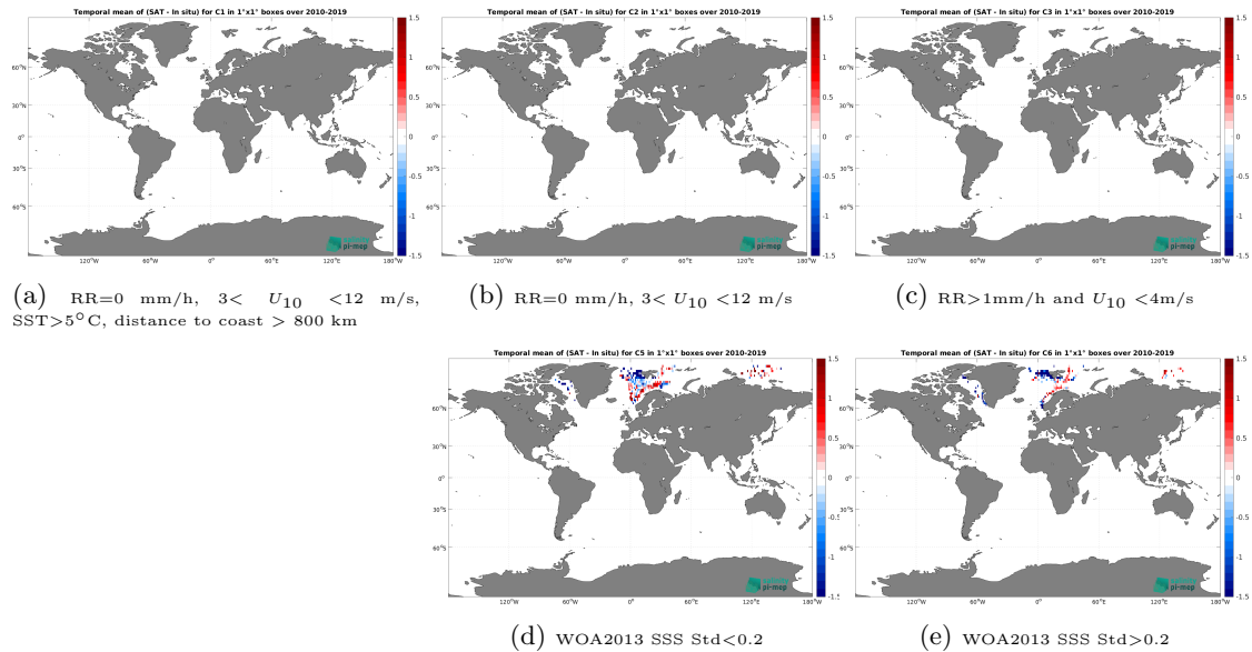
Figure 12: Temporal mean gridded over spatial boxes of size 1^{\circ}\times 1^{\circ} of \Delta\text{SSS} (SMOS SSS L3 Arctic v1.1 - 7-Day running mean (CATDS-CEC-LOCEAN) - TSG (Polarstern)) for 5 different subdatasets corresponding to:RR=0 mm/h, 3 < U_{10} < 12 m/s, SST > 5^{\circ}\text{C} , distance to coast > 800 km (a), RR=0 mm/h, 3 < U_{10} < 12 m/s (b), RR > 1 mm/h and U_{10} < 4 m/s (c), WOA2013 SSS Std < 0.2 (d), WOA2013 SSS Std > 0.2 (e).
