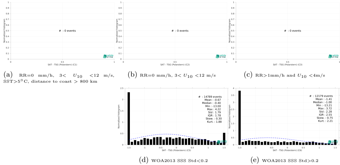
Figure 13: Normalized histogram of \Delta SSS (SMOS SSS L3 Arctic v1.1 - 7-Day runing mean (CATDS-CEC-LOCEAN) - TSG (Polarstern)) for 5 different subdatasets corresponding to: RR=0 mm/h, 3 < U_{10} < 12 m/s, SST>5°C, distance to coast > 800 km (a), RR=0 mm/h, 3 < U_{10} < 12 m/s (b), RR>1mm/h and U_{10} < 4 m/s (c), WOA2013 SSS Std<0.2 (d), WOA2013 SSS Std>0.2 (e).
