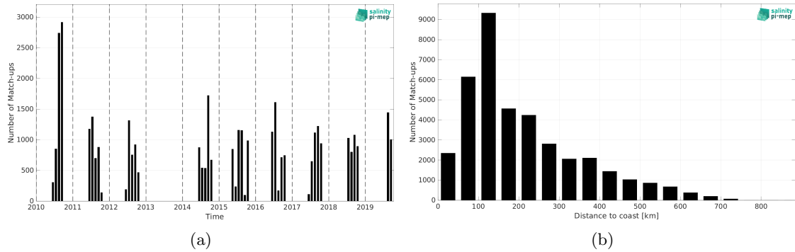
Figure 1: Number of match-ups between TSG (Polarstern) and SMOS SSS L3 Arctic v1.1 - 7-Day running mean (CATDS-CEC-LOCEAN) SSS as a function of time (a) and as function of the distance to coast (b) over the Global Ocean Pi-MEP region and for the full satellite product period.
