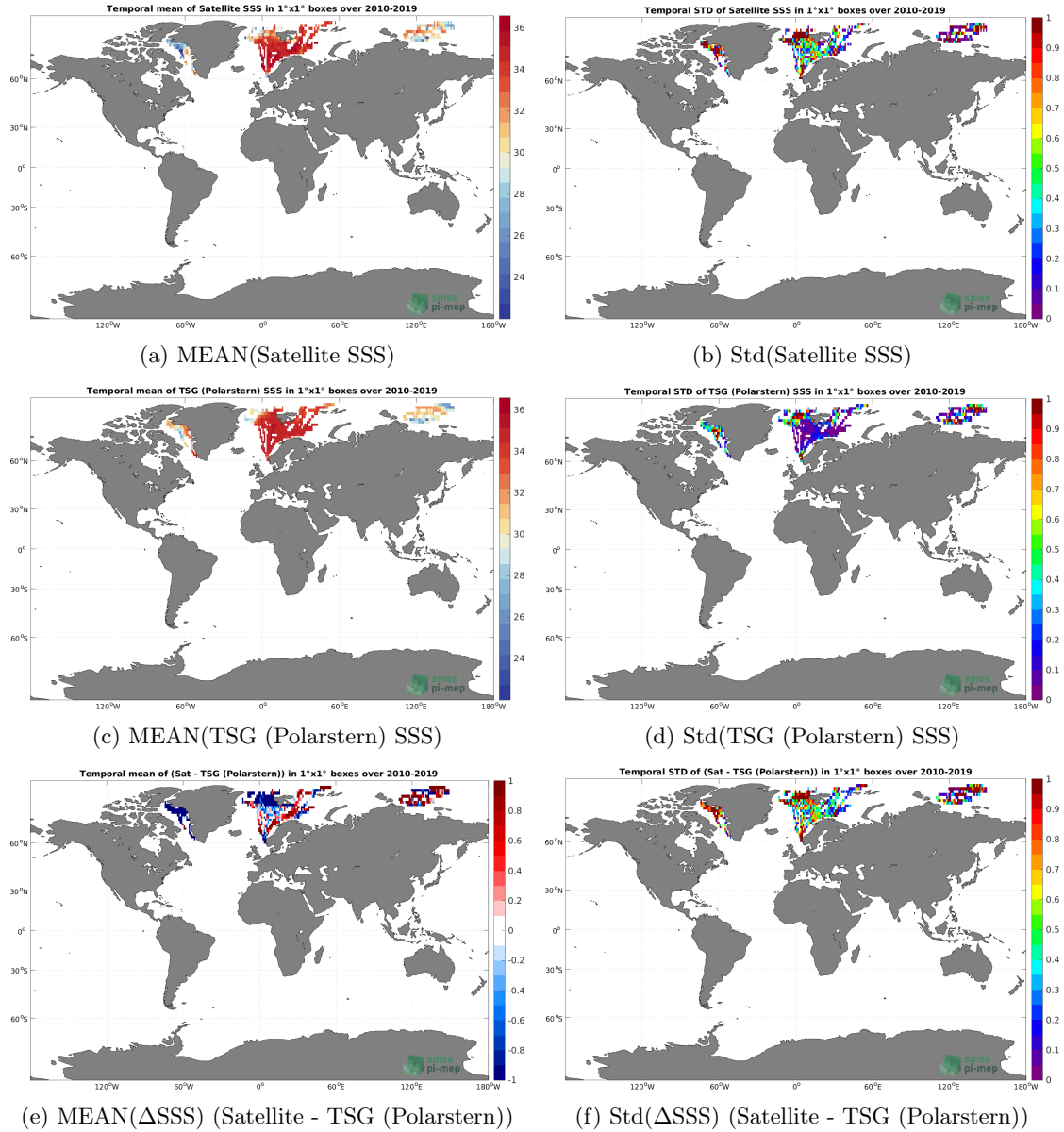
Figure 6: Temporal mean (left) and Std (right) of SSS from SMOS SSS L3 Arctic v1.1 - 7-Day running mean (CATDS-CECOS-LOCEAN) (top), TSG (Polarstern) (middle), and of \Delta SSS (Satellite - TSG (Polarstern)). Only match-up pairs are used to generate these maps.
