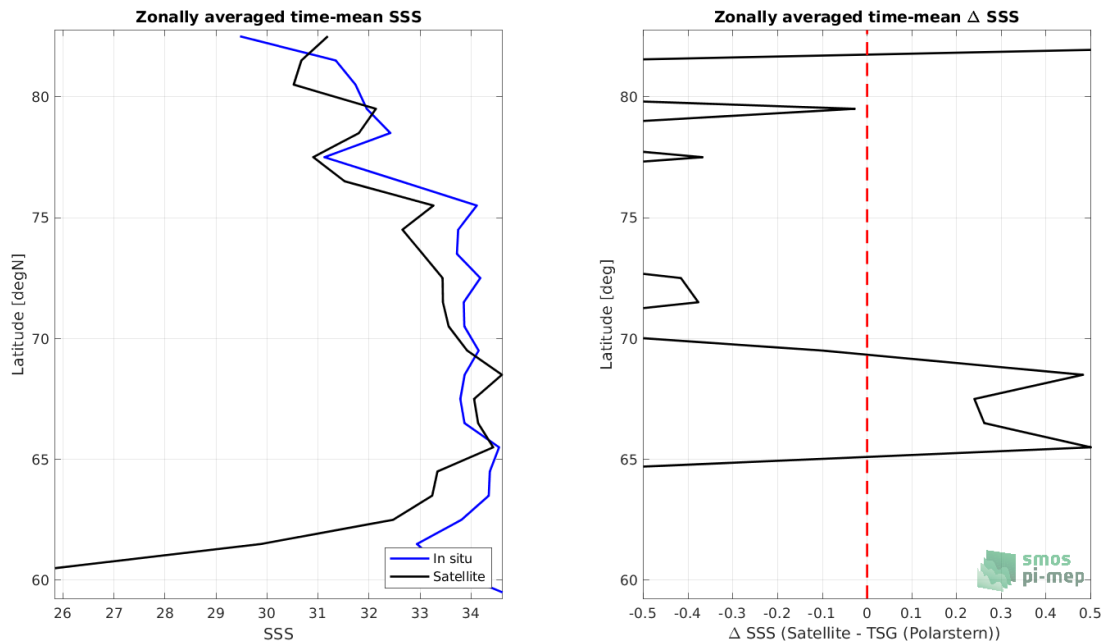
Figure 8: Left panel: Zonal mean SSS from SMOS SSS L3 Arctic v1.1 - 7-Day running mean (CATDS-CECOS-LOCEAN) satellite product (black) and from TSG (Polarstern) (blue). Right panel: Zonal mean of \Delta SSS (Satellite - TSG (Polarstern)) for all the collected Pi-MEP match-up pairs estimated over the full satellite product period.
