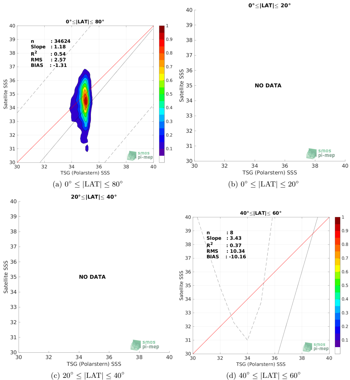
Figure 9: Contour maps of the concentration of SMOS SSS L3 Arctic v1.1 - 7-Day running mean (CATDS-CECOS-LOCEAN) SSS (y-axis) versus TSG (Polarstern) SSS (x-axis) at match-up pairs for different latitude bands. For each plot, the red line shows x=y . The black thin and dashed lines indicate a linear fit through the data cloud and the \pm 95\% confidence levels, respectively. The number match-up pairs n , the slope and R^2 coefficient of the linear fit, the root mean square (RMS) and the mean bias between satellite and in situ data are indicated for each latitude band in each plots.
