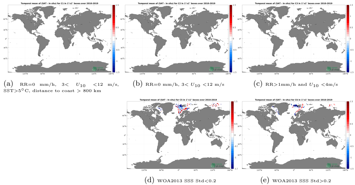
Figure 12: Temporal mean gridded over spatial boxes of size 1^{\circ}\times 1^{\circ} of \Delta\text{SSS} (SMOS SSS L3 Arctic v1.1 - 7-Day running mean (CATDS-CECOS-LOCEAN) - TSG (Polarstern)) for 5 different subdatasets corresponding to:RR=0 mm/h, 3 < U_{10} < 12 m/s, SST > 5^{\circ}\text{C} , distance to coast > 800 km (a), RR=0 mm/h, 3 < U_{10} < 12 m/s (b), RR > 1 mm/h and U_{10} < 4 m/s (c), WOA2013 SSS Std < 0.2 (d), WOA2013 SSS Std > 0.2 (e).
