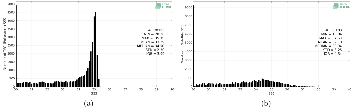
Figure 2: Histograms of SSS from TSG (Polarstern) (a) and SMOS SSS L3 Arctic v1.1 - 7-Day running mean (CATDS-CECOS-LOCEAN) (b) considering all match-up pairs per bins of 0.1 over the Global Ocean Pi-MEP region and for the full satellite product period.
