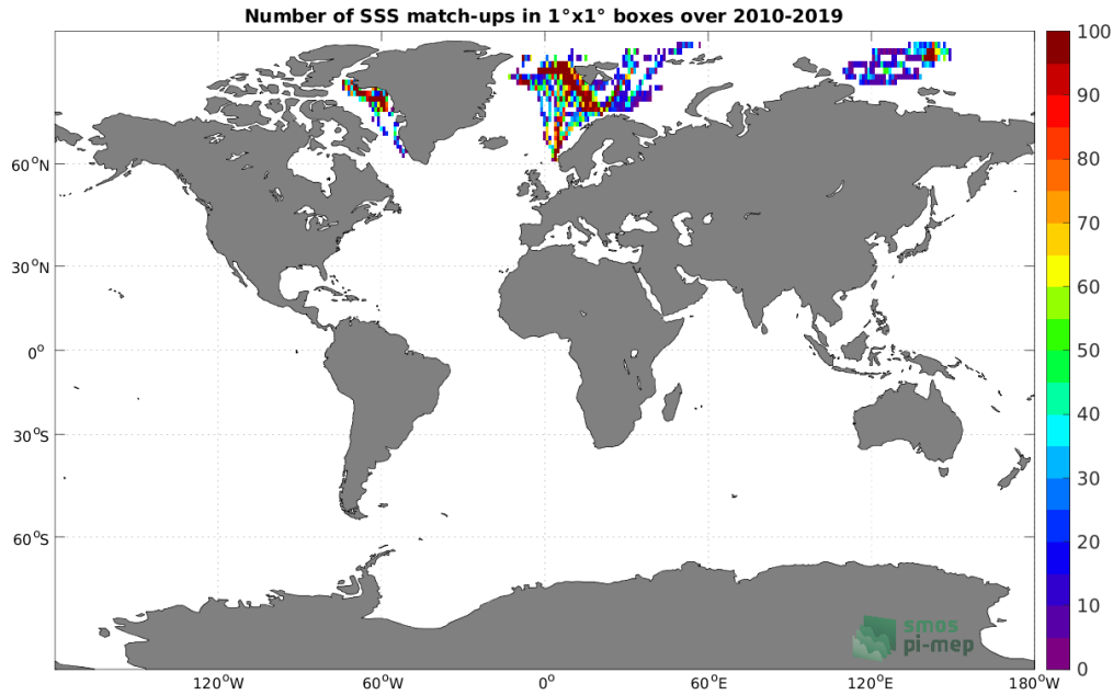
Figure 4: Number of SSS match-ups between TSG (Polarstern) SSS and the SMOS SSS L3 Arctic v1.1 - 7-Day running mean (CATDS-CECOS-LOCEAN) SSS product for the Global Ocean Pi-MEP region over 1^\circ \times 1^\circ boxes and for the full satellite product period.
