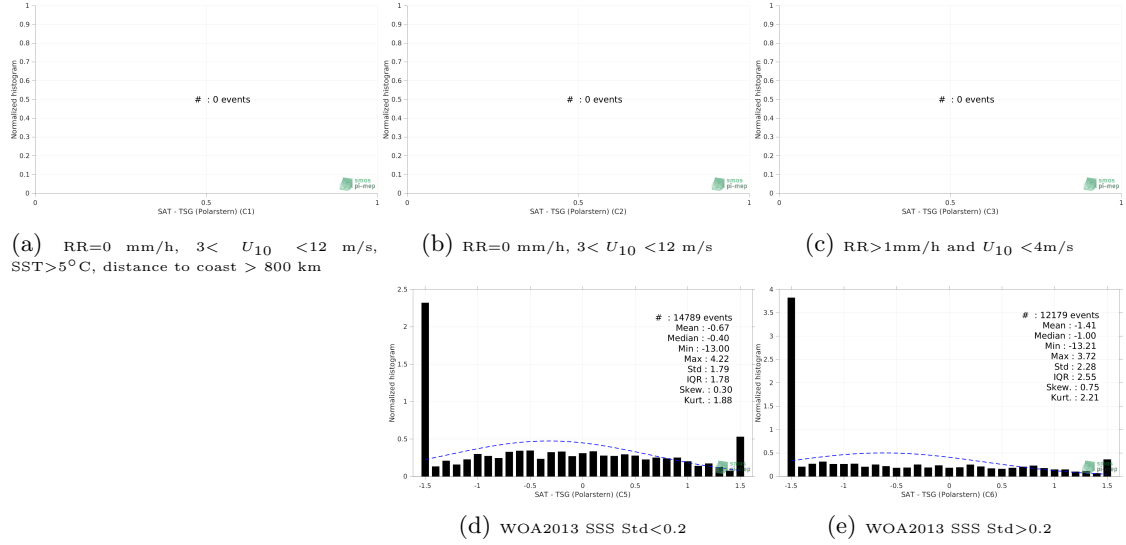
Figure 13: Normalized histogram of \Delta SSS (SMOS SSS L3 Arctic v1.1 - 7-Day running mean (CATDS-CECOS-LOCEAN) - TSG (Polarstern)) for 5 different subdatasets corresponding to: RR=0 mm/h, 3 < U_{10} < 12 m/s, SST > 5°C, distance to coast > 800 km (a), RR=0 mm/h, 3 < U_{10} < 12 m/s (b), RR > 1mm/h and U_{10} < 4 m/s (c), WOA2013 SSS Std < 0.2 (d), WOA2013 SSS Std > 0.2 (e).
