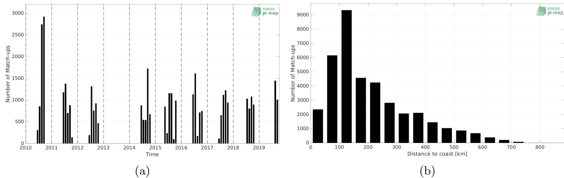
Figure 1: Number of match-ups between TSG (Polarstern) and SMOS SSS L3 Arctic v1.1 - 7-Day running mean (CATDS-CECOS-LOCEAN) SSS as a function of time (a) and as function of the distance to coast (b) over the Global Ocean Pi-MEP region and for the full satellite product period.
