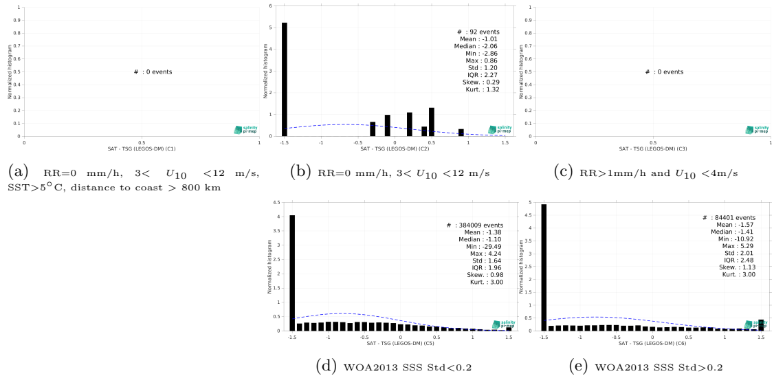
Figure 13: Normalized histogram of \Delta SSS (SMOS SSS L3 Arctic v1.1 - 7-Day runing mean (CATDS-CEC-LOCEAN) - TSG (LEGOS-DM)) for 5 different subdatasets corresponding to: RR=0 mm/h, 3 < U_{10} < 12 m/s, SST > 5°C, distance to coast > 800 km (a), RR=0 mm/h, 3 < U_{10} < 12 m/s (b), RR > 1mm/h and U_{10} < 4 m/s (c), WOA2013 SSS Std < 0.2 (d), WOA2013 SSS Std > 0.2 (e).
