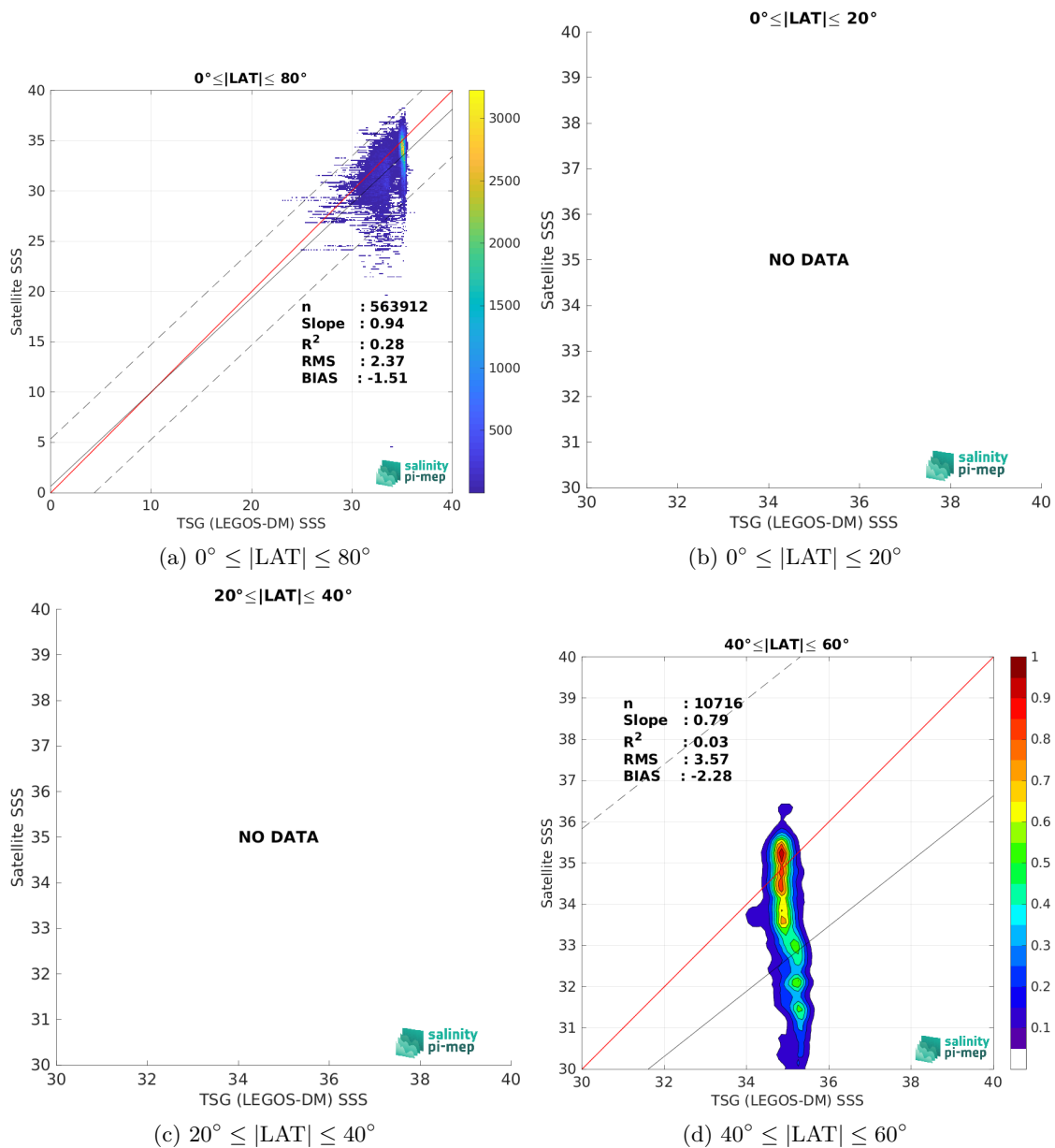
Figure 9: Contour maps of the concentration of SMOS SSS L3 Arctic v1.1 - 7-Day running mean (CATDS-CEC-LOCEAN) SSS (y-axis) versus TSG (LEGOS-DM) SSS (x-axis) at match-up pairs for different latitude bands. For each plot, the red line shows x=y . The black thin and dashed lines indicate a linear fit through the data cloud and the \pm 95\% confidence levels, respectively. The number match-up pairs n , the slope and R^2 coefficient of the linear fit, the root mean square (RMS) and the mean bias between satellite and in situ data are indicated for each latitude band in each plots.
