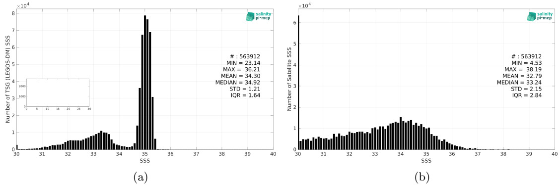
Figure 2: Histograms of SSS from TSG (LEGOS-DM) (a) and SMOS SSS L3 Arctic v1.1 - 7-Day running mean (CATDS-CEC-LOCEAN) (b) considering all match-up pairs per bins of 0.1 over the Global Ocean Pi-MEP region and for the full satellite product period.
