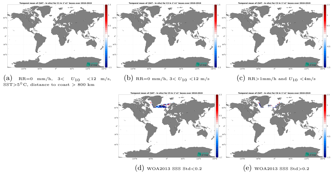
Figure 12: Temporal mean gridded over spatial boxes of size 1^{\circ}\times 1^{\circ} of \Delta\text{SSS} (SMOS SSS L3 Arctic v1.1 - 7-Day running mean (CATDS-CEC-LOCEAN) - TSG (LEGOS-DM)) for 5 different subdatasets corresponding to:RR=0 mm/h, 3 < U_{10} < 12 m/s, SST > 5^{\circ}\text{C} , distance to coast > 800 km (a), RR=0 mm/h, 3 < U_{10} < 12 m/s (b), RR > 1 mm/h and U_{10} < 4 m/s (c), WOA2013 SSS Std < 0.2 (d), WOA2013 SSS Std > 0.2 (e).
