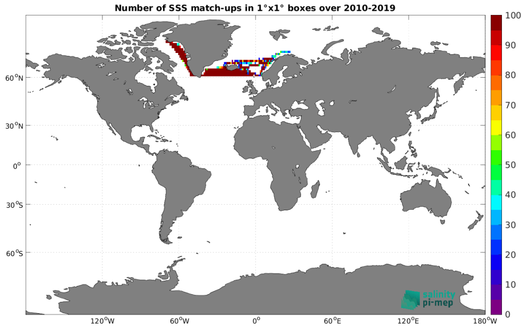
Figure 4: Number of SSS match-ups between TSG (LEGOS-DM) SSS and the SMOS SSS L3 Arctic v1.1 - 7-Day running mean (CATDS-CEC-LOCEAN) SSS product for the Global Ocean Pi-MEP region over 1^\circ \times 1^\circ boxes and for the full satellite product period.
