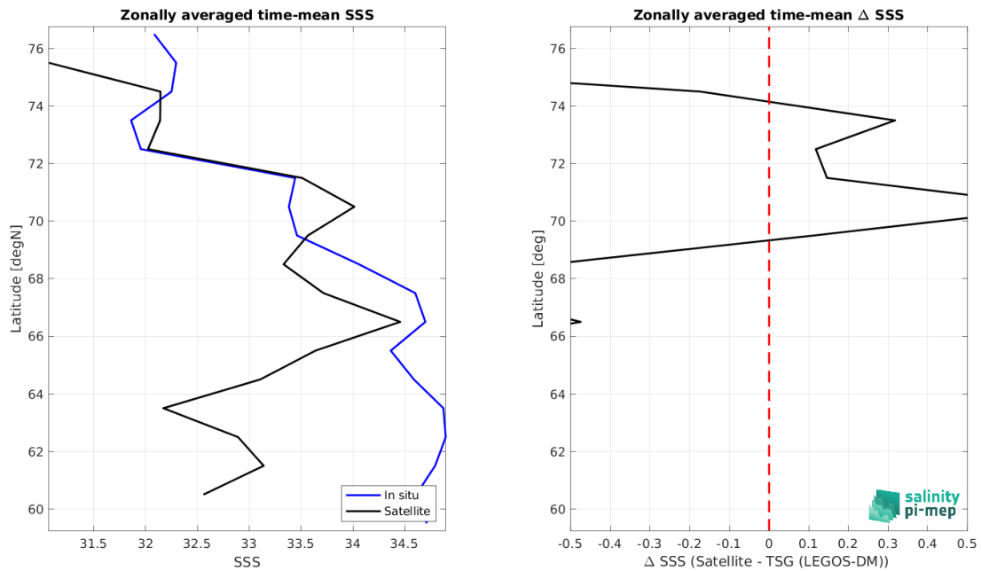
Figure 8: Left panel: Zonal mean SSS from SMOS SSS L3 Arctic v1.1 - 7-Day running mean (CATDS-CEC-LOCEAN) satellite product (black) and from TSG (LEGOS-DM) (blue). Right panel: Zonal mean of \Delta SSS (Satellite - TSG (LEGOS-DM)) for all the collected Pi-MEP match-up pairs estimated over the full satellite product period.
