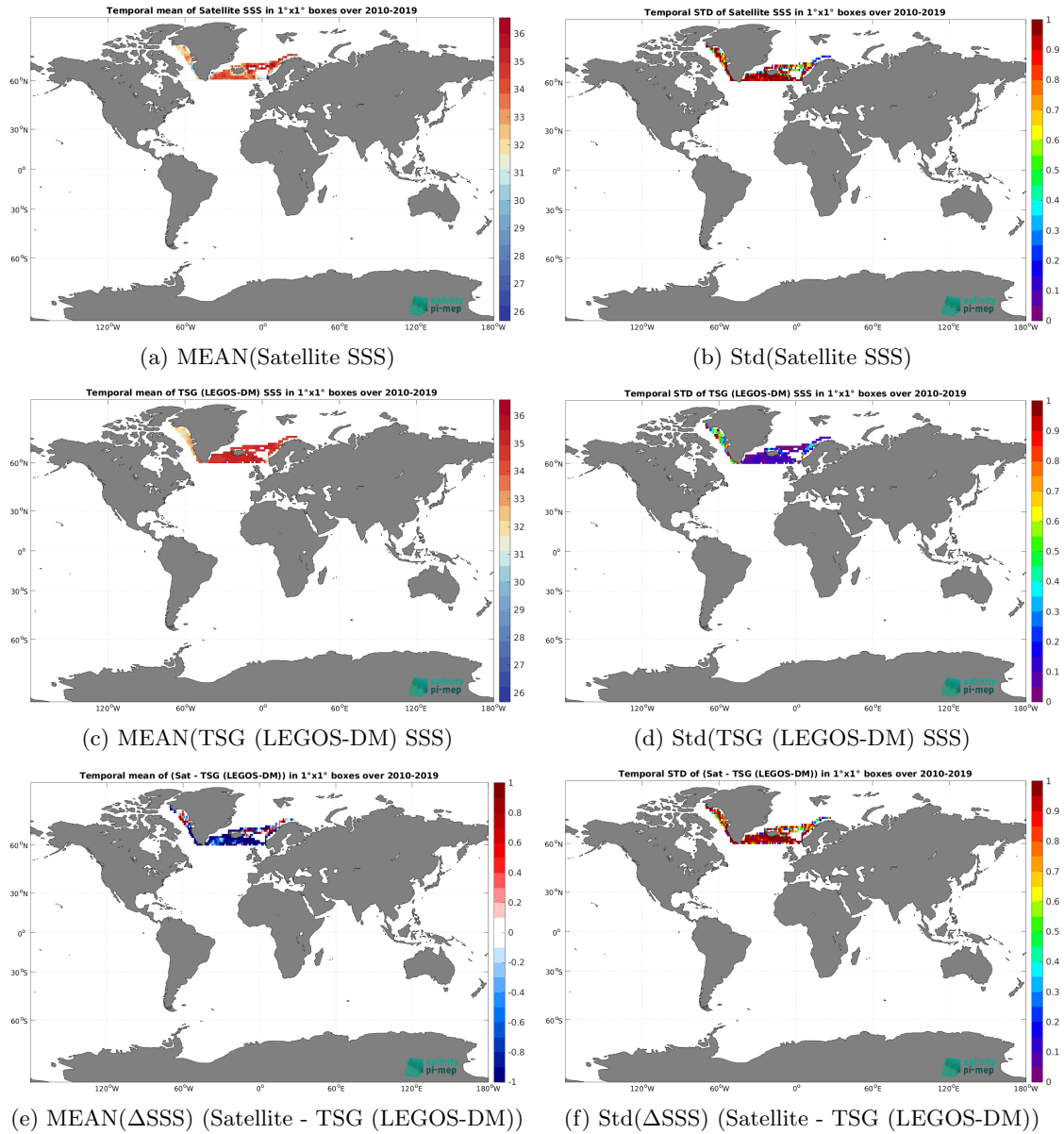
Figure 6: Temporal mean (left) and Std (right) of SSS from SMOS SSS L3 Arctic v1.1 - 7-Day running mean (CATDS-CEC-LOCEAN) (top), TSG (LEGOS-DM) (middle), and of \Delta SSS (Satellite - TSG (LEGOS-DM)). Only match-up pairs are used to generate these maps.
