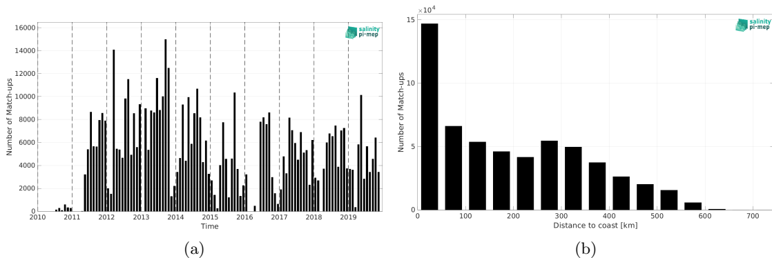
Figure 1: Number of match-ups between TSG (LEGOS-DM) and SMOS SSS L3 Arctic v1.1 - 7-Day running mean (CATDS-CEC-LOCEAN) SSS as a function of time (a) and as function of the distance to coast (b) over the Global Ocean Pi-MEP region and for the full satellite product period.
