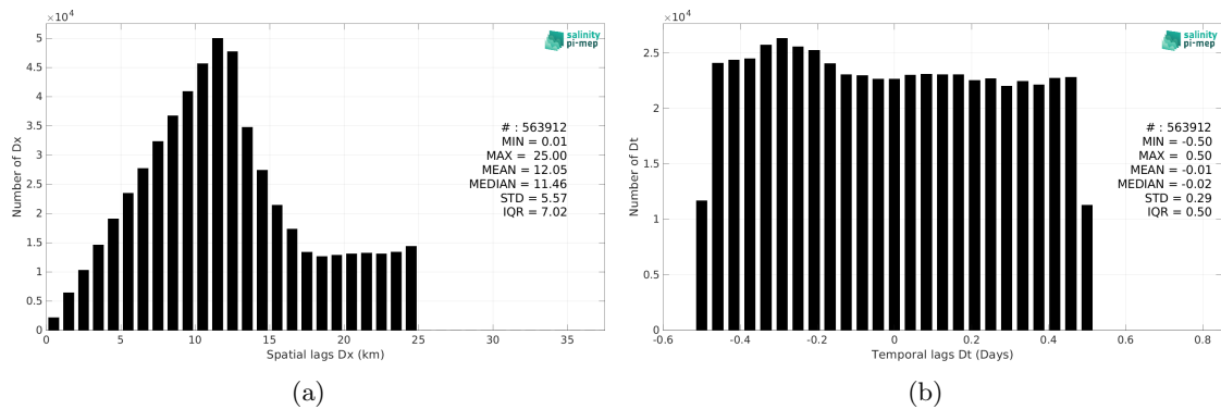
Figure 5: Histograms of the spatial (a) and temporal (b) lags between the location/time of the TSG (LEGOS-DM) measurement and the date of the corresponding SMOS SSS L3 Arctic v1.1 - 7-Day running mean (CATDS-CEC-LOCEAN) SSS pixel.
