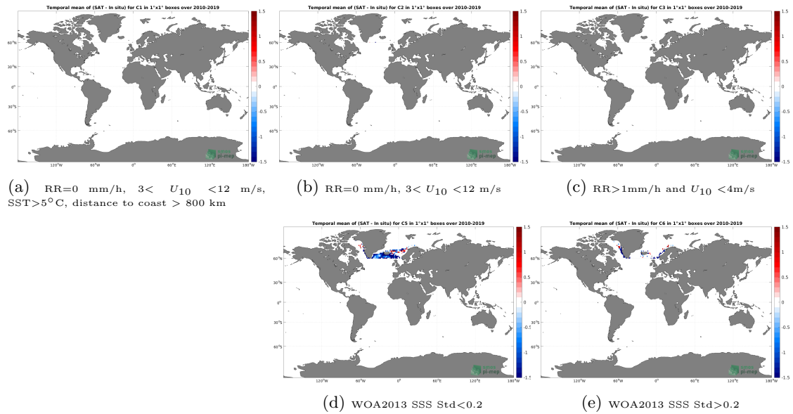
Figure 12: Temporal mean gridded over spatial boxes of size 1^{\circ}\times 1^{\circ} of \Delta\text{SSS} (SMOS SSS L3 Arctic v1.1 - 7-Day running mean (CATDS-CECOS-LOCEAN) - TSG (LEGOS-DM)) for 5 different subdatasets corresponding to:RR=0 mm/h, 3 < U_{10} < 12 m/s, SST >5^{\circ}\text{C} , distance to coast > 800 km (a), RR=0 mm/h, 3 < U_{10} < 12 m/s (b), RR >1 mm/h and U_{10} < 4 m/s (c), WOA2013 SSS Std <0.2 (d), WOA2013 SSS Std >0.2 (e).
