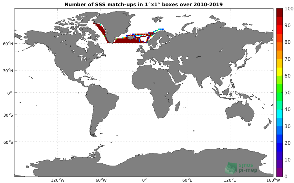
Figure 4: Number of SSS match-ups between TSG (LEGOS-DM) SSS and the SMOS SSS L3 Arctic v1.1 - 7-Day running mean (CATDS-CECOS-LOCEAN) SSS product for the Global Ocean Pi-MEP region over 1^\circ \times 1^\circ boxes and for the full satellite product period.
