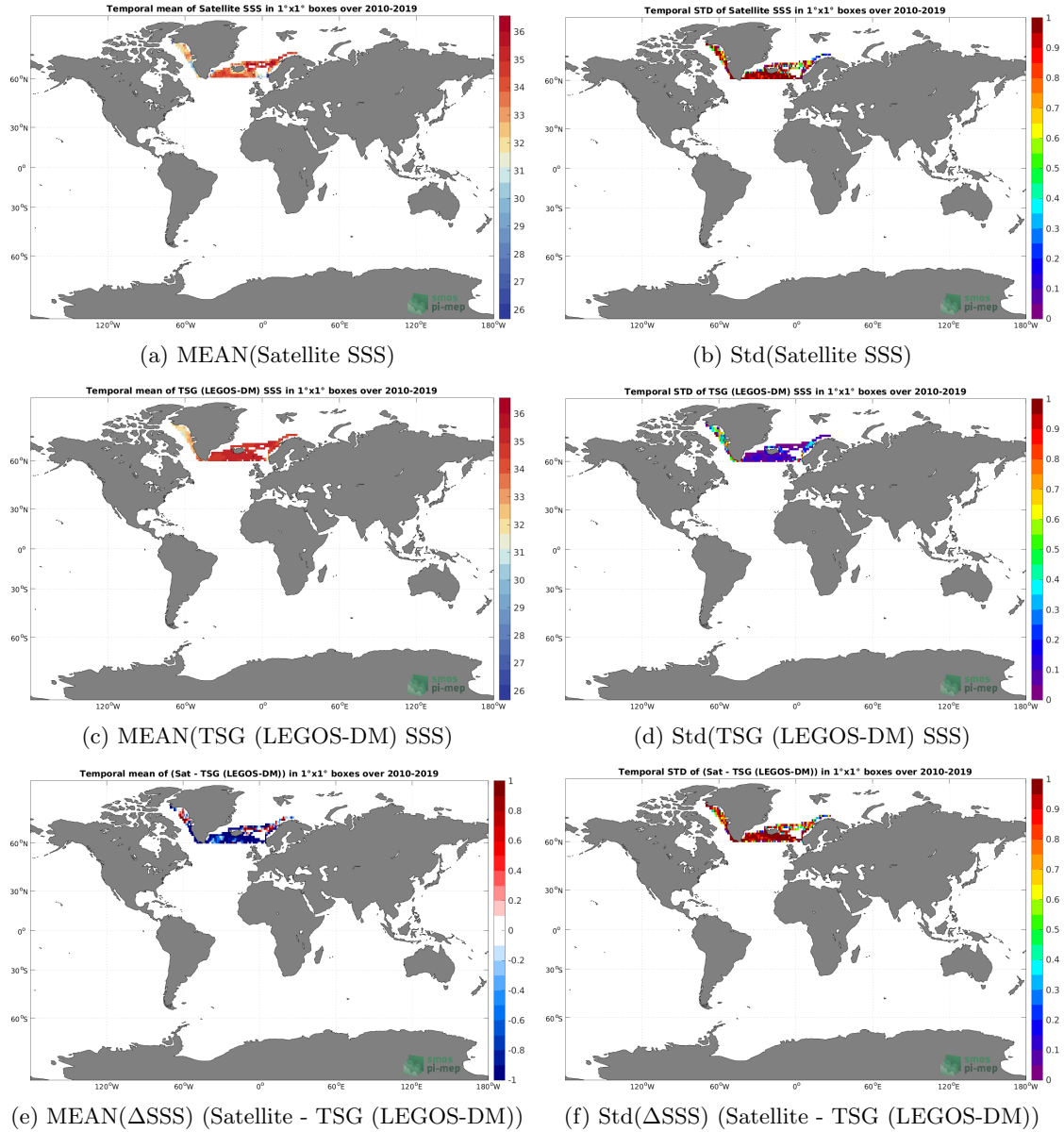
Figure 6: Temporal mean (left) and Std (right) of SSS from SMOS SSS L3 Arctic v1.1 - 7-Day running mean (CATDS-CECOS-LOCEAN) (top), TSG (LEGOS-DM) (middle), and of \Delta SSS (Satellite - TSG (LEGOS-DM)). Only match-up pairs are used to generate these maps.
