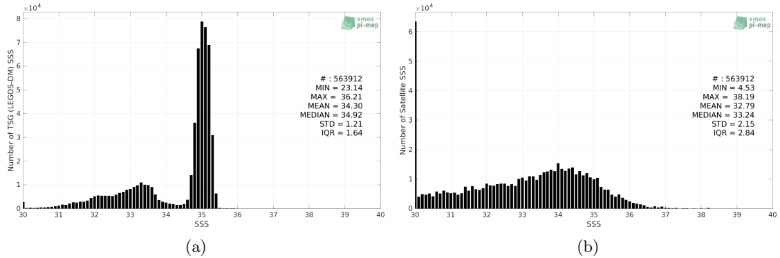
Figure 2: Histograms of SSS from TSG (LEGOS-DM) (a) and SMOS SSS L3 Arctic v1.1 - 7-Day running mean (CATDS-CECOS-LOCEAN) (b) considering all match-up pairs per bins of 0.1 over the Global Ocean Pi-MEP region and for the full satellite product period.
