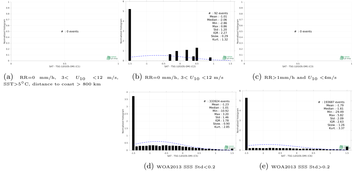
Figure 13: Normalized histogram of \Delta SSS (SMOS SSS L3 Arctic v1.1 - 7-Day running mean (CATDS-CECOS-LOCEAN) - TSG (LEGOS-DM)) for 5 different subdatasets corresponding to: RR=0 mm/h, 3 < U_{10} < 12 m/s, SST > 5°C, distance to coast > 800 km (a), RR=0 mm/h, 3 < U_{10} < 12 m/s (b), RR > 1mm/h and U_{10} < 4 m/s (c), WOA2013 SSS Std < 0.2 (d), WOA2013 SSS Std > 0.2 (e).
