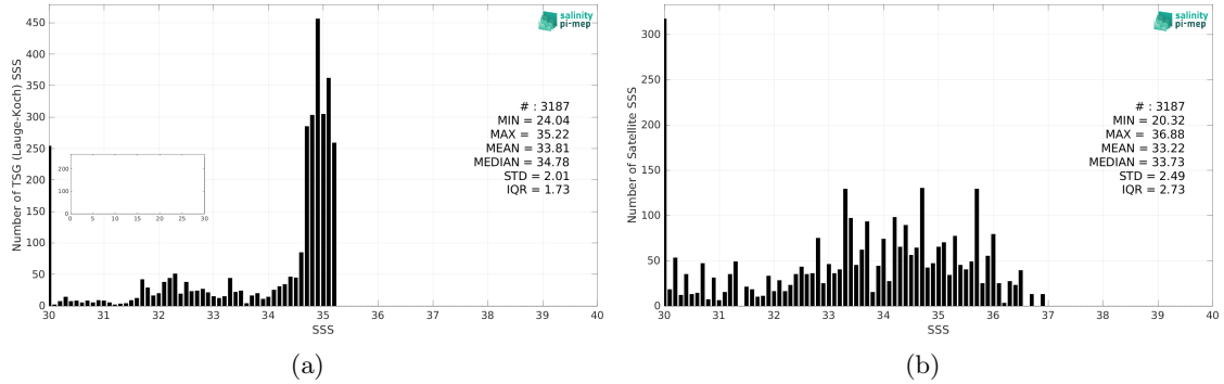
Figure 2: Histograms of SSS from TSG (Lauge-Koch) (a) and SMOS SSS L3 Arctic v1.1 - 7-Day running mean (CATDS-CEC-LOCEAN) (b) considering all match-up pairs per bins of 0.1 over the Global Ocean Pi-MEP region and for the full satellite product period.
