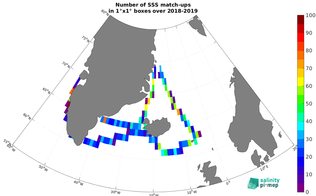
Figure 4: Number of SSS match-ups between TSG (Lauge-Koch) SSS and the SMOS SSS L3 Arctic v1.1 - 7-Day running mean (CATDS-CEC-LOCEAN) SSS product for the Global Ocean Pi-MEP region over 1^\circ \times 1^\circ boxes and for the full satellite product period.
