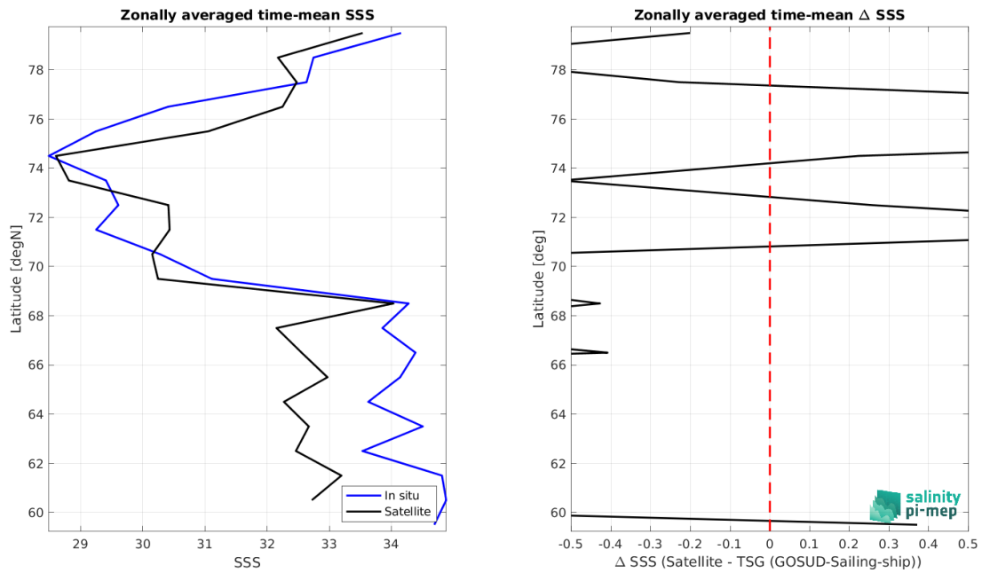
Figure 8: Left panel: Zonal mean SSS from SMOS SSS L3 Arctic v1.1 - 7-Day running mean (CATDS-CEC-LOCEAN) satellite product (black) and from TSG (GOSUD-Sailing-ship) (blue). Right panel: Zonal mean of \Delta SSS (Satellite - TSG (GOSUD-Sailing-ship)) for all the collected Pi-MEP match-up pairs estimated over the full satellite product period.
