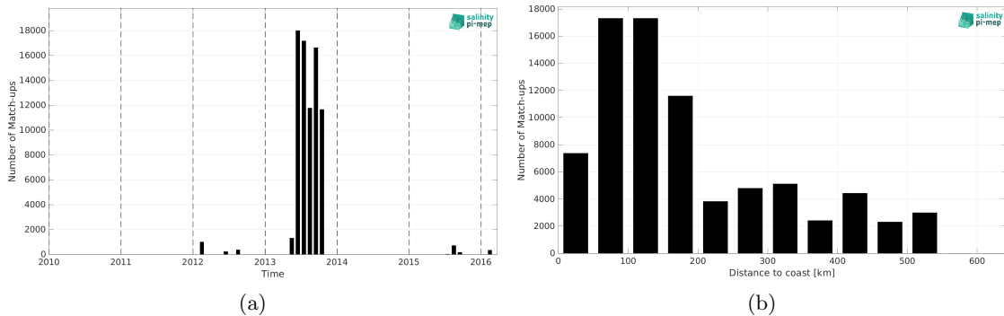
Figure 1: Number of match-ups between TSG (GOSUD-Sailing-ship) and SMOS SSS L3 Arctic v1.1 - 7-Day running mean (CATDS-CEC-LOCEAN) SSS as a function of time (a) and as function of the distance to coast (b) over the Global Ocean Pi-MEP region and for the full satellite product period.
