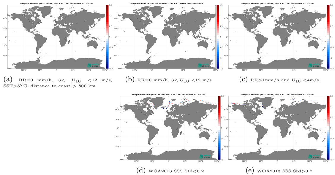
Figure 12: Temporal mean gridded over spatial boxes of size 1^{\circ}\times 1^{\circ} of \Delta SSS (SMOS SSS L3 Arctic v1.1 - 7-Day running mean (CATDS-CEC-LOCEAN) - TSG (GOSUD-Sailing-ship)) for 5 different subdatasets corresponding to:RR=0 mm/h, 3 < U_{10} < 12 m/s, SST >5^{\circ}\text{C} , distance to coast > 800 km (a), RR=0 mm/h, 3 < U_{10} < 12 m/s (b), RR >1 mm/h and U_{10} < 4 m/s (c), WOA2013 SSS Std <0.2 (d), WOA2013 SSS Std >0.2 (e).
