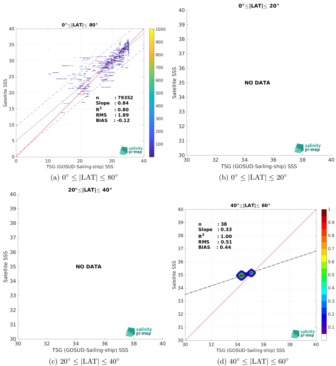
Figure 9: Contour maps of the concentration of SMOS SSS L3 Arctic v1.1 - 7-Day running mean (CATDS-CEC-LOCEAN) SSS (y-axis) versus TSG (GOSUD-Sailing-ship) SSS (x-axis) at match-up pairs for different latitude bands. For each plot, the red line shows x=y . The black thin and dashed lines indicate a linear fit through the data cloud and the \pm 95\% confidence levels, respectively. The number match-up pairs n , the slope and R^2 coefficient of the linear fit, the root mean square (RMS) and the mean bias between satellite and in situ data are indicated for each latitude band in each plots.
