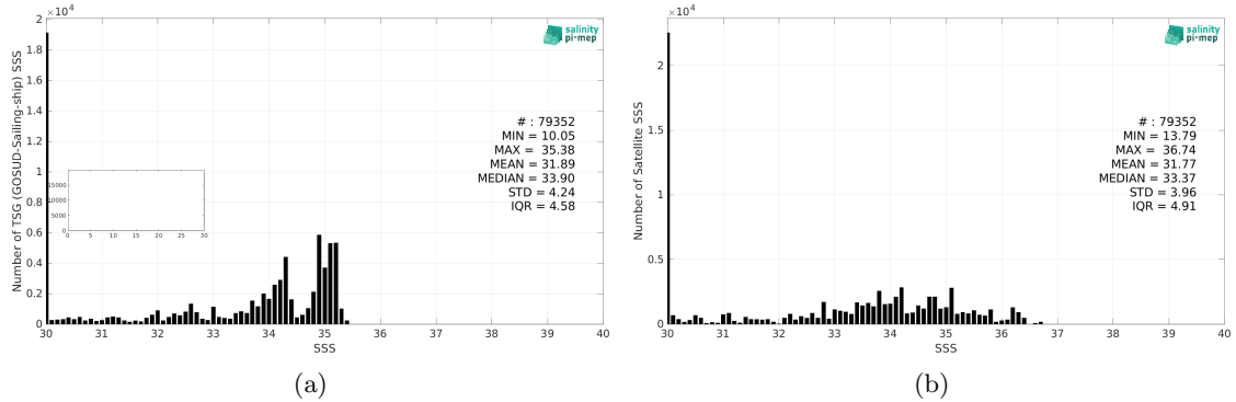
Figure 2: Histograms of SSS from TSG (GOSUD-Sailing-ship) (a) and SMOS SSS L3 Arctic v1.1 - 7-Day running mean (CATDS-CEC-LOCEAN) (b) considering all match-up pairs per bins of 0.1 over the Global Ocean Pi-MEP region and for the full satellite product period.
