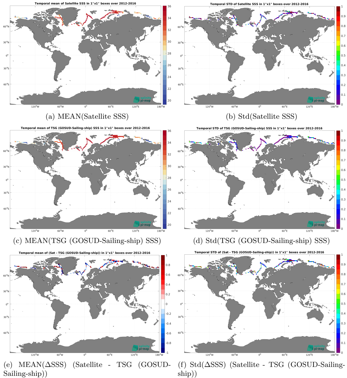
Figure 6: Temporal mean (left) and Std (right) of SSS from SMOS SSS L3 Arctic v1.1 - 7-Day running mean (CATDS-CEC-LOCEAN) (top), TSG (GOSUD-Sailing-ship) (middle), and of \Delta SSS (Satellite - TSG (GOSUD-Sailing-ship)). Only match-up pairs are used to generate these maps.
