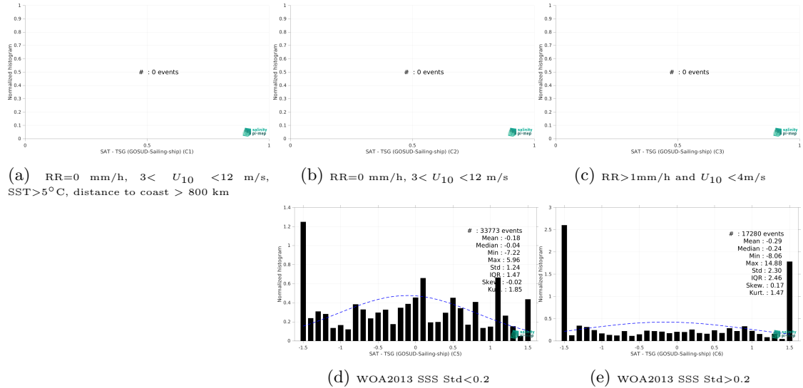
Figure 13: Normalized histogram of \Delta SSS (SMOS SSS L3 Arctic v1.1 - 7-Day runing mean (CATDS-CEC-LOCEAN) - TSG (GOSUD-Sailing-ship)) for 5 different subdatasets corresponding to: RR=0 mm/h, 3 < U_{10} < 12 m/s, SST>5°C, distance to coast > 800 km (a), RR=0 mm/h, 3 < U_{10} < 12 m/s (b), RR>1mm/h and U_{10} < 4 m/s (c), WOA2013 SSS Std<0.2 (d), WOA2013 SSS Std>0.2 (e).
