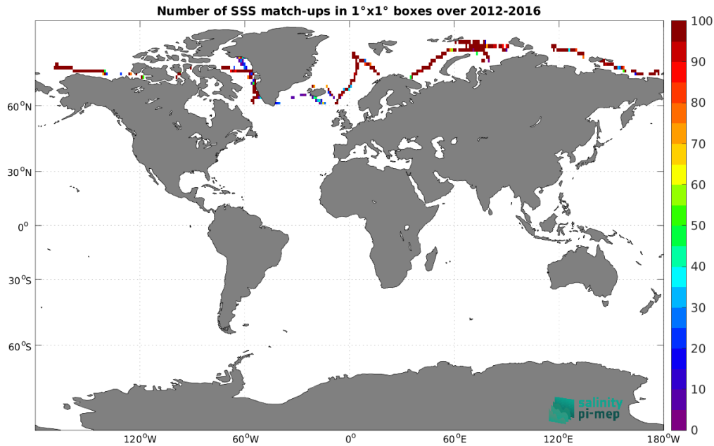
Figure 4: Number of SSS match-ups between TSG (GOSUD-Sailing-ship) SSS and the SMOS SSS L3 Arctic v1.1 - 7-Day running mean (CATDS-CEC-LOCEAN) SSS product for the Global Ocean Pi-MEP region over 1^\circ \times 1^\circ boxes and for the full satellite product period.
