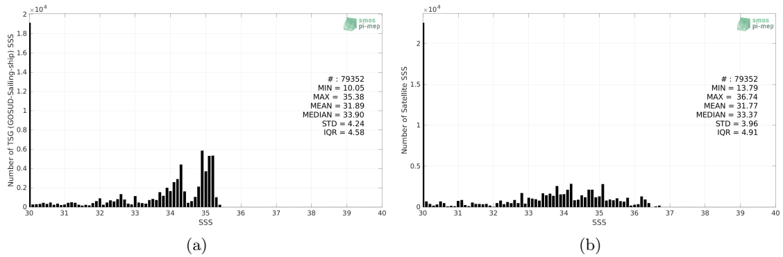
Figure 2: Histograms of SSS from TSG (GOSUD-Sailing-ship) (a) and SMOS SSS L3 Arctic v1.1 - 7-Day running mean (CATDS-CECOS-LOCEAN) (b) considering all match-up pairs per bins of 0.1 over the Global Ocean Pi-MEP region and for the full satellite product period.
