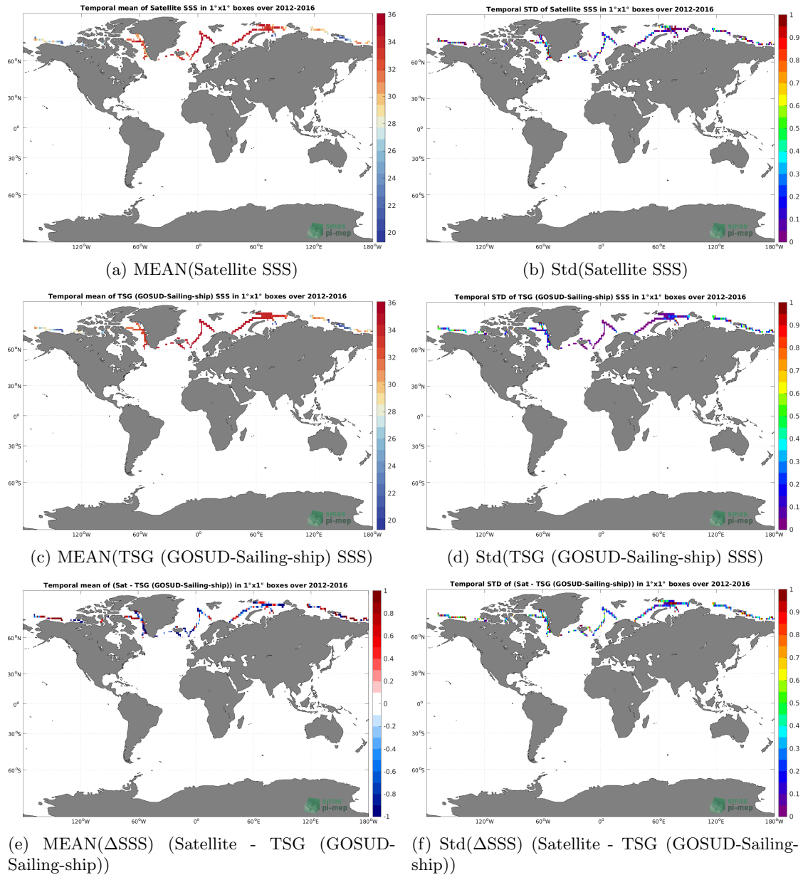
Figure 6: Temporal mean (left) and Std (right) of SSS from SMOS SSS L3 Arctic v1.1 - 7-Day running mean (CATDS-CECOS-LOCEAN) (top), TSG (GOSUD-Sailing-ship) (middle), and of \Delta SSS (Satellite - TSG (GOSUD-Sailing-ship)). Only match-up pairs are used to generate these maps.
