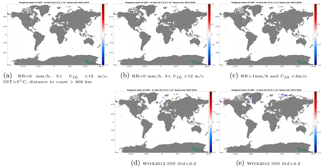
Figure 12: Temporal mean gridded over spatial boxes of size 1^{\circ}\times 1^{\circ} of \Delta SSS (SMOS SSS L3 Arctic v1.1 - 7-Day running mean (CATDS-CECOS-LOCEAN) - TSG (GOSUD-Sailing-ship)) for 5 different subdatasets corresponding to:RR=0 mm/h, 3 < U_{10} < 12 m/s, SST >5^{\circ}\text{C} , distance to coast > 800 km (a), RR=0 mm/h, 3 < U_{10} < 12 m/s (b), RR >1 mm/h and U_{10} < 4 m/s (c), WOA2013 SSS Std <0.2 (d), WOA2013 SSS Std >0.2 (e).
