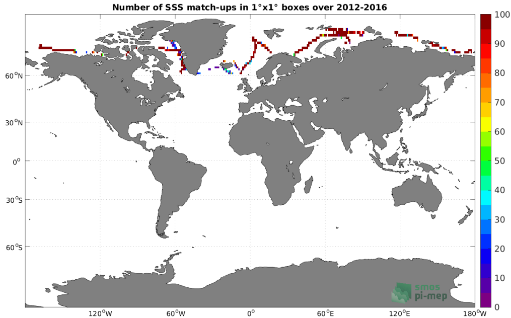
Figure 4: Number of SSS match-ups between TSG (GOSUD-Sailing-ship) SSS and the SMOS SSS L3 Arctic v1.1 - 7-Day running mean (CATDS-CECOS-LOCEAN) SSS product for the Global Ocean Pi-MEP region over 1^\circ \times 1^\circ boxes and for the full satellite product period.
