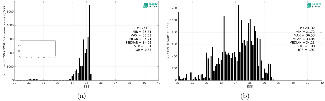
Figure 2: Histograms of SSS from TSG (GOSUD-Research-vessel) (a) and SMOS SSS L3 Arctic v1.1 - 7-Day running mean (CATDS-CEC-LOCEAN) (b) considering all match-up pairs per bins of 0.1 over the Global Ocean Pi-MEP region and for the full satellite product period.
