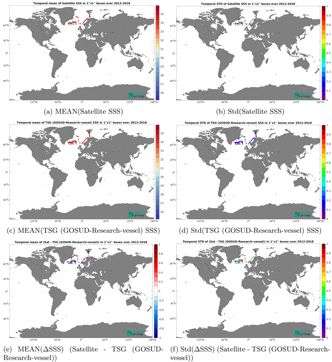
Figure 6: Temporal mean (left) and Std (right) of SSS from SMOS SSS L3 Arctic v1.1 - 7-Day running mean (CATDS-CEC-LOCEAN) (top), TSG (GOSUD-Research-vessel) (middle), and of \Delta SSS (Satellite - TSG (GOSUD-Research-vessel)). Only match-up pairs are used to generate these maps.
