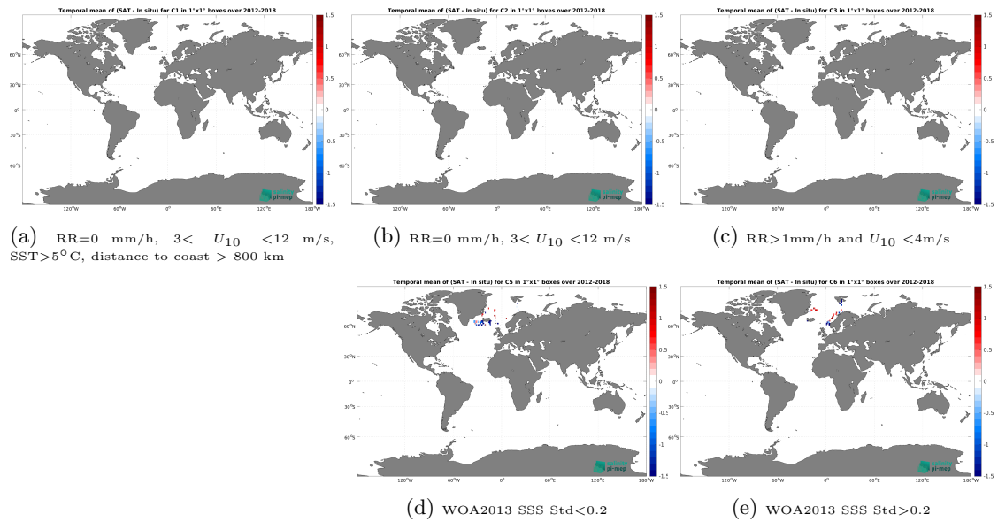
Figure 12: Temporal mean gridded over spatial boxes of size 1^{\circ}\times 1^{\circ} of \Delta SSS (SMOS SSS L3 Arctic v1.1 - 7-Day running mean (CATDS-CEC-LOCEAN) - TSG (GOSUD-Research-vessel)) for 5 different subdatasets corresponding to:RR=0 mm/h, 3 < U_{10} < 12 m/s, SST >5^{\circ}\text{C} , distance to coast > 800 km (a), RR=0 mm/h, 3 < U_{10} < 12 m/s (b), RR >1 mm/h and U_{10} < 4 m/s (c), WOA2013 SSS Std <0.2 (d), WOA2013 SSS Std >0.2 (e).
