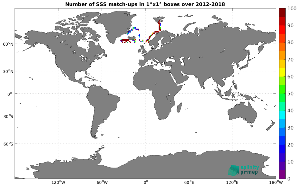
Figure 4: Number of SSS match-ups between TSG (GOSUD-Research-vessel) SSS and the SMOS SSS L3 Arctic v1.1 - 7-Day running mean (CATDS-CEC-LOCEAN) SSS product for the Global Ocean Pi-MEP region over 1^\circ \times 1^\circ boxes and for the full satellite product period.
