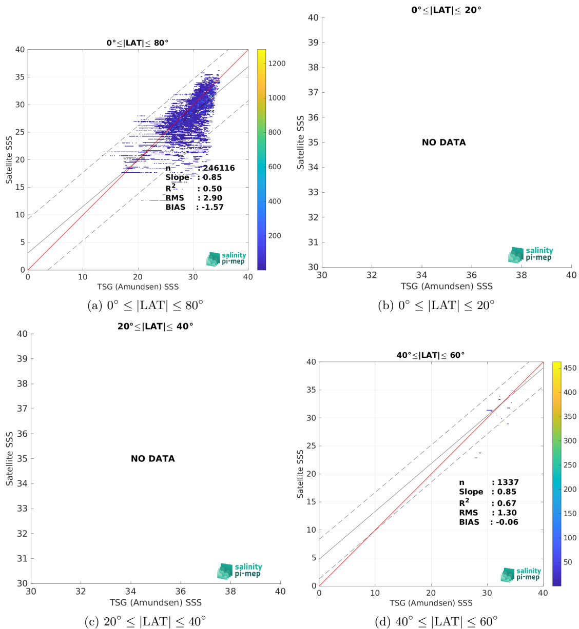
Figure 9: Contour maps of the concentration of SMOS SSS L3 Arctic v1.1 - 7-Day running mean (CATDS-CEC-LOCEAN) SSS (y-axis) versus TSG (Amundsen) SSS (x-axis) at match-up pairs for different latitude bands. For each plot, the red line shows x=y . The black thin and dashed lines indicate a linear fit through the data cloud and the \pm 95\% confidence levels, respectively. The number match-up pairs n , the slope and R^2 coefficient of the linear fit, the root mean square (RMS) and the mean bias between satellite and in situ data are indicated for each latitude band in each plots.
