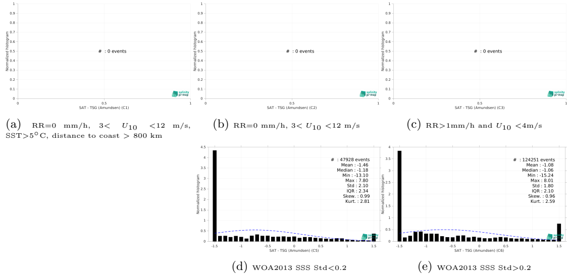
Figure 13: Normalized histogram of \Delta SSS (SMOS SSS L3 Arctic v1.1 - 7-Day runing mean (CATDS-CEC-LOCEAN) - TSG (Amundsen)) for 5 different subdatasets corresponding to: RR=0 mm/h, 3 < U_{10} < 12 m/s, SST>5°C, distance to coast > 800 km (a), RR=0 mm/h, 3 < U_{10} < 12 m/s (b), RR>1mm/h and U_{10} < 4 m/s (c), WOA2013 SSS Std<0.2 (d), WOA2013 SSS Std>0.2 (e).
