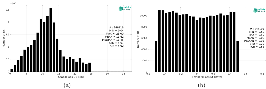
Figure 5: Histograms of the spatial (a) and temporal (b) lags between the location/time of the TSG (Amundsen) measurement and the date of the corresponding SMOS SSS L3 Arctic v1.1 - 7-Day running mean (CATDS-CEC-LOCEAN) SSS pixel.
