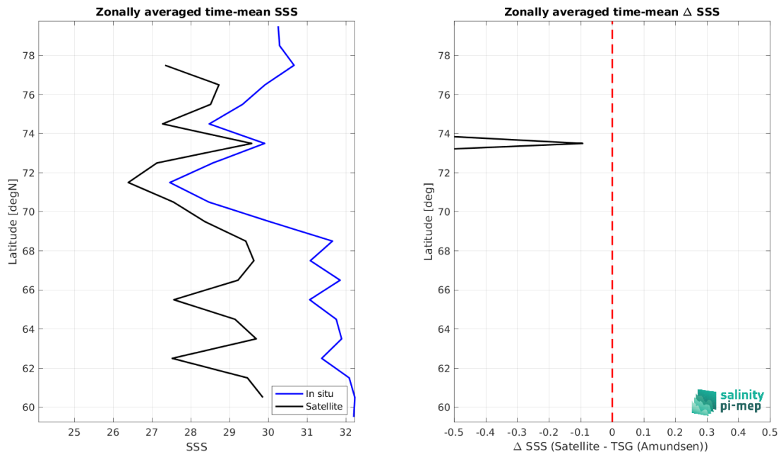
Figure 8: Left panel: Zonal mean SSS from SMOS SSS L3 Arctic v1.1 - 7-Day running mean (CATDS-CEC-LOCEAN) satellite product (black) and from TSG (Amundsen) (blue). Right panel: Zonal mean of \Delta SSS (Satellite - TSG (Amundsen)) for all the collected Pi-MEP match-up pairs estimated over the full satellite product period.
