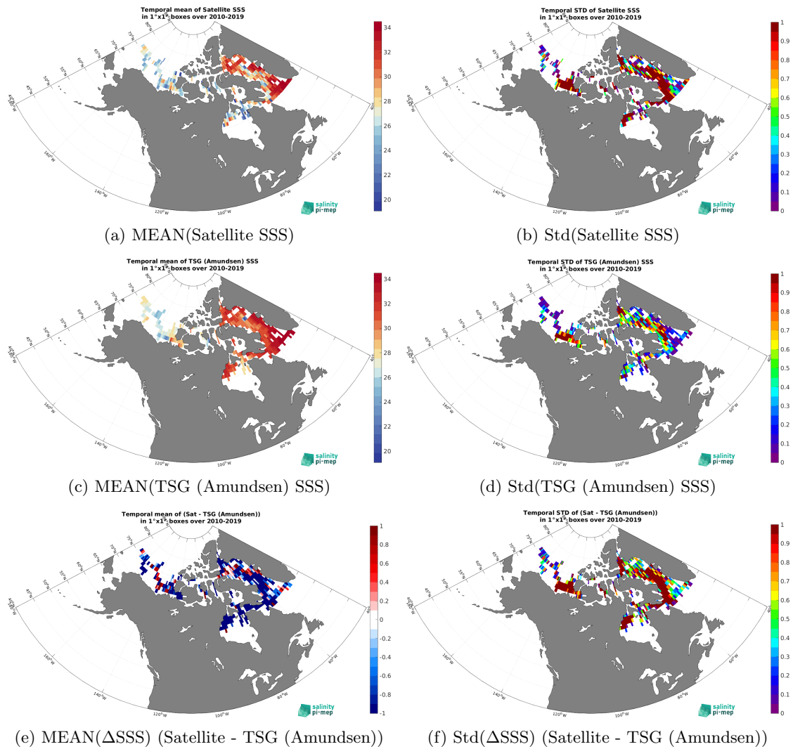
Figure 6: Temporal mean (left) and Std (right) of SSS from SMOS SSS L3 Arctic v1.1 - 7-Day running mean (CATDS-CEC-LOCEAN) (top), TSG (Amundsen) (middle), and of \Delta SSS (Satellite - TSG (Amundsen)). Only match-up pairs are used to generate these maps.
