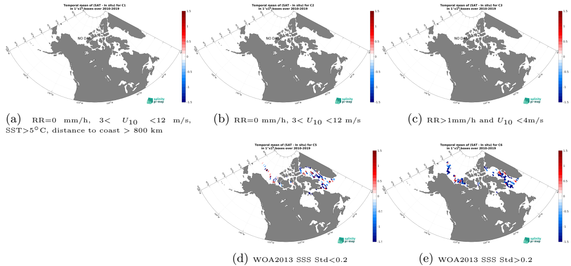
Figure 12: Temporal mean gridded over spatial boxes of size 1^{\circ}\times 1^{\circ} of \Delta\text{SSS} (SMOS SSS L3 Arctic v1.1 - 7-Day running mean (CATDS-CEC-LOCEAN) - TSG (Amundsen)) for 5 different subdatasets corresponding to:RR=0 mm/h, 3 < U_{10} < 12 m/s, SST >5^{\circ}\text{C} , distance to coast > 800 km (a), RR=0 mm/h, 3 < U_{10} < 12 m/s (b), RR >1 mm/h and U_{10} < 4 m/s (c), WOA2013 SSS Std <0.2 (d), WOA2013 SSS Std >0.2 (e).
